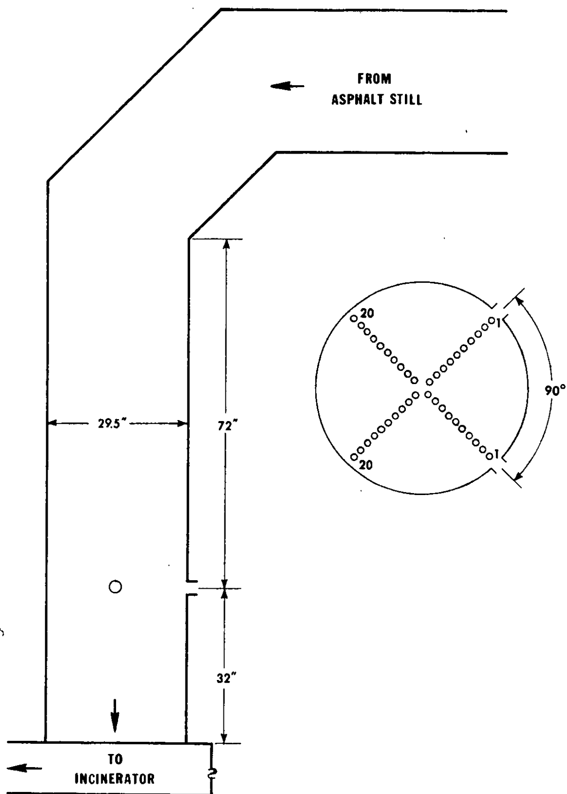
Figure B-5. Saturator inlet - Plant B.
