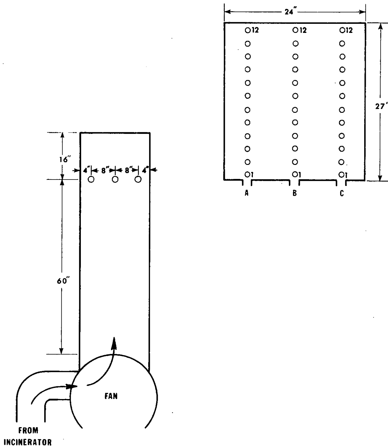
Figure B-6. Saturator outlet - Plant B.
