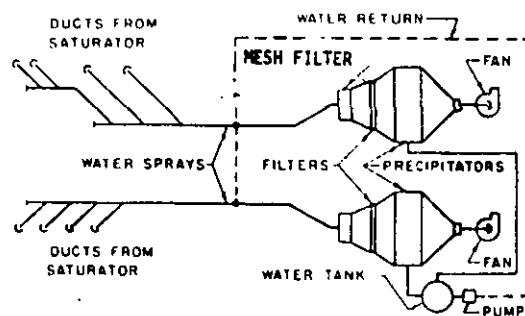
Figure 5.1 Flow diagram for low-voltage electrostatic precipitators. 5.1
