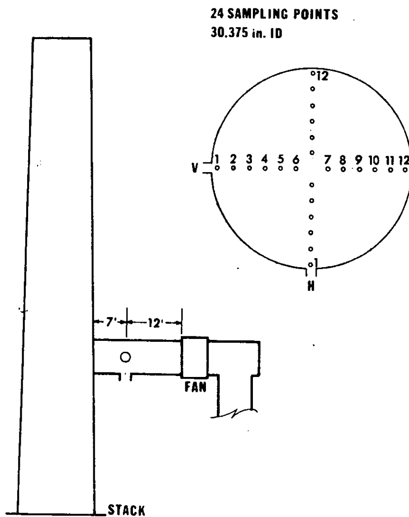
Figure B-9. Asphalt blowing outlet - Plant C.
