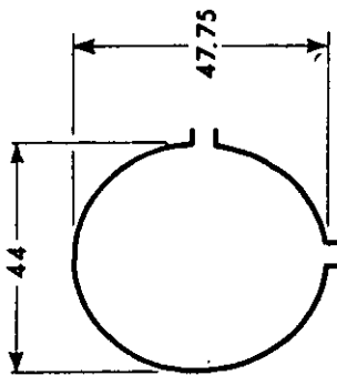
L-3 EXIT STACK
