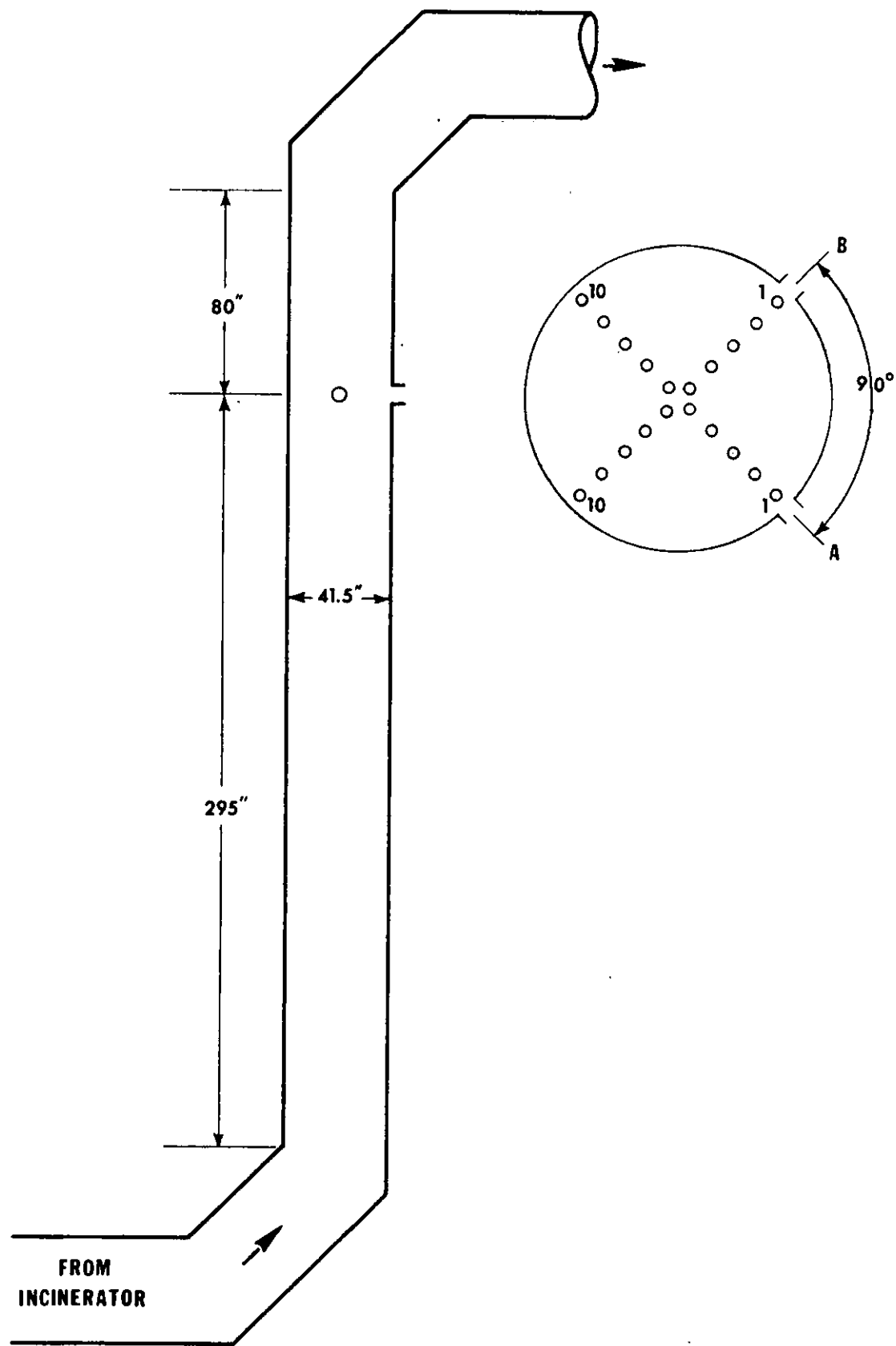
Figure B-4. Asphalt blowing outlet - Plant B.
