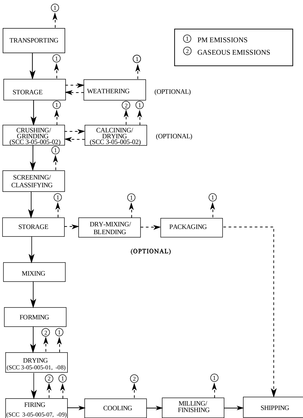
Figure 11.5-1. Refractory manufacturing process flow diagram. 1 (Source Classification Codes in parentheses.)
