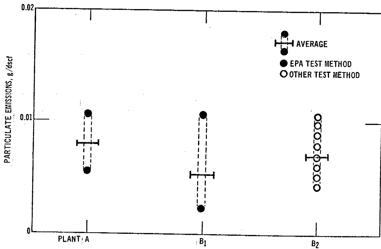
Figure 1. Particulate emissions from air table exhausts controlled by fabric filters.
