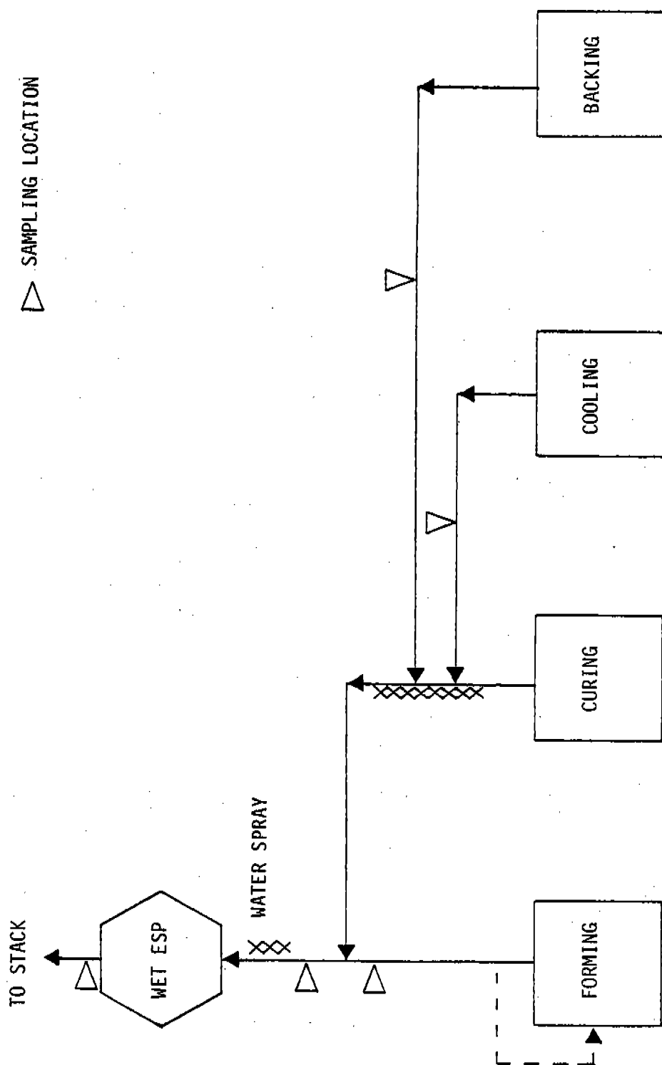
Figure C-5. Schematic drawing of sampling locations for Line E.
