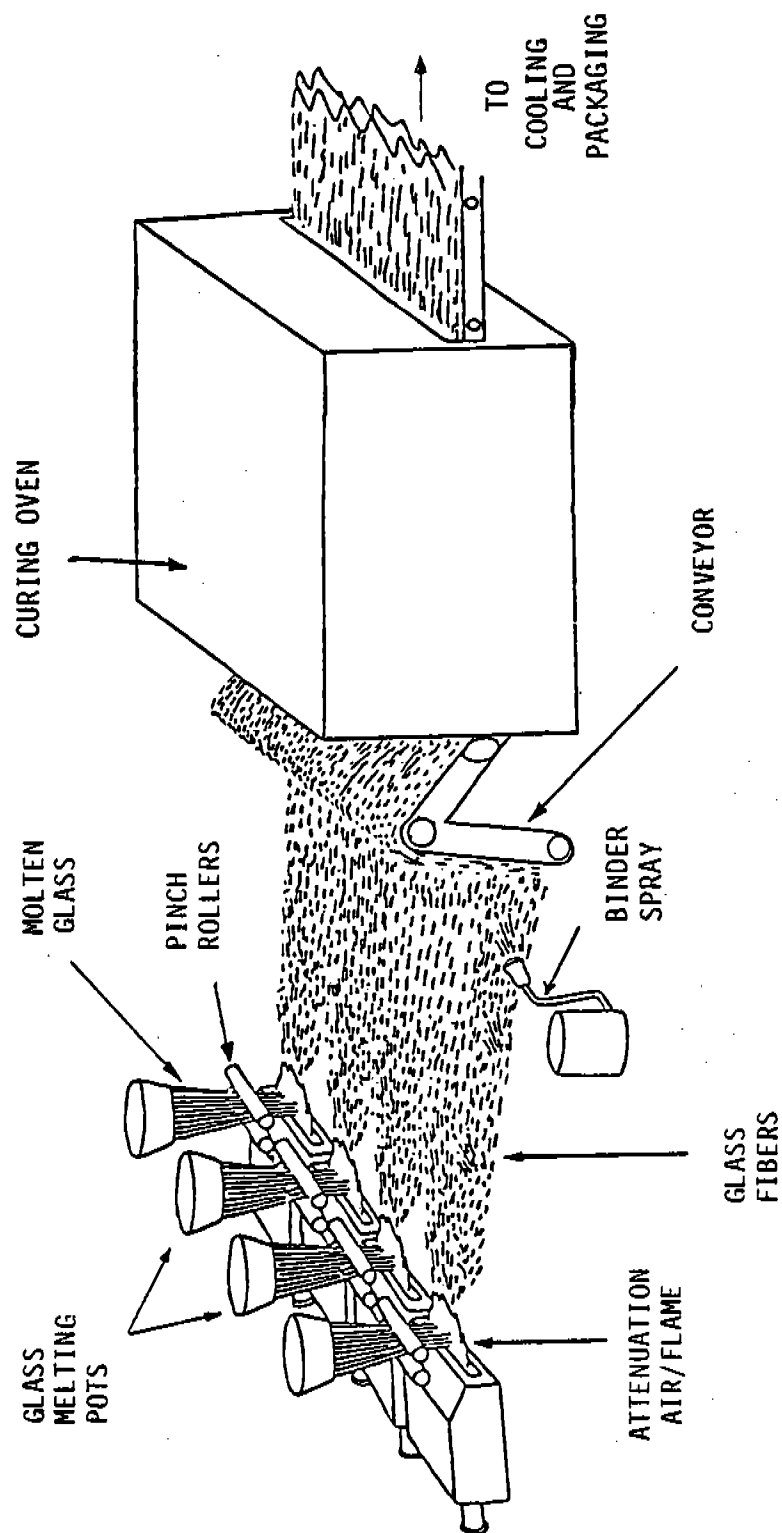
Figure 3-4. Flame attenuation process.
