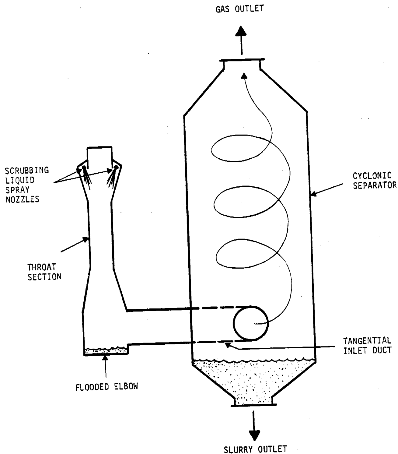
Figure 4-4. Cross-sectional side view of a typical venturi scrubber.
