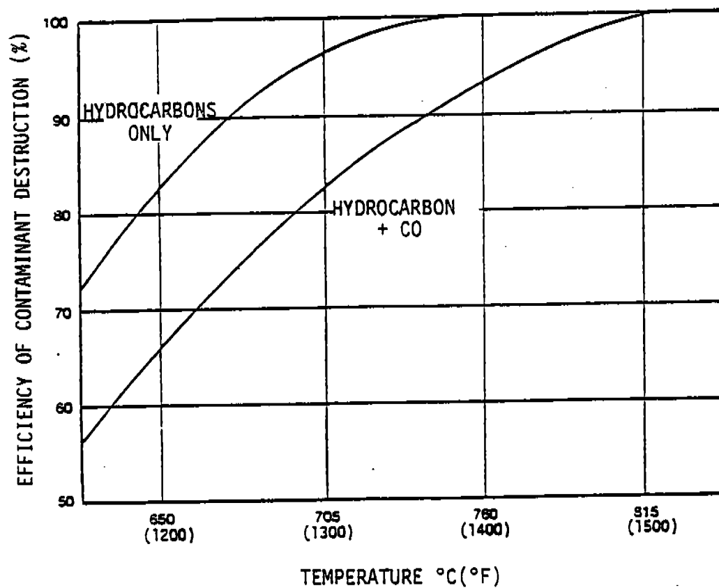
Figure 4-10. Typical effect of operating temperature on effectiveness of thermal incinerator for destruction of hydrocarbons and carbon monoxide. 54
