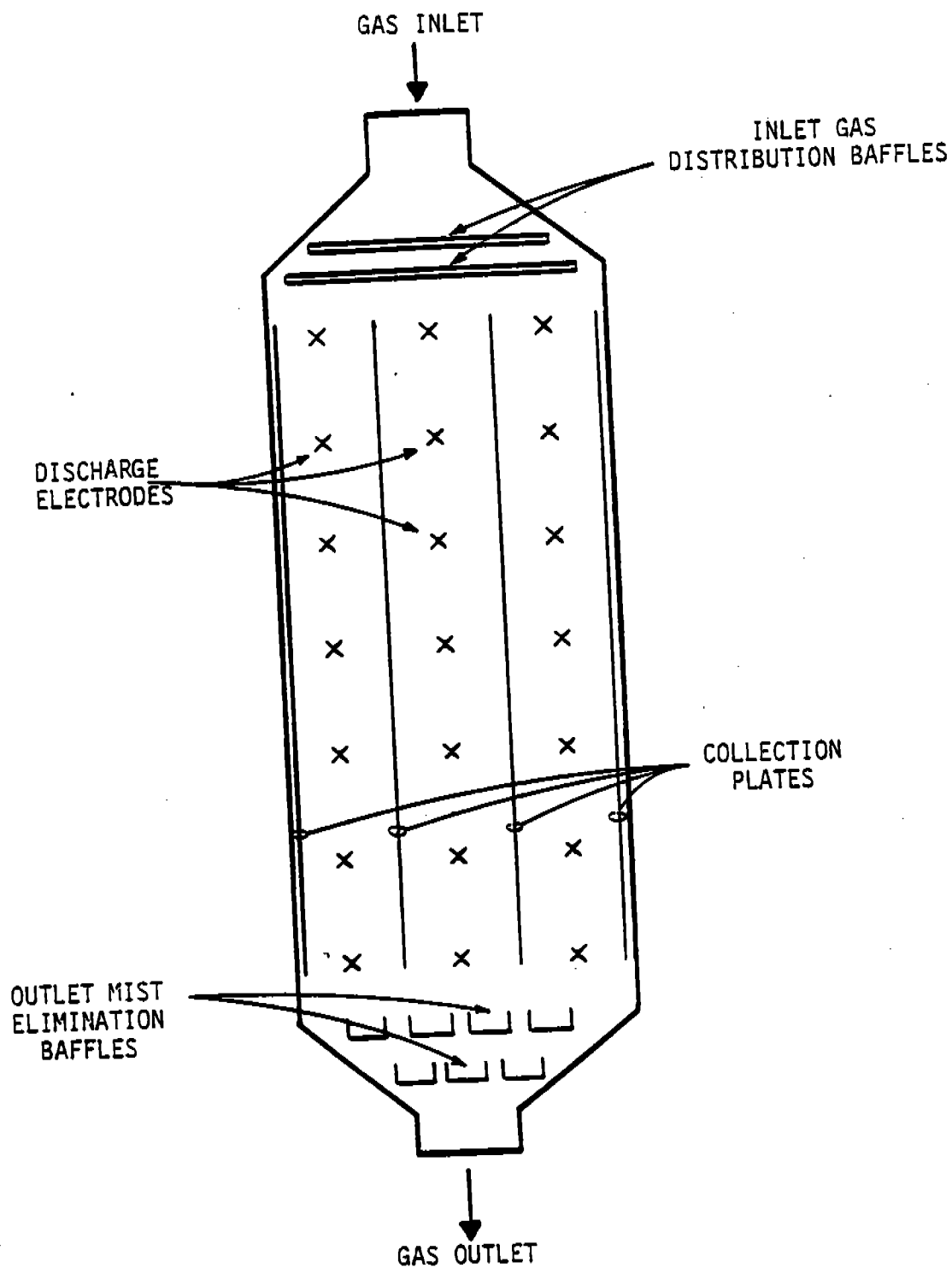
Figure 4-2. Cross-sectional top view of a typical wet ESP.
