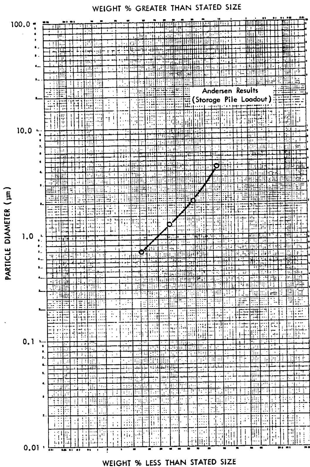
Figure 19. Particle size distribution--aggregate loadout emissions.
