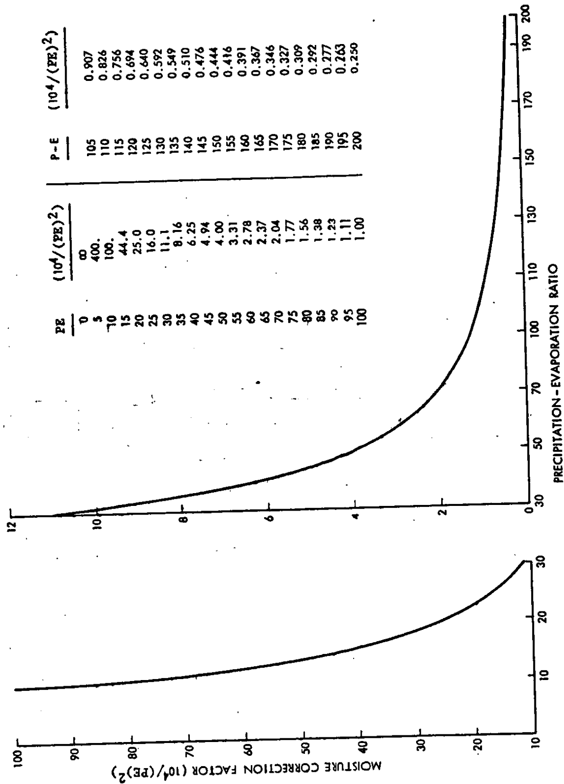
Figure 26. Moisture correction factors.
