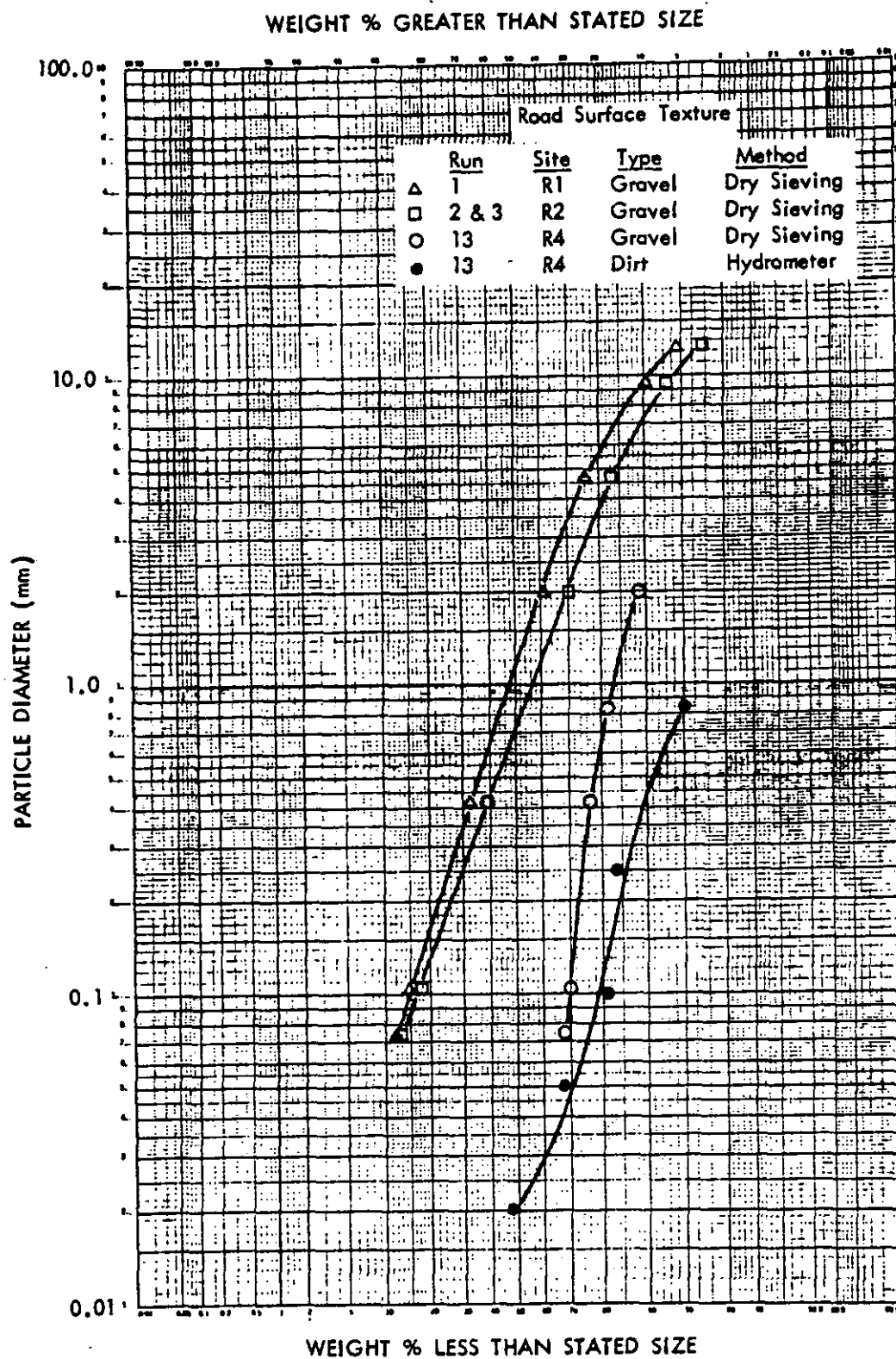
Figure 8. In-place road dust texture.
