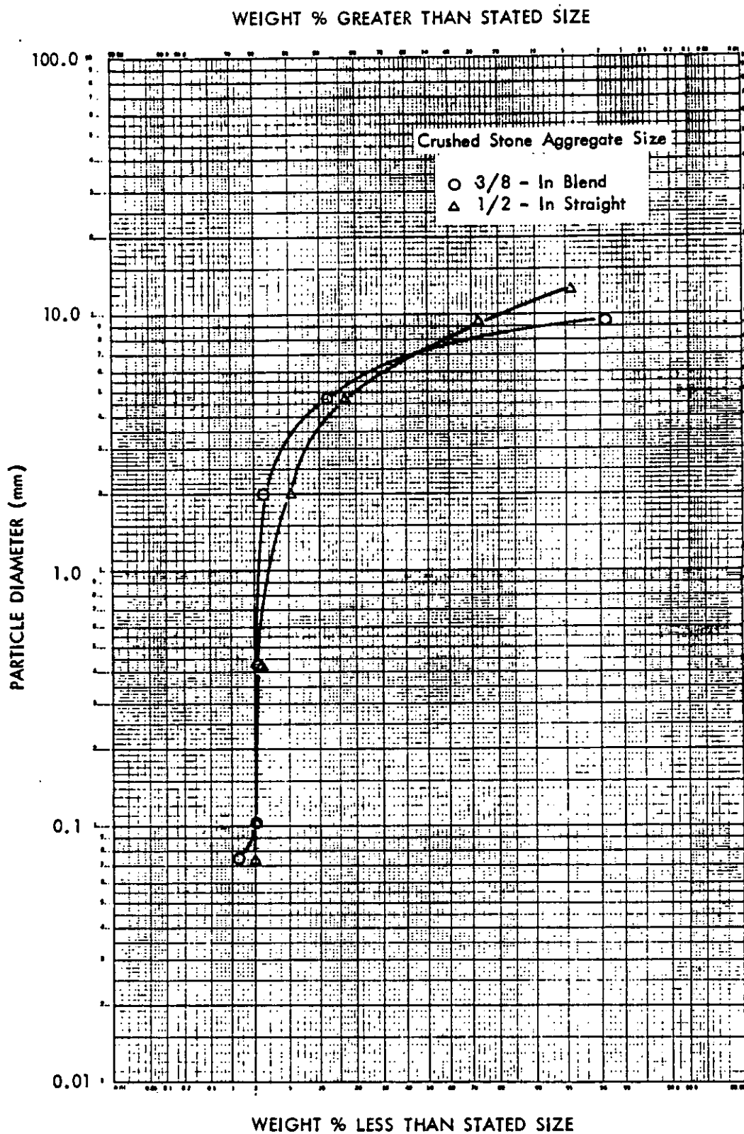
Figure 20. Aggregate size distribution--crushed stone.
