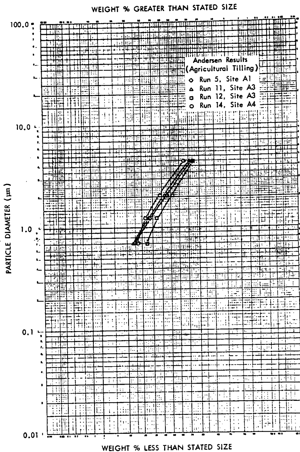
Figure 13. Particle size distributions--agricultural emissions.
