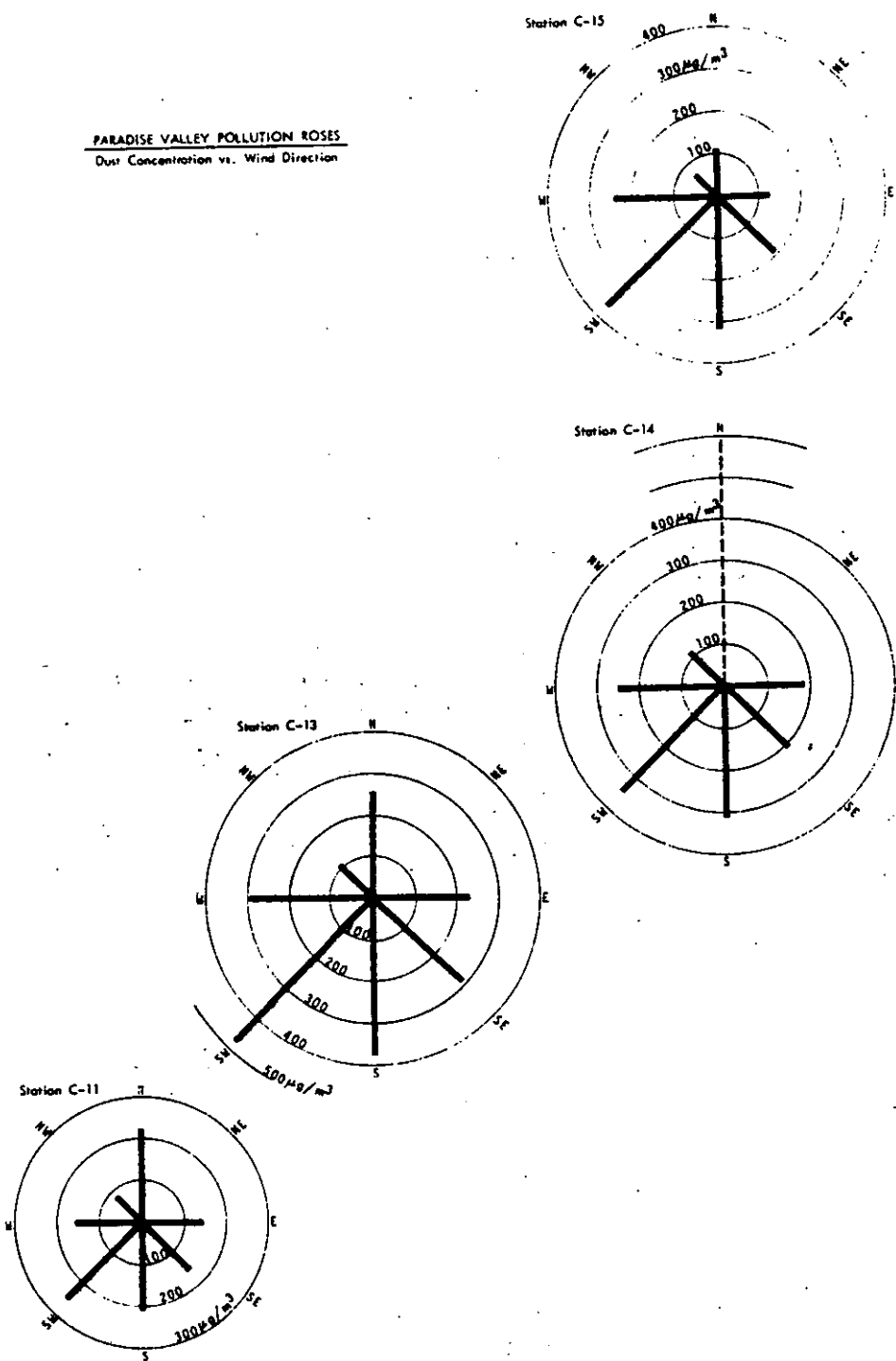
Figure 22. Pollution Roses - Paradise Valley Construction Site.
