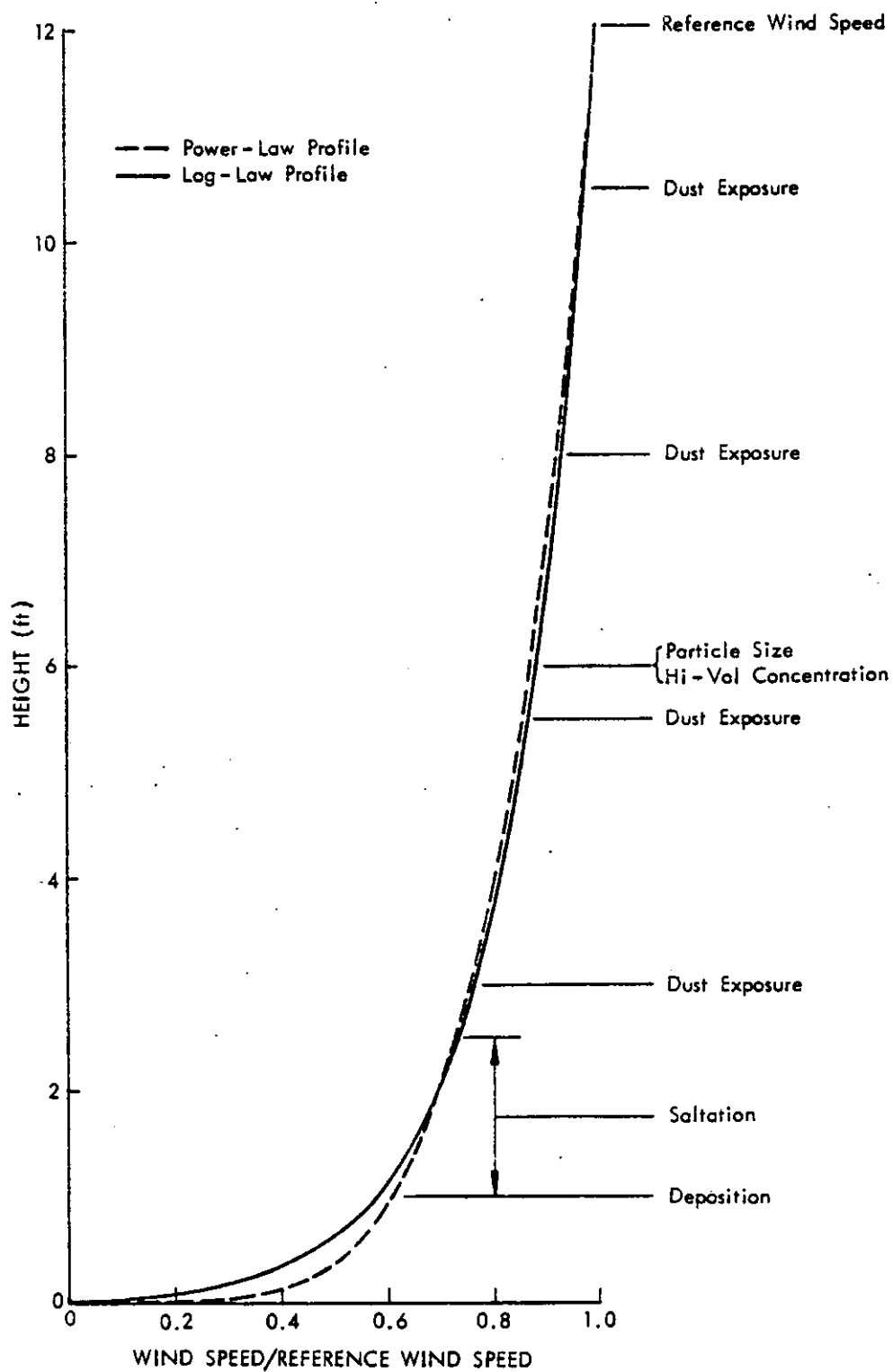
Figure 2. Comparison of wind speed profiles.
