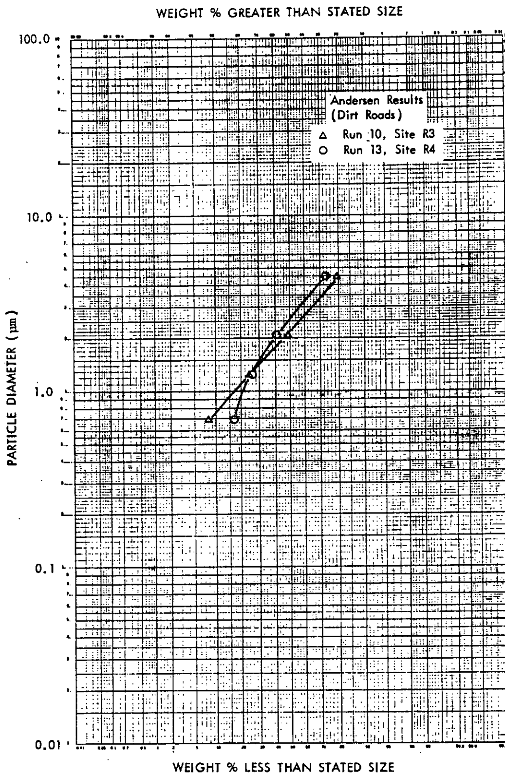
Figure 7. Particle size distributions--dirt road emissions.
