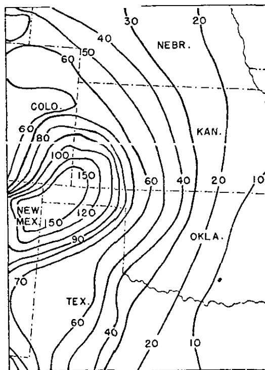
Fig. 5—Wind erosion climatic factor C' (per cent) for Kansas and parts of Nebraska, Colorado, Oklahoma, New Mexico, and Texas. Similar maps for other parts of the USA are available from the Erosion Research Laboratory at Manhattan, Kans.
