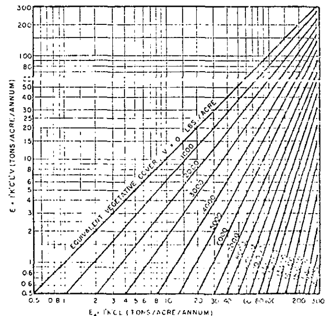
Fig. 10—Chart to determine soil loss E = I'K'C'LV from soil loss E_4 = I'K'C' and from the vegetative cover factor, V . The chart can be used in reverse to determine V needed to reduce soil loss to any degree.
