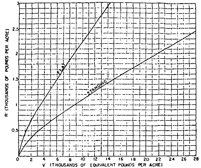
Fig. 7—Chart to determine V from R' or R' from V of standing and flat anchored small grain stubble with any row width up to 10 inches, including stover.
