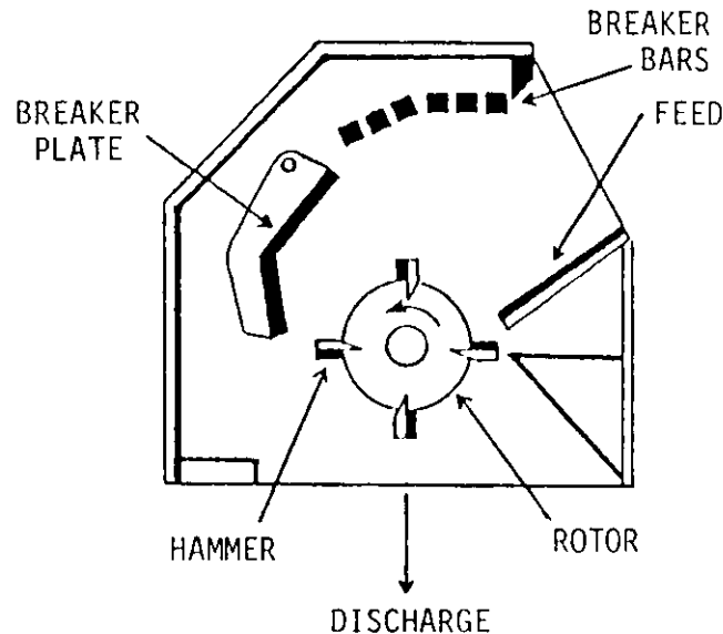
Figure 2.10 Impact Crusher
