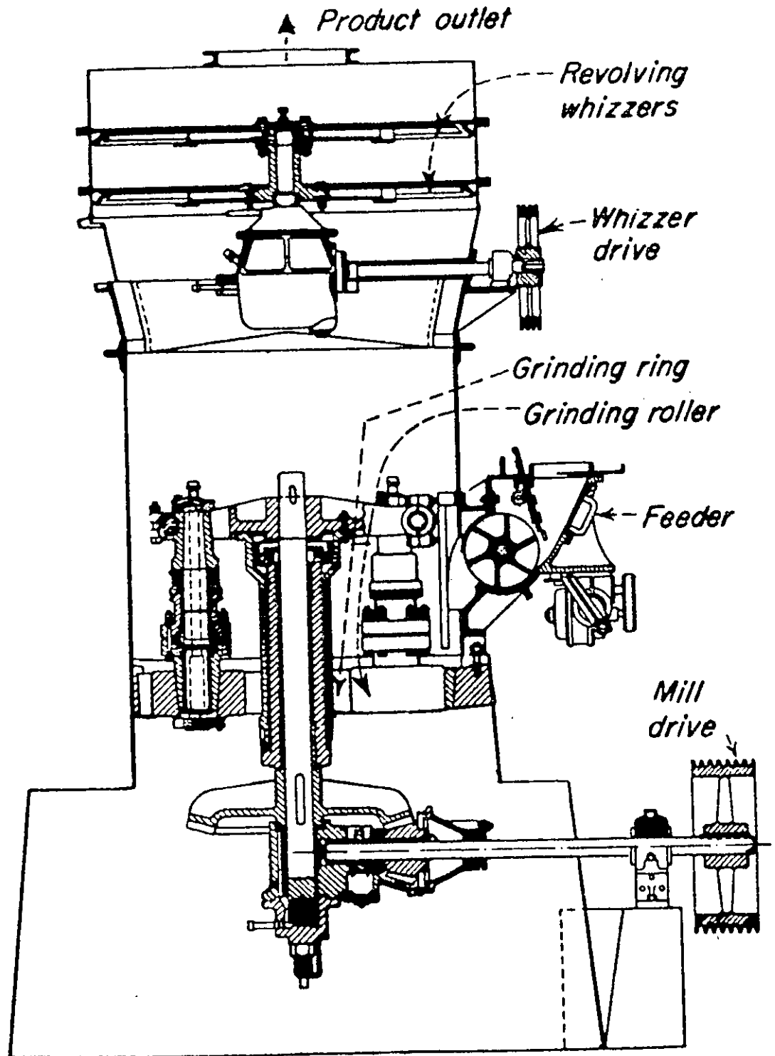
Figure 2.15 Roller Mill
