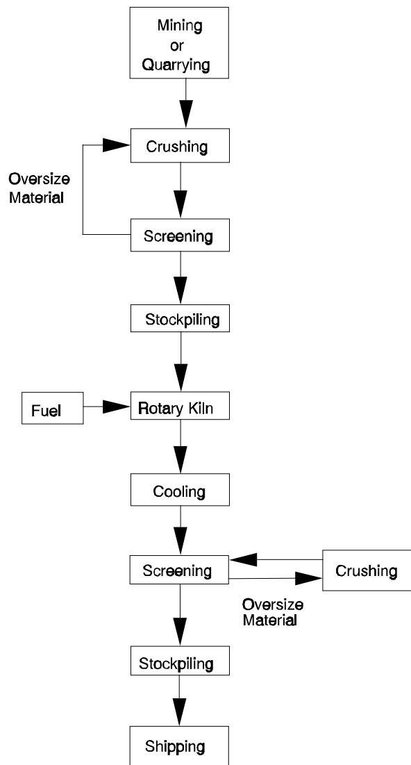
Figure 11.20-1. Process flow diagram for lightweight aggregate manufacturing.
