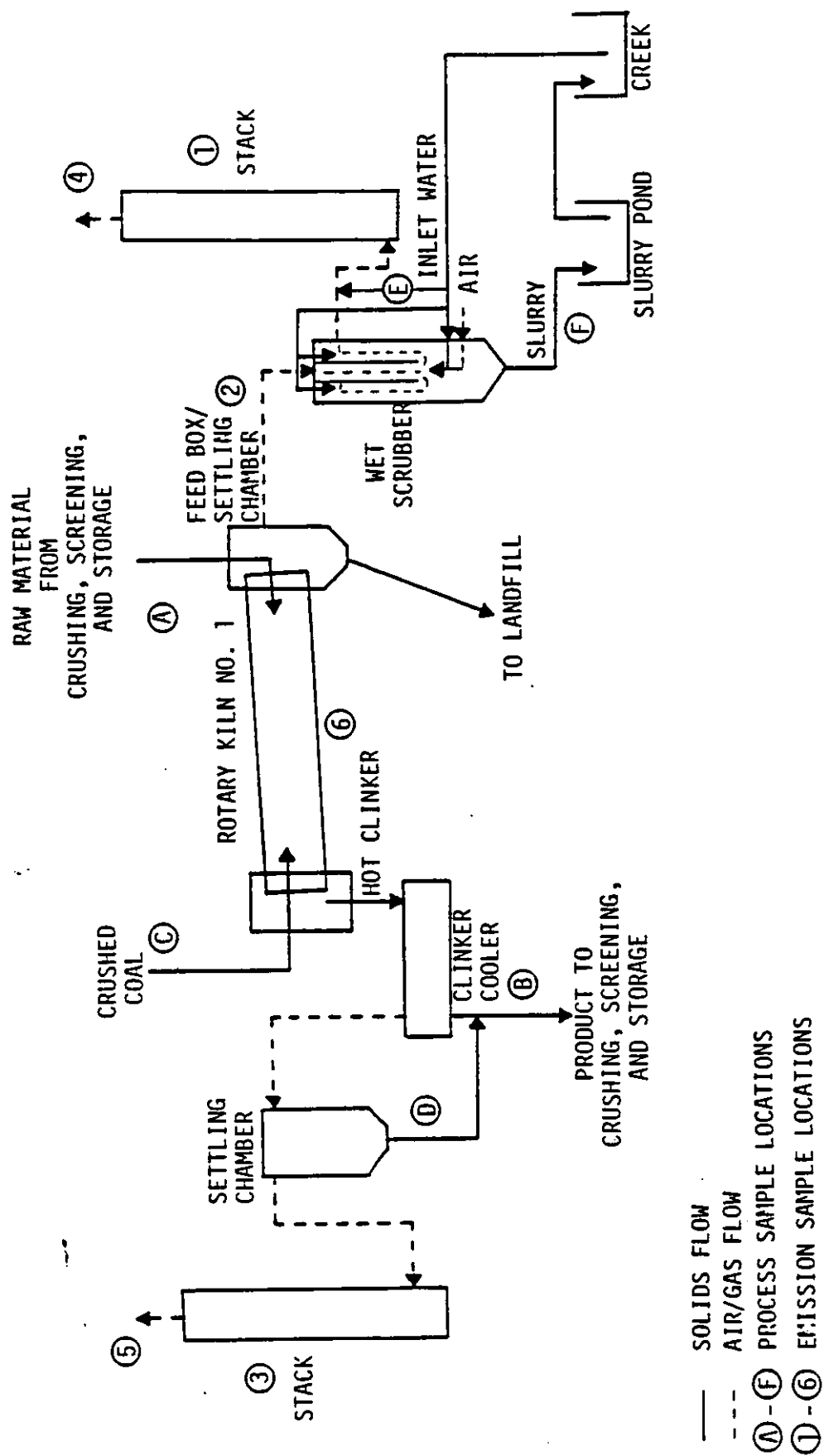
Figure 2-1. Simplified process flow diagram for the lightweight aggregate plant at Galite Corporation, Rockmart, Georgia.
