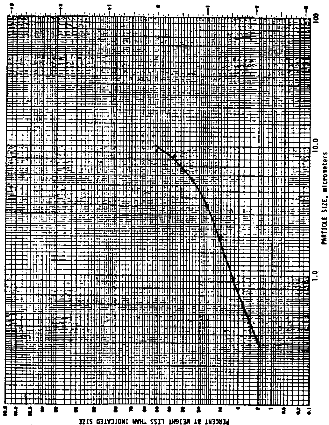
Figure 3-12. Particle size distribution for Run No. CCPS-4.
