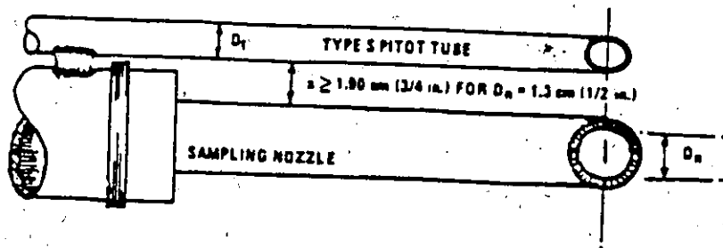
A. BOTTOM VIEW: SHOWING MINIMUM PITOT-NOZZLE SEPARATION.
