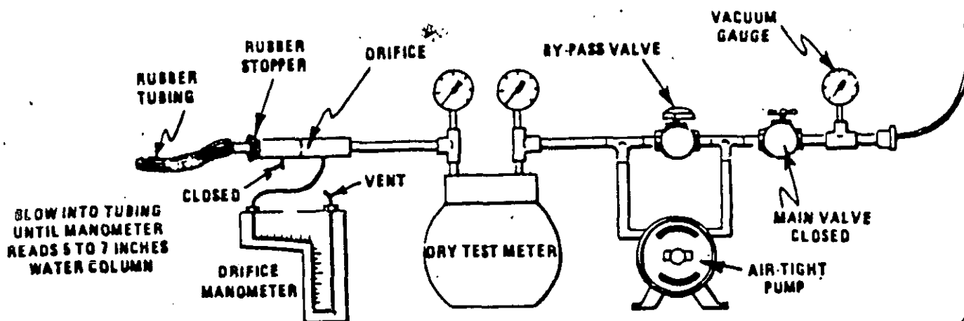
Figure 17-5. Leak check of meter box.
