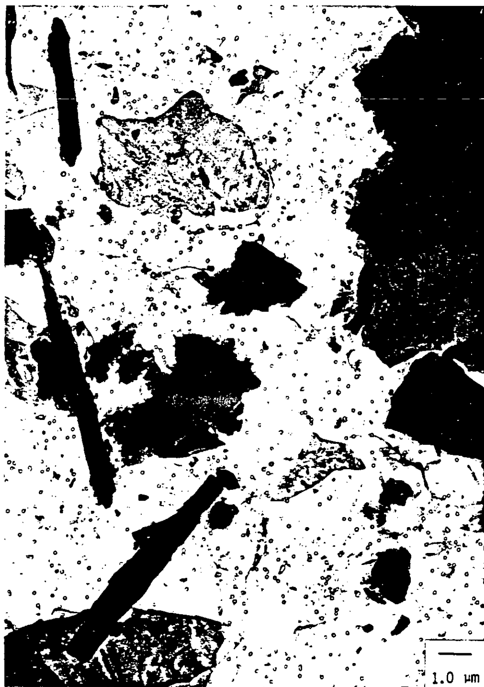
Transmission electron micrograph showing typical particulate matter found in water suspension after laboratory exfoliation of Sample 264-O, Grace, Libby, Montana, Grade 5 (composite).
