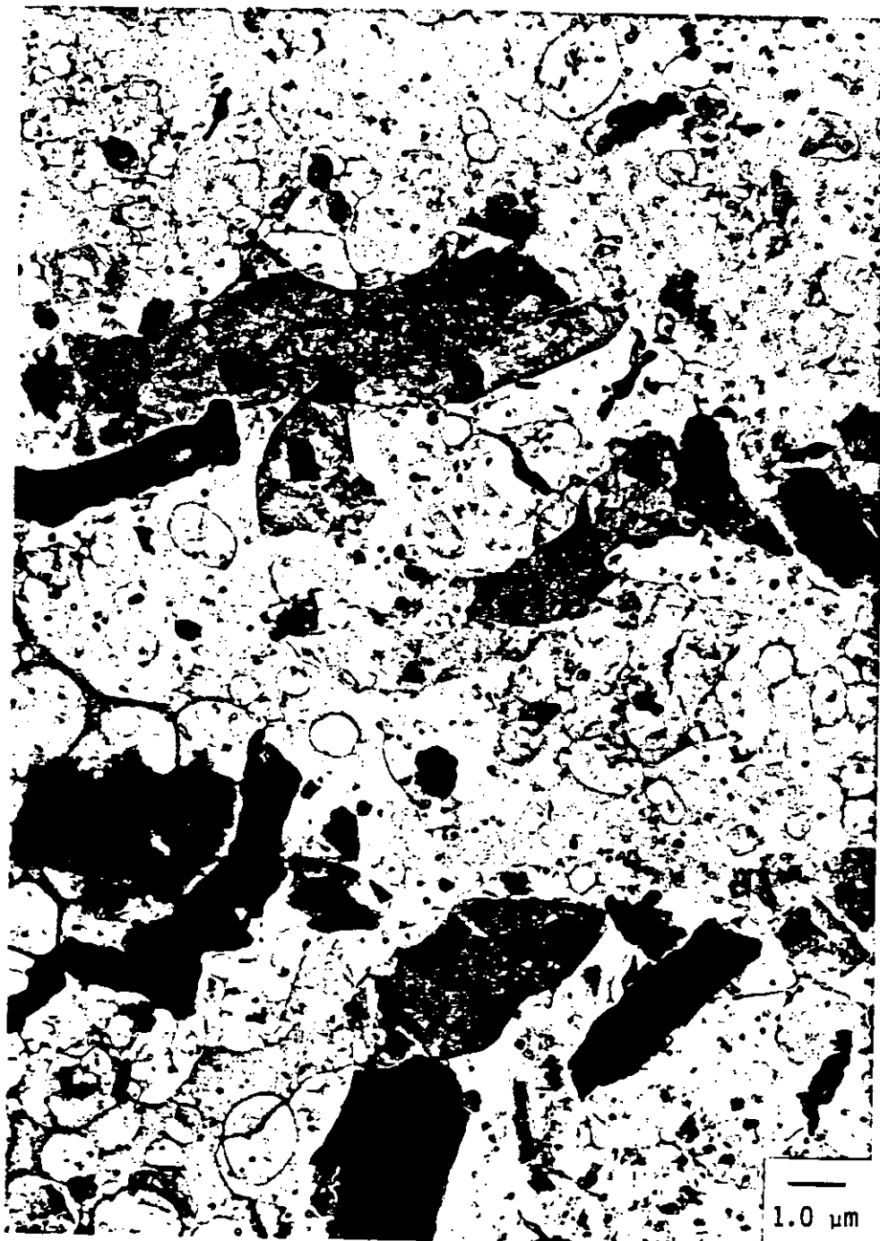
Transmission electron micrograph showing typical particulate matter found in water suspension after laboratory exfoliation of Sample 573-0, Patterson, Enoree, South Carolina, Ungraded, Dried Ore (composite).
