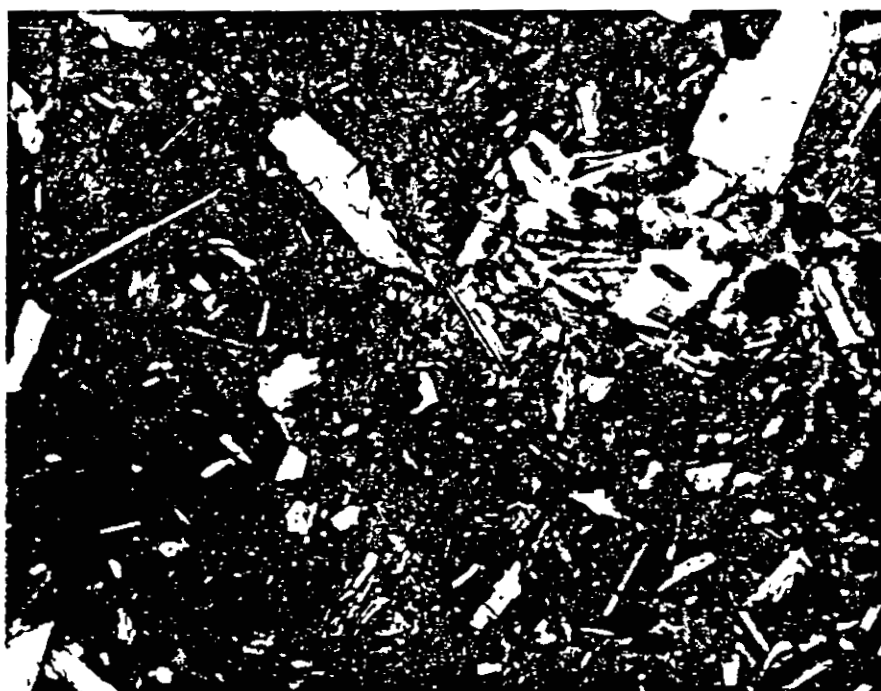
430-I-2.76 sink (after grinding); 208X. Most of the prismatic to near fibrous amphibole separated into this density fraction because it was so intimately intergrown with vermiculite and talc.
