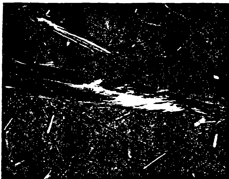
259-I-TBS-Fibers (ground); 208X. Large bundle in the center is unquestionably fibrous tremolite-actinolite. Note the (white) interference colors of fibers growing at angles to the main fiber bundle which has been rotated to an extinction position (and is therefore gray).
