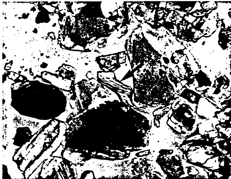
436-I; 82X. The amphiboles are mostly chunky and prismatic in this sample. Arrow points to tremolite composed of rather thick, lamellated prisms.
