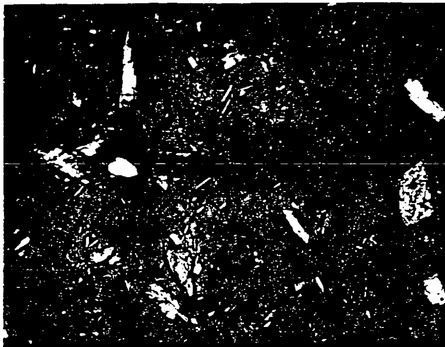
436-I-TBS-milky green (ground); 208X. Mineral grains composed of this tremolite-hornblend mixture were irregular in shape and rough. Appearances of crushed fragments indicated that the grains were composed of agglomerated smaller crystals which themselves were irregularly grown.
