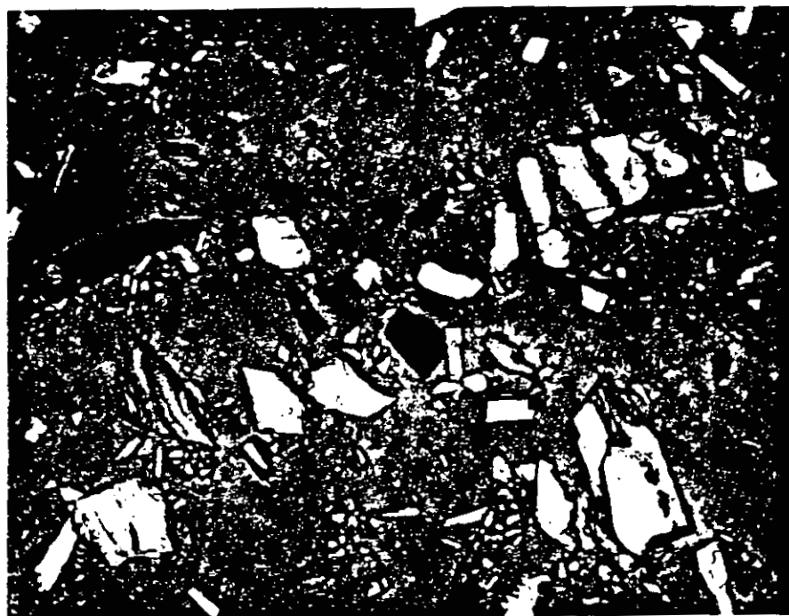
276-I-TBS-dark green glassy (ground); 208X. The pyroxene, diopside, exhibits some conchoidal as well as prismatic fracture patterns.
