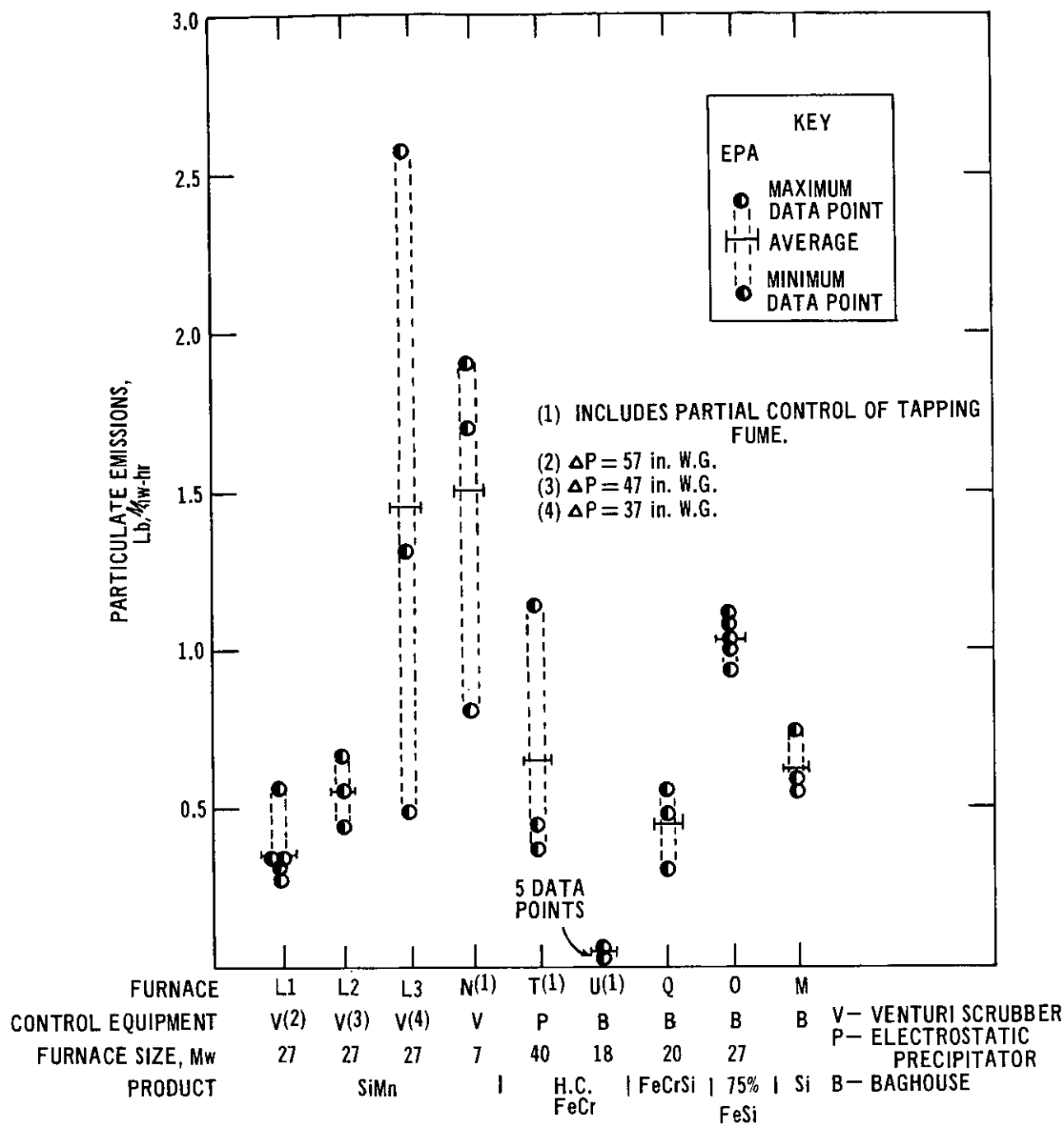
Figure VI-6. Particulate emissions from open electric submerged-arc furnaces producing ferroalloys.
