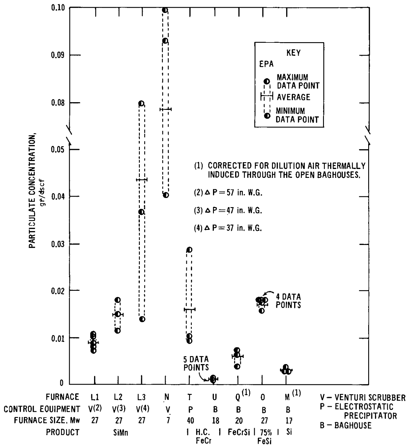
Figure VI-5. Particulate concentrations in control system exhaust from open electric submerged-arc furnaces producing ferroalloys.
