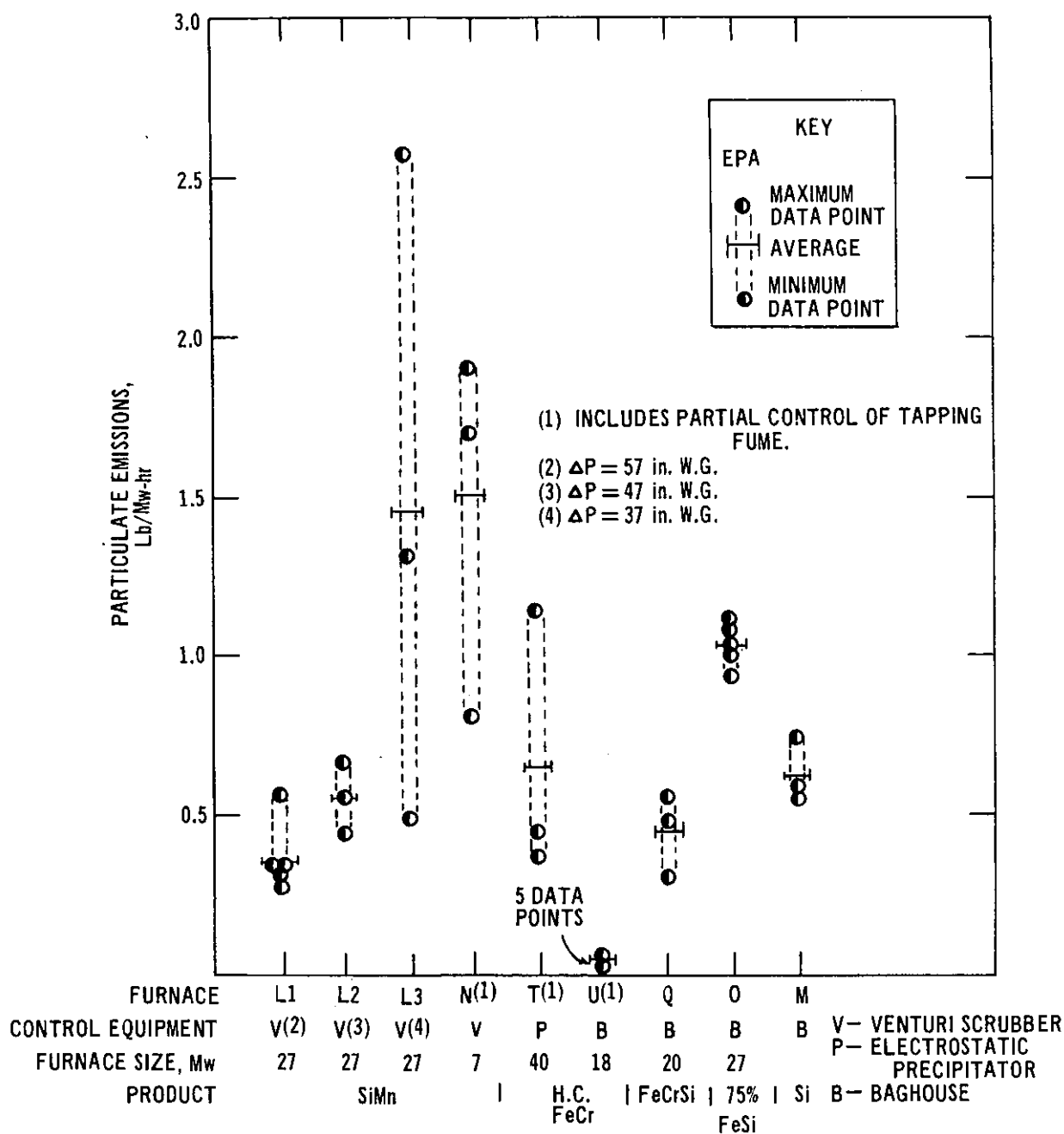
Figure 6. Particulate emissions from open electric submerged-arc furnaces producing ferroalloys.
