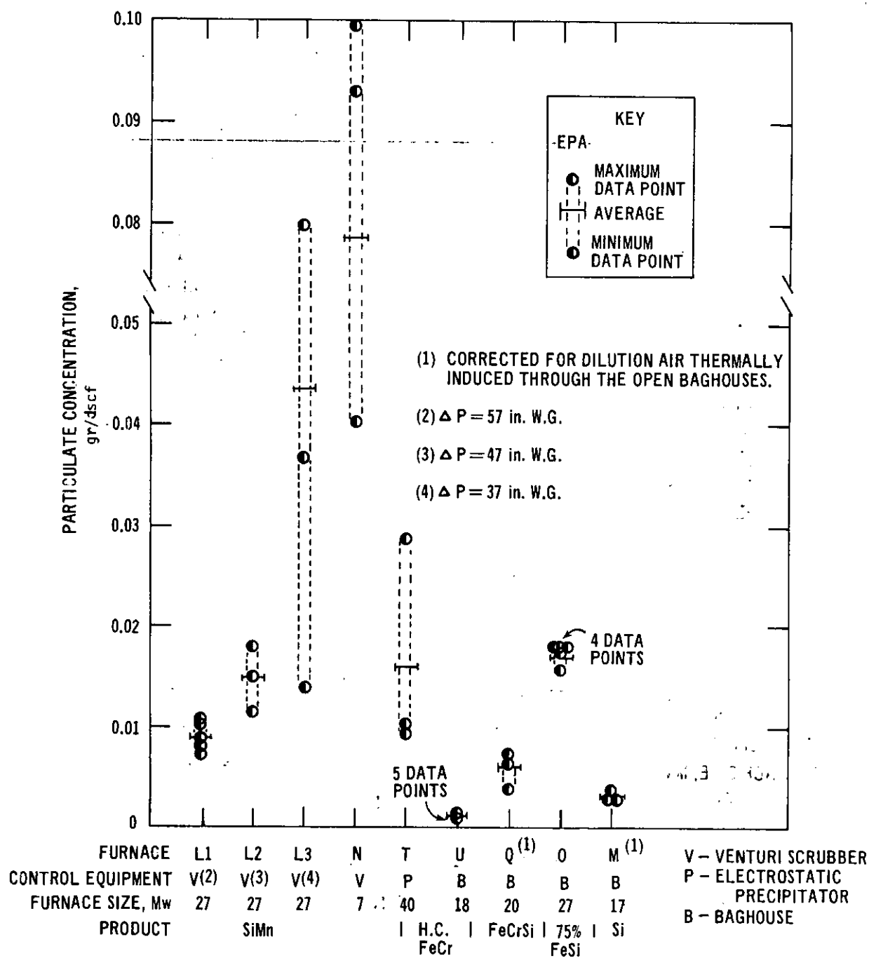
Figure 5. Particulate concentrations in control system exhaust from open electric submerged-arc furnaces producing ferroalloys.
