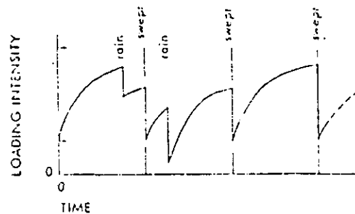
Accumulation of Contaminants - Typical Case (natural buildup with periodic sweeping and intermittent rainfall)
