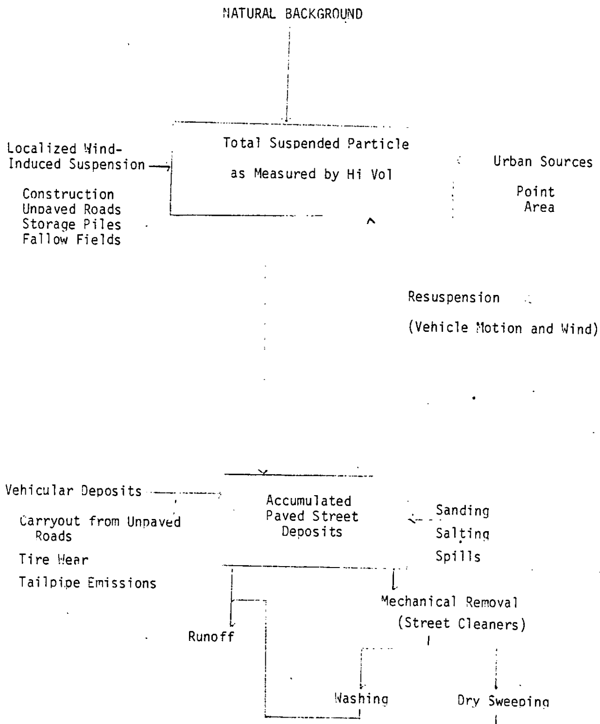
Figure 3. Urban Resuspension
