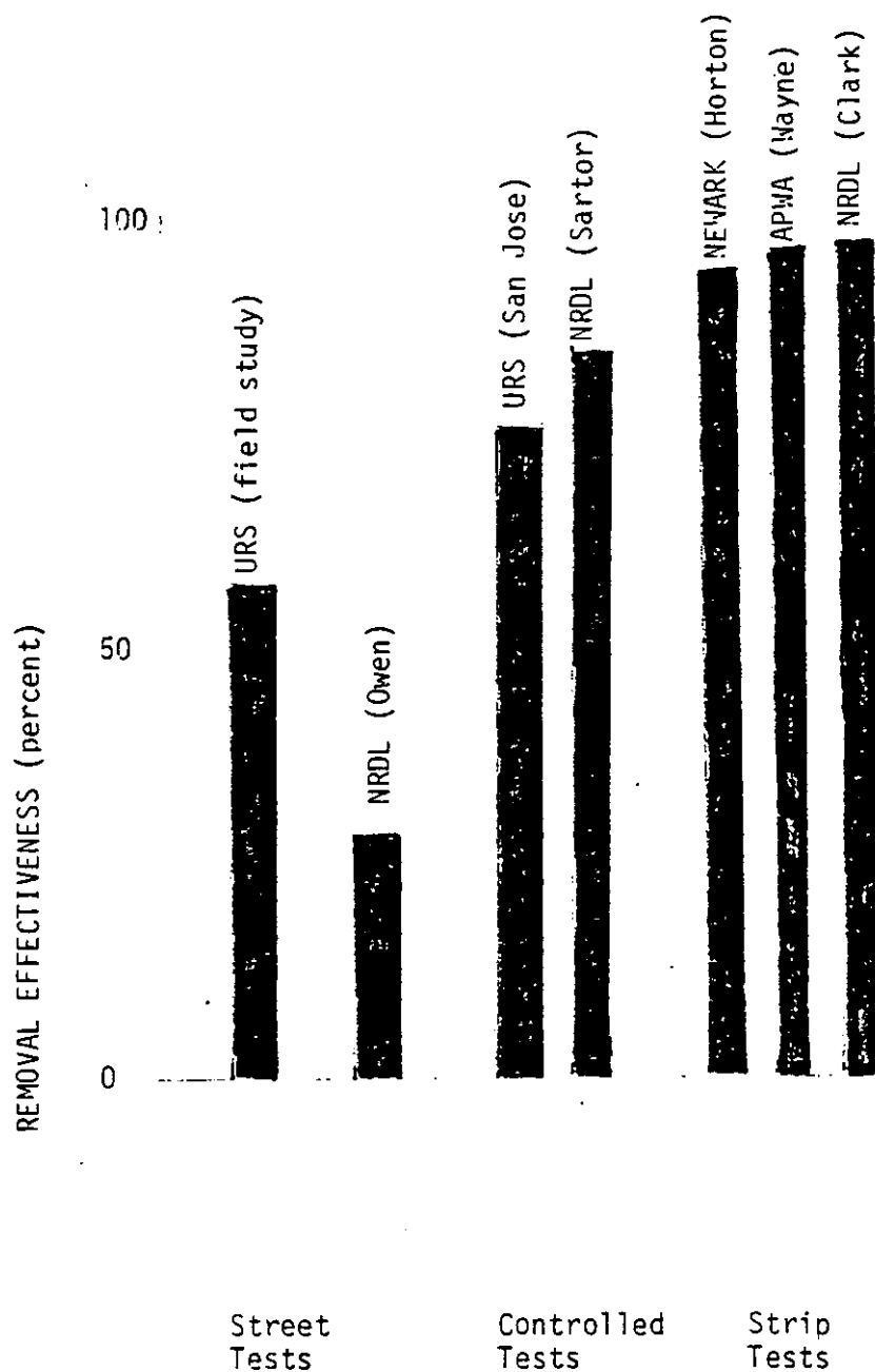
FIG. II. Comparison of Results from Sweeping Effectiveness Tests Conducted Under Various Conditions: For Dirt/Dust Fraction
