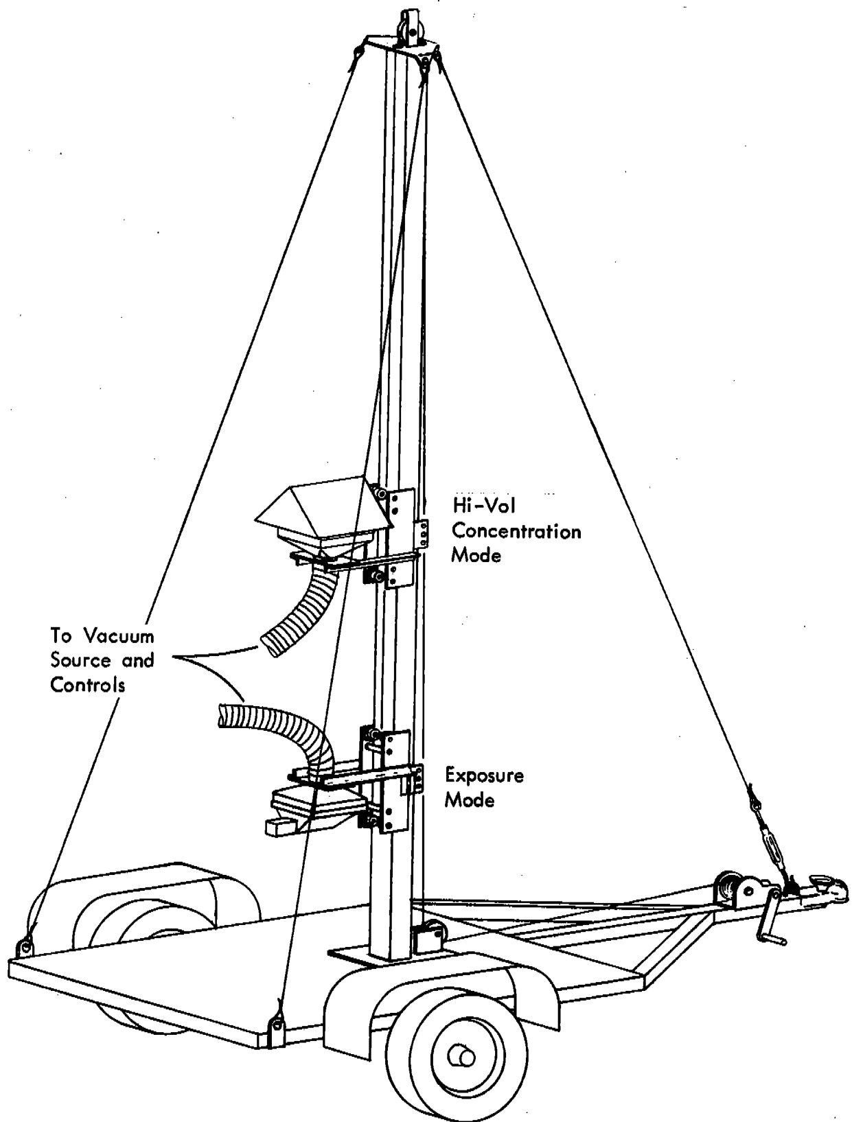
Figure 2. MRI Exposure Profiler (with illustrations of sampling modes)
