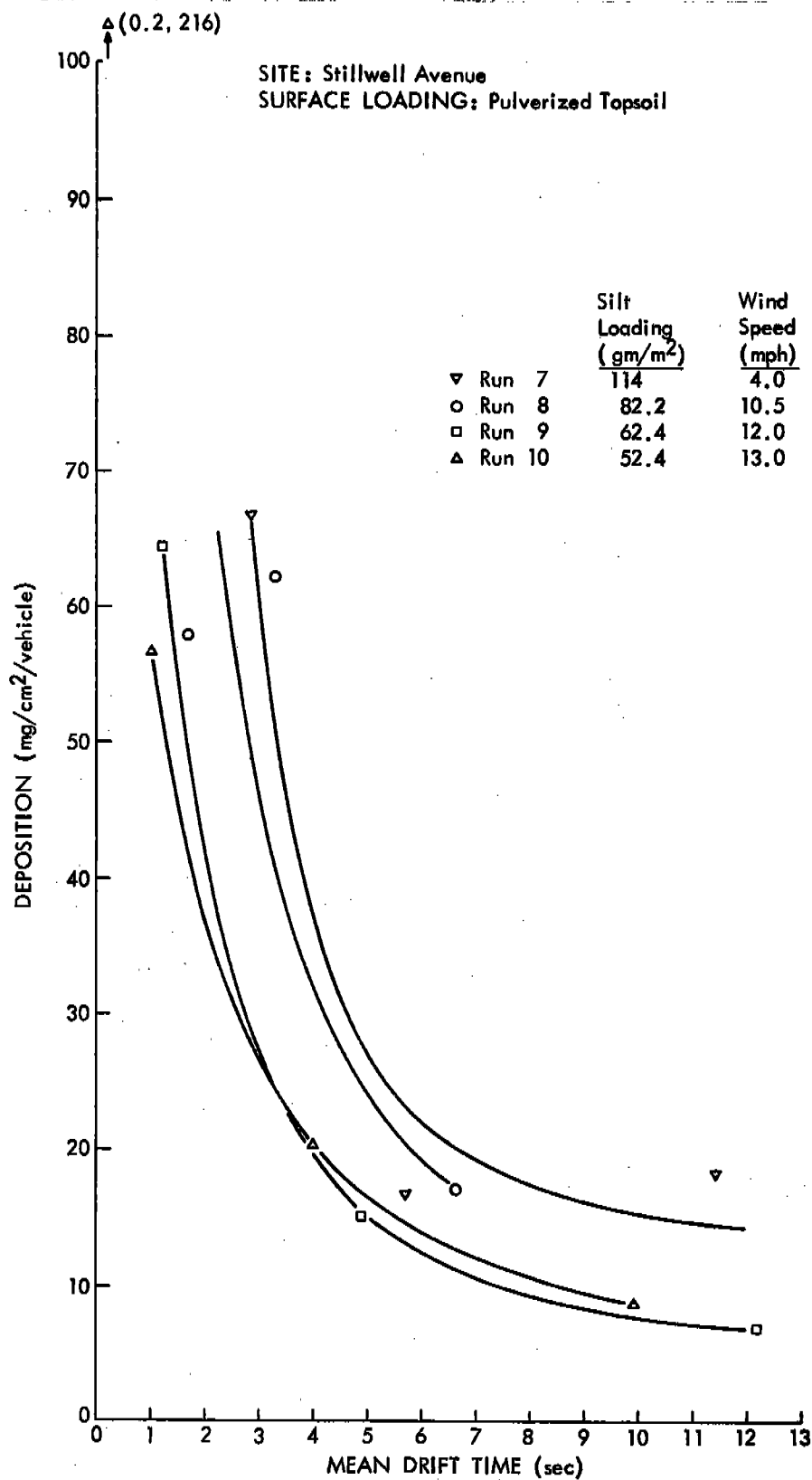
Figure 15. Downwind Distribution of Dust Deposition (Stillwell-Pulverized Topsoil)
