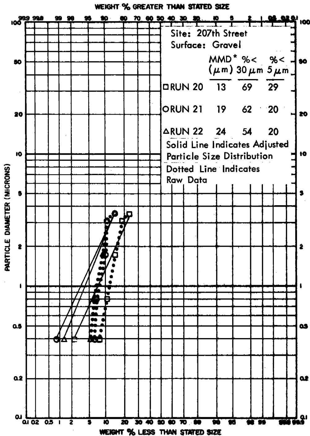
Figure A-5. Airborne Particle Size Distributions (207th Street-Gravel)
