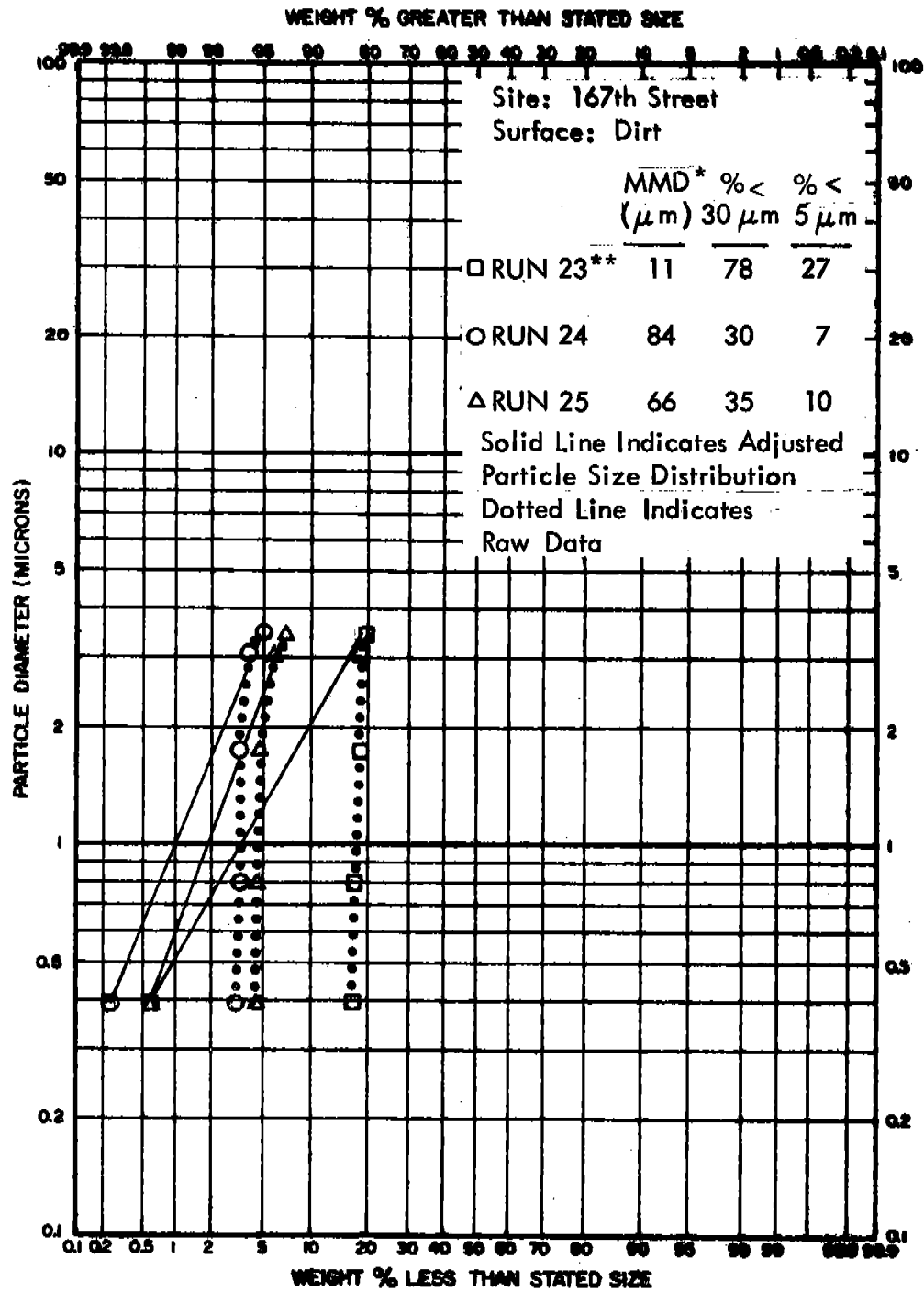
Figure A-6. Airborne Particle Size Distribution (167th Street-Dirt)
