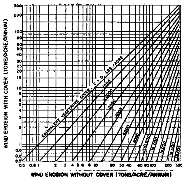
Figure B-2. Mitigative Effect of Vegetative Cover
