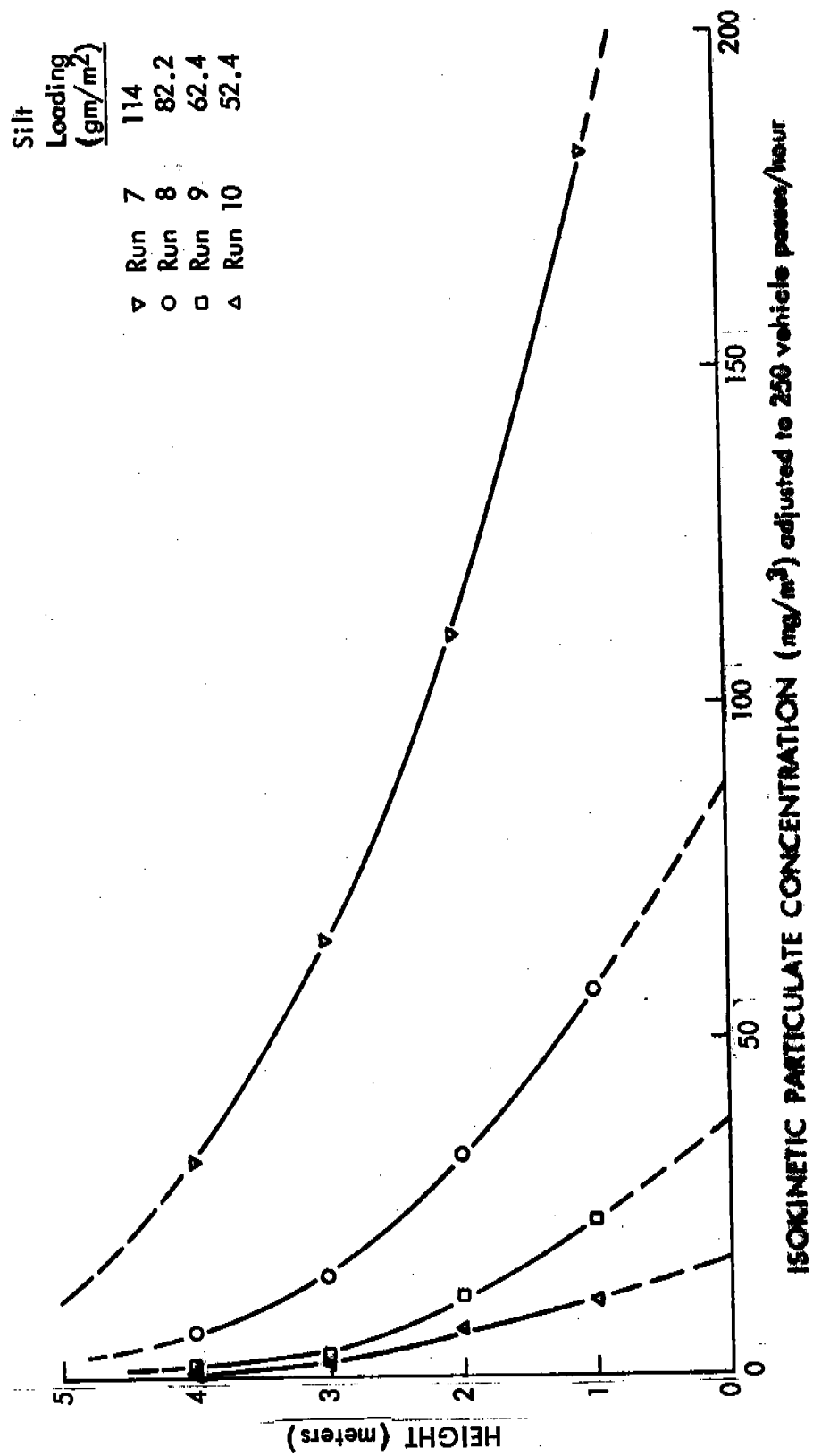
Figure 13. Vertical Profiles of Particulate Concentration (Stillwell-Pulverized Topsoil)
