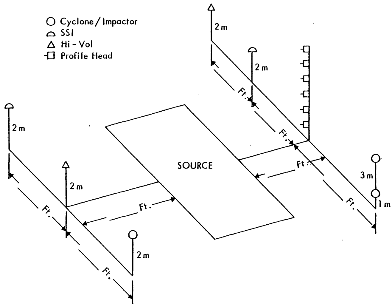
Figure 3. Exposure profiling equipment deployment diagram.
