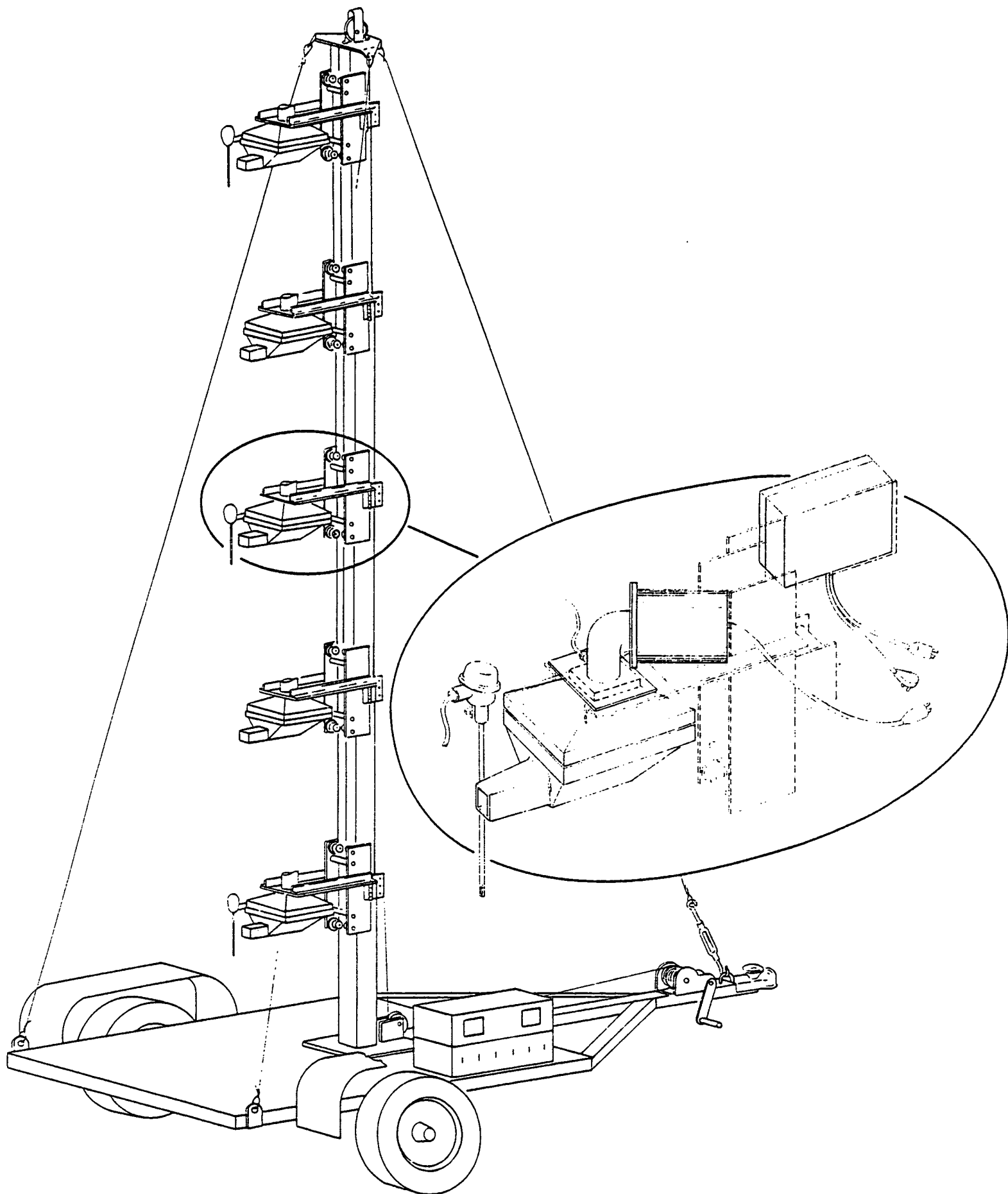
Figure 2. MRI exposure profile tower and equipment.
