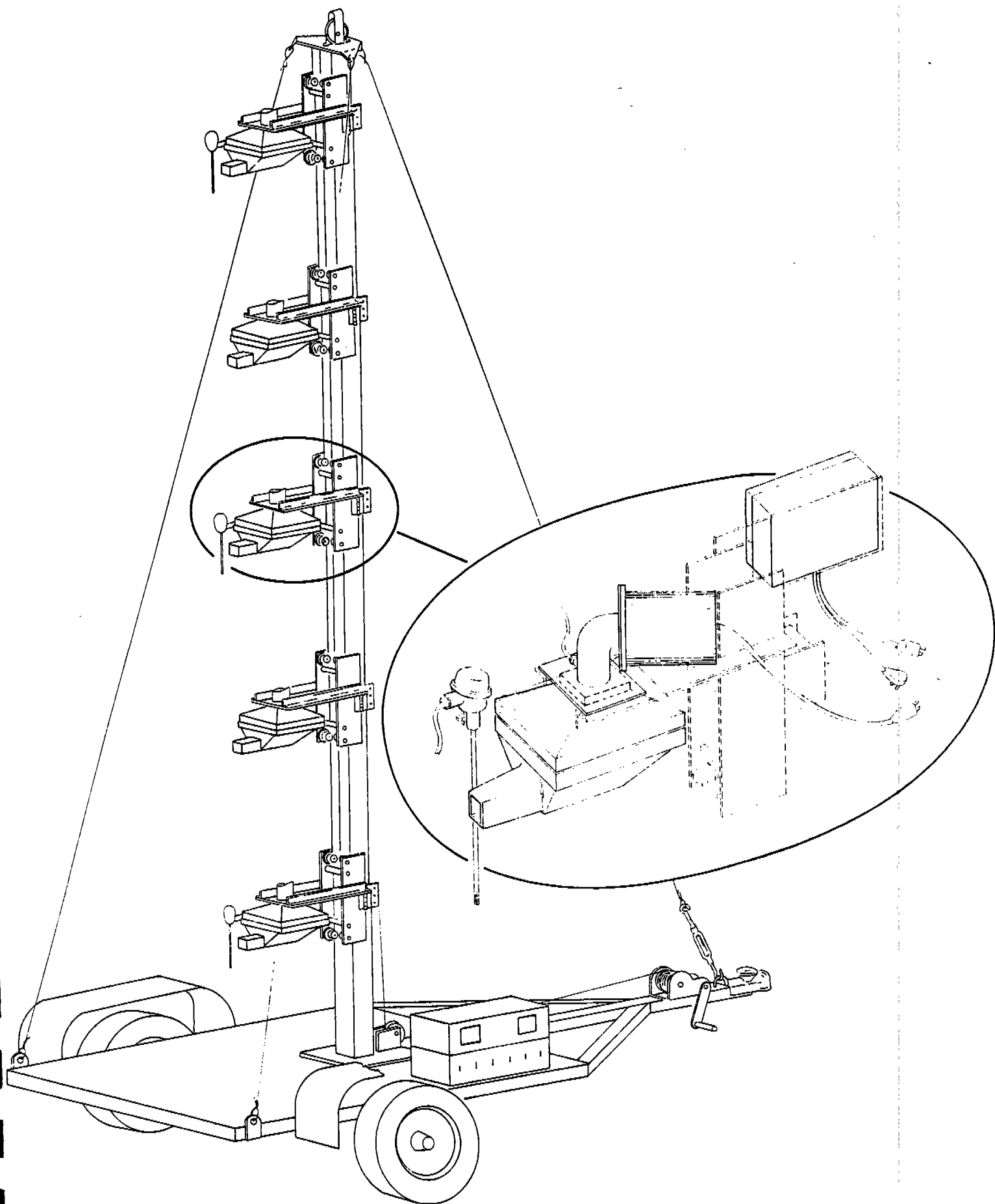
Figure 2. MRI exposure profile tower and equipment.
