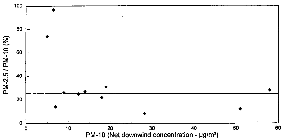
Figure 6-1. Dependence of PM-2.5/PM-10 Ratio on PM-10 Plume Impact
