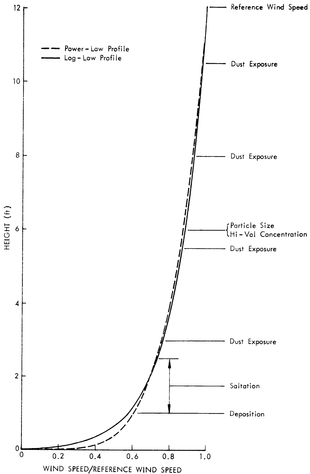
Figure 2. Comparison of wind speed profiles.
