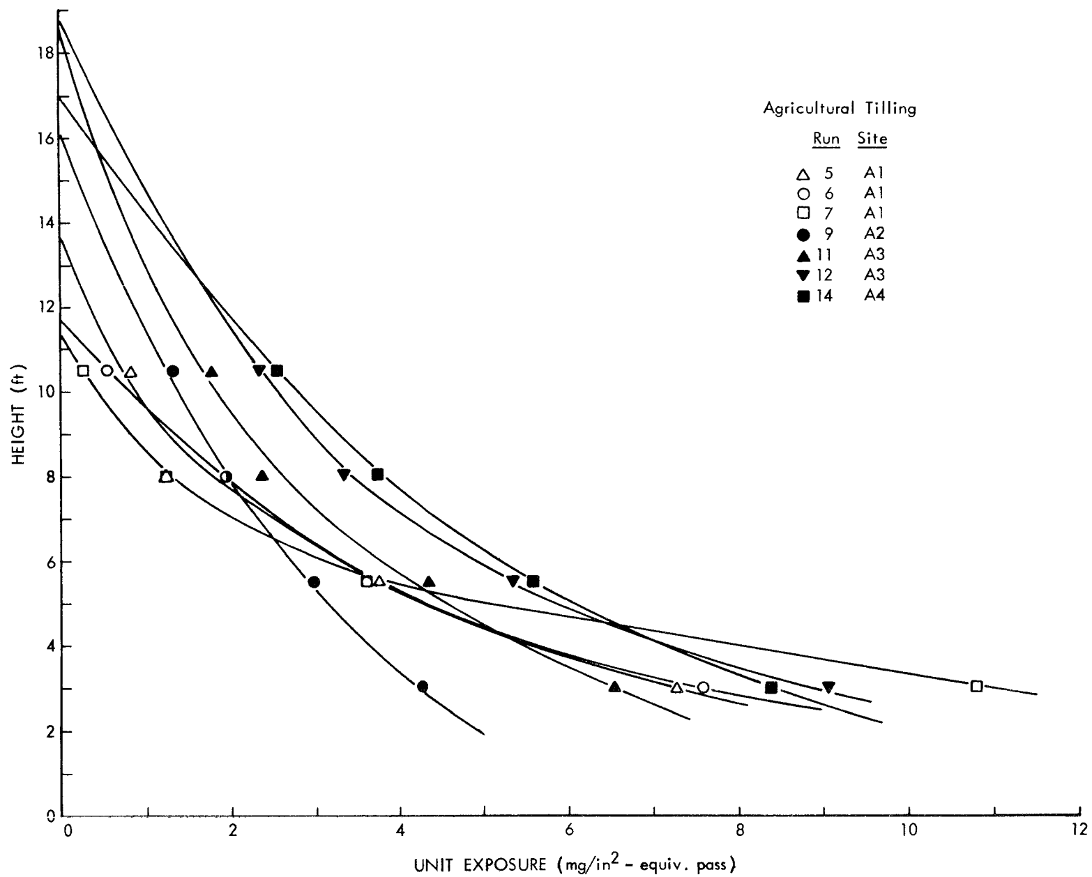
Figure 12. Exposure profiles--agricultural tilling.
