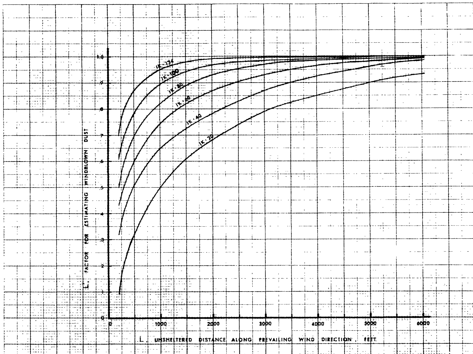
Figure A-5. Effect of field length on relative emission rate.
