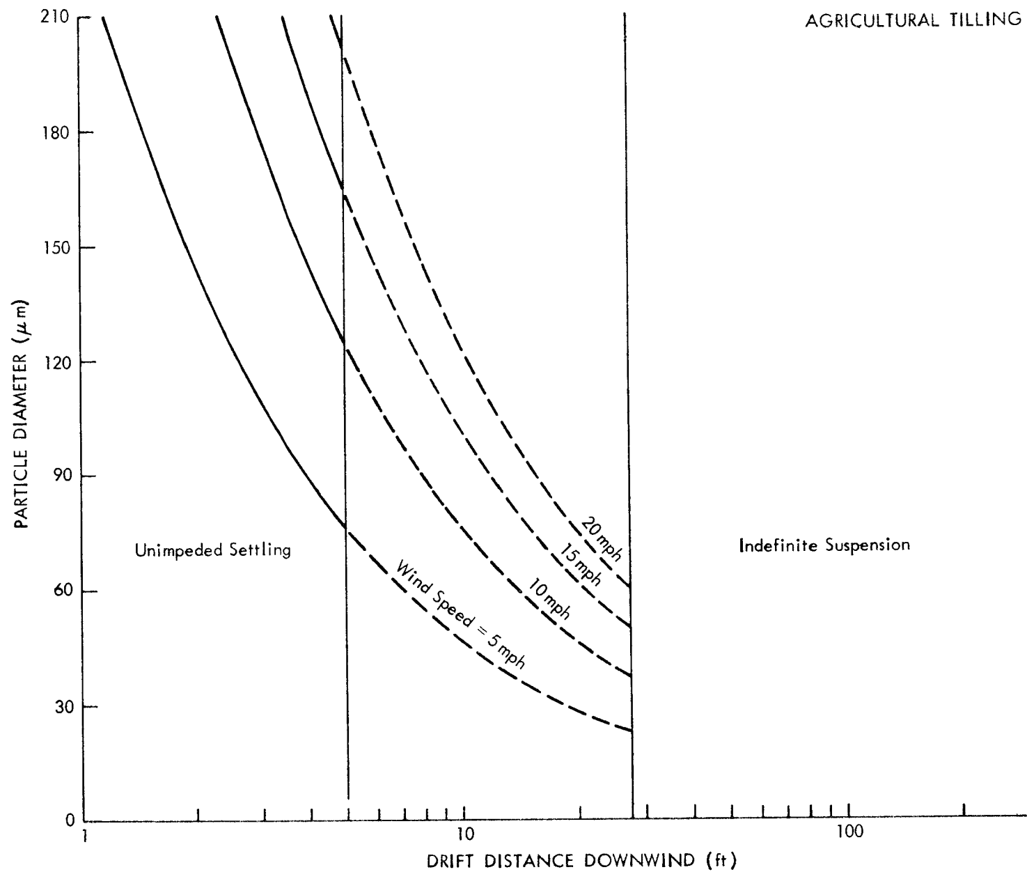
Figure 15. Drift potential of tillage emissions.
