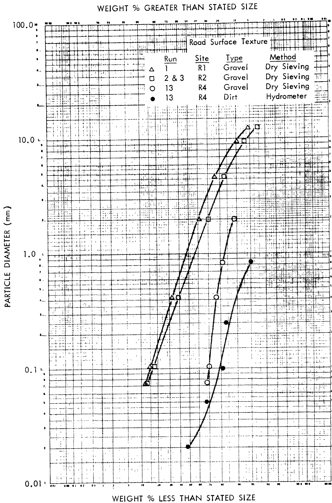
Figure 8. In-place road dust texture.
