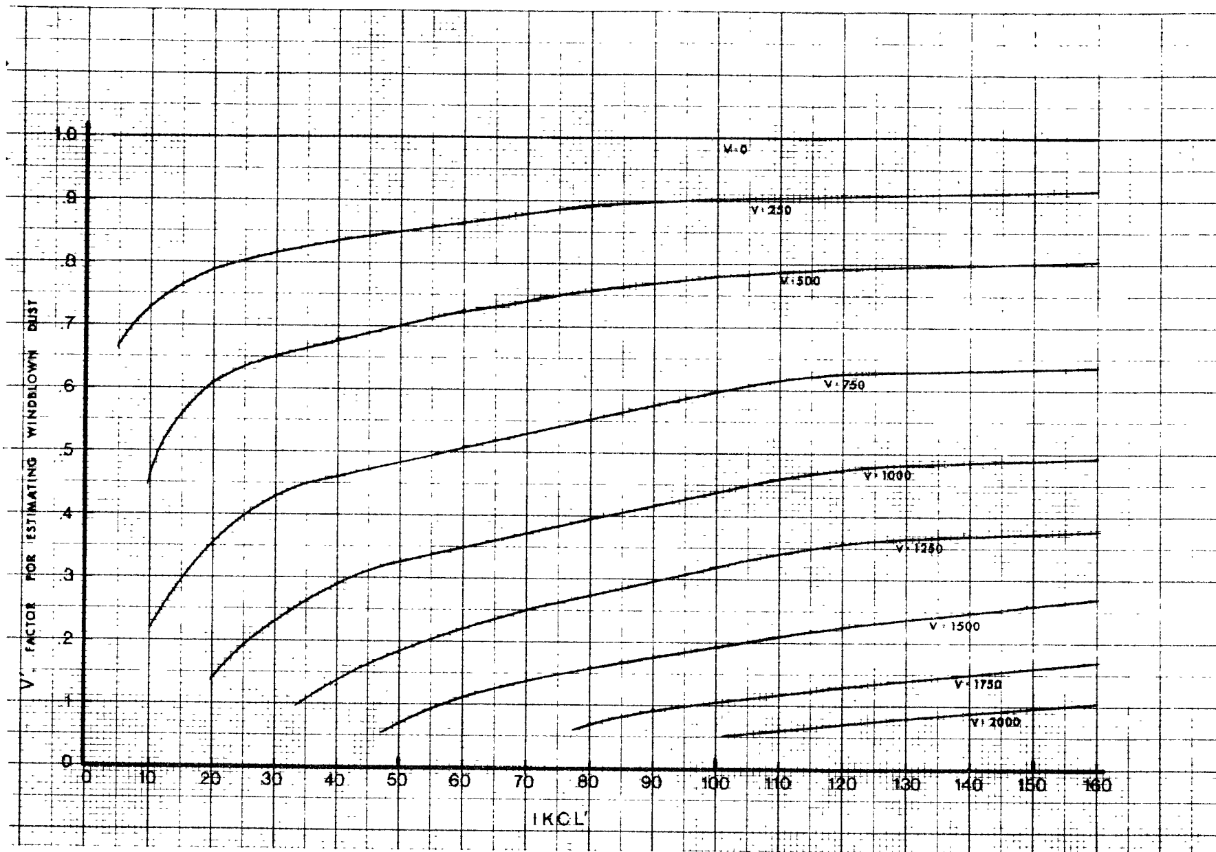
Figure A-6. Effect of vegetative cover on relative emission rate.
