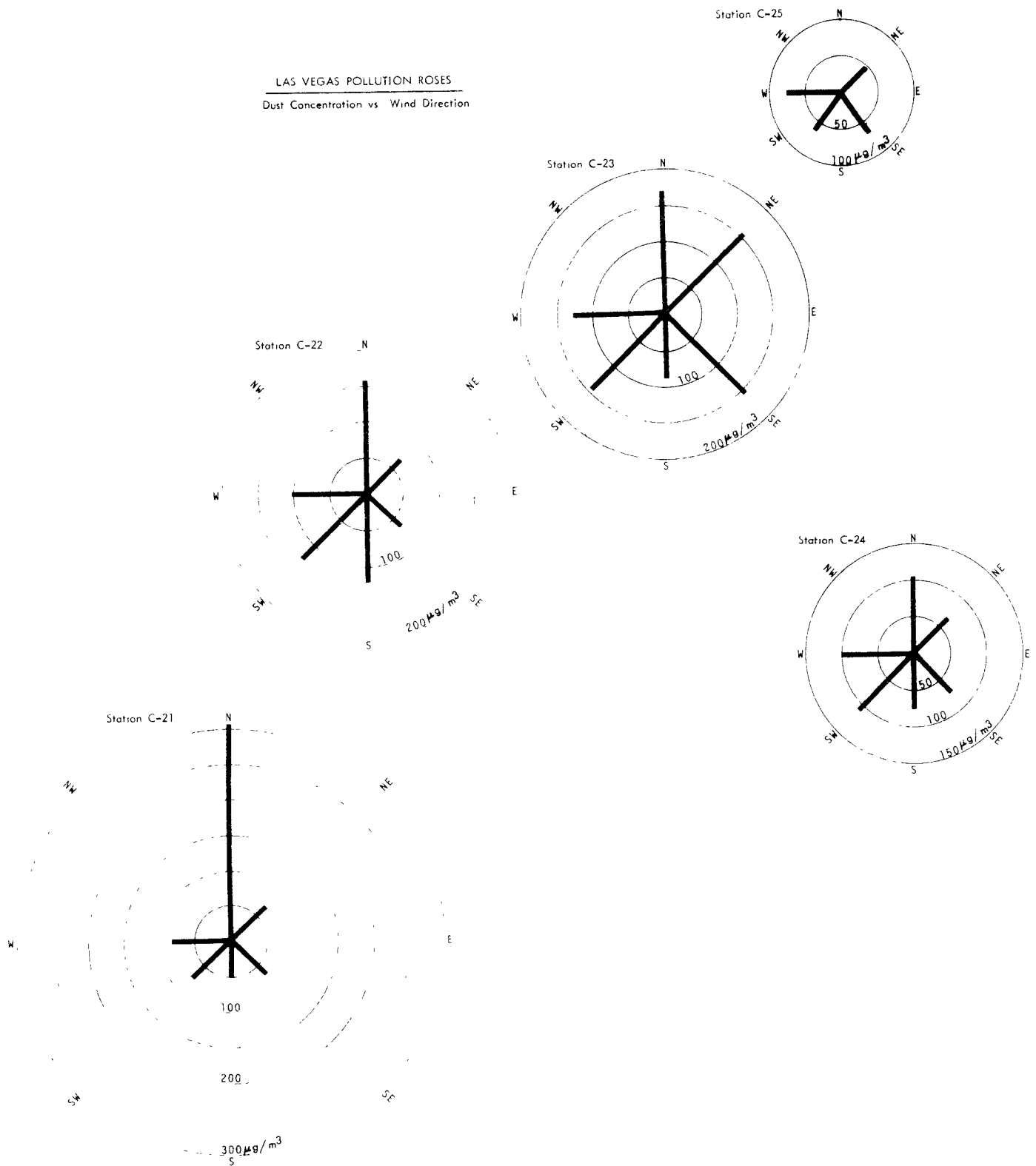
Figure 24. Pollution Roses - Las Vegas Construction Site.
