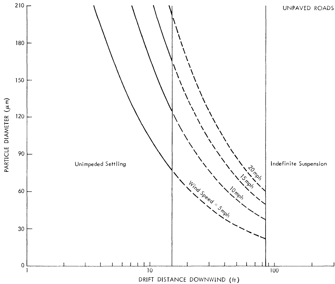
Figure 9. Drift potential of road emissions.
