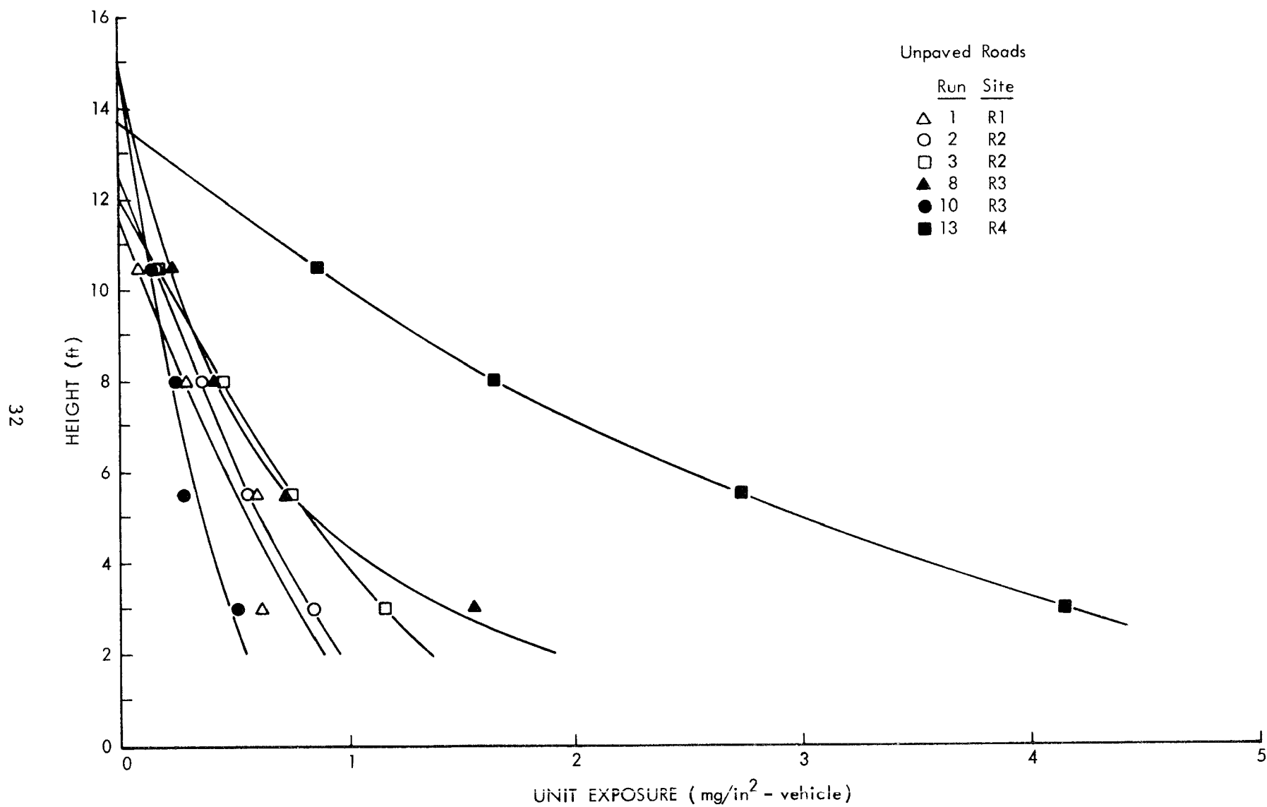
Figure 6. Exposure profiles--unpaved roads.
