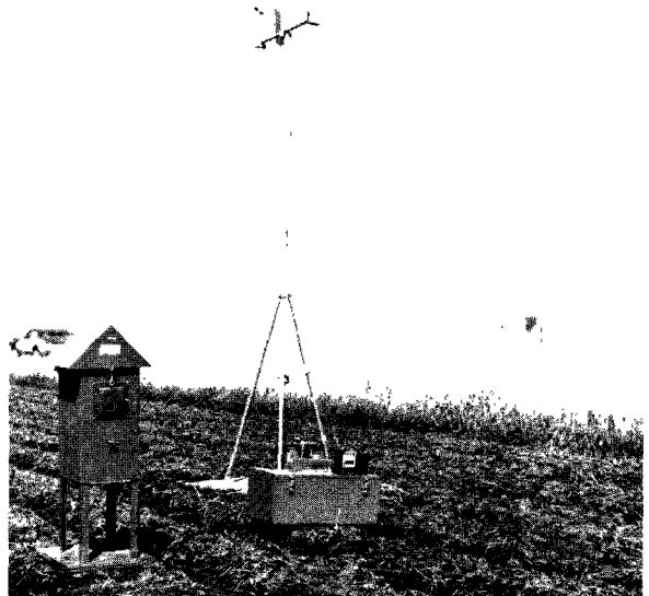
Background Station
