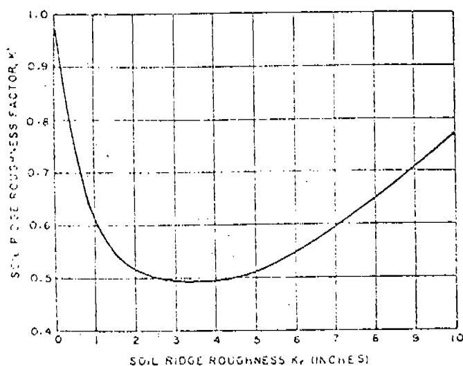
Fig. 4—Chart to determine soil ridge roughness factor K' from the soil ridge roughness K_r .
