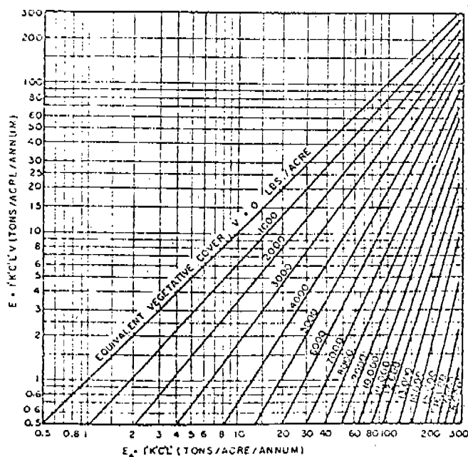
Fig. 10—Chart to determine soil loss E = I'K'C'L'V from soil loss E_4 = I'K'C'L' and from the vegetative cover factor, V . The chart can be used in reverse to determine V needed to reduce soil loss to any degree.
