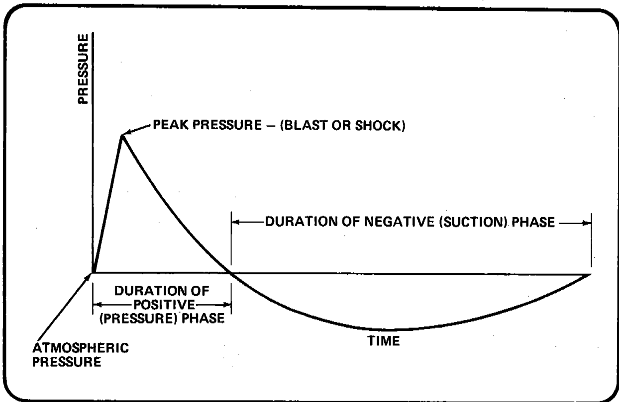
Figure 6 TIME PHASES OF A BLAST WAVE
