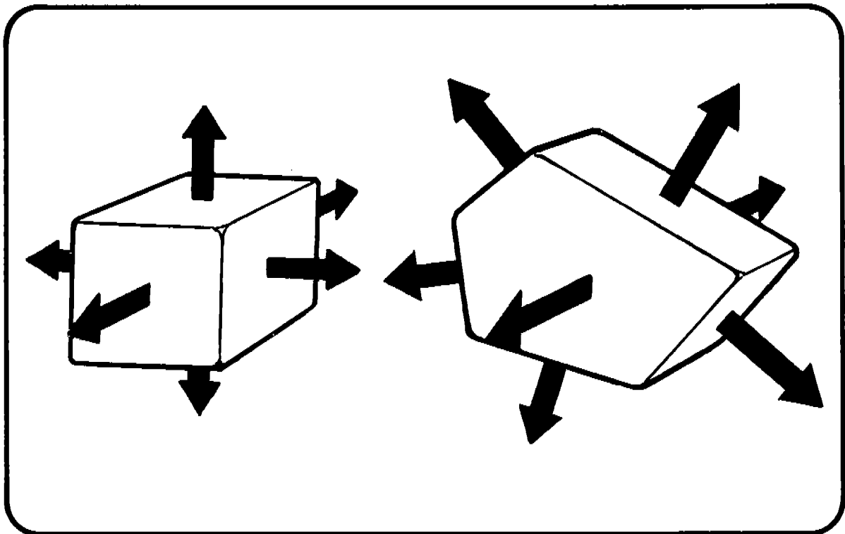
Figure 11 RESULTING DIRECTIONAL EXPLOSIVE FORCES
