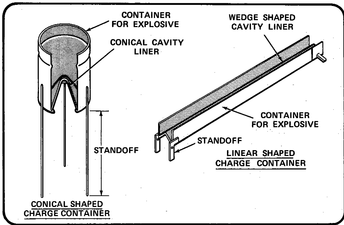
Figure 14 SHAPED CHARGE CONTAINERS
