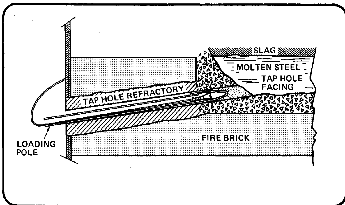
Figure 16 CROSS SECTION OF OPEN HEARTH FURNACE TAP HOLE SHOWING JET TAPPER IN POSITION FOR FIRING
