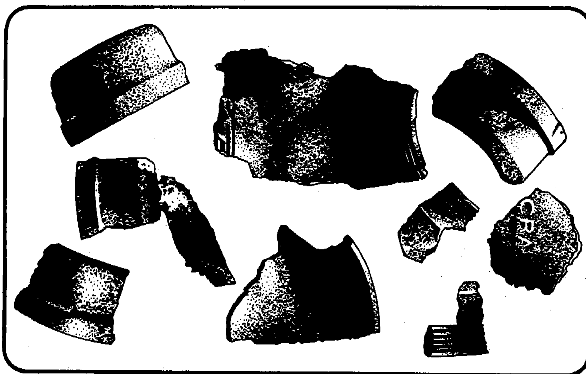
Figure 8 PIPE BOMB FRAGMENTS
