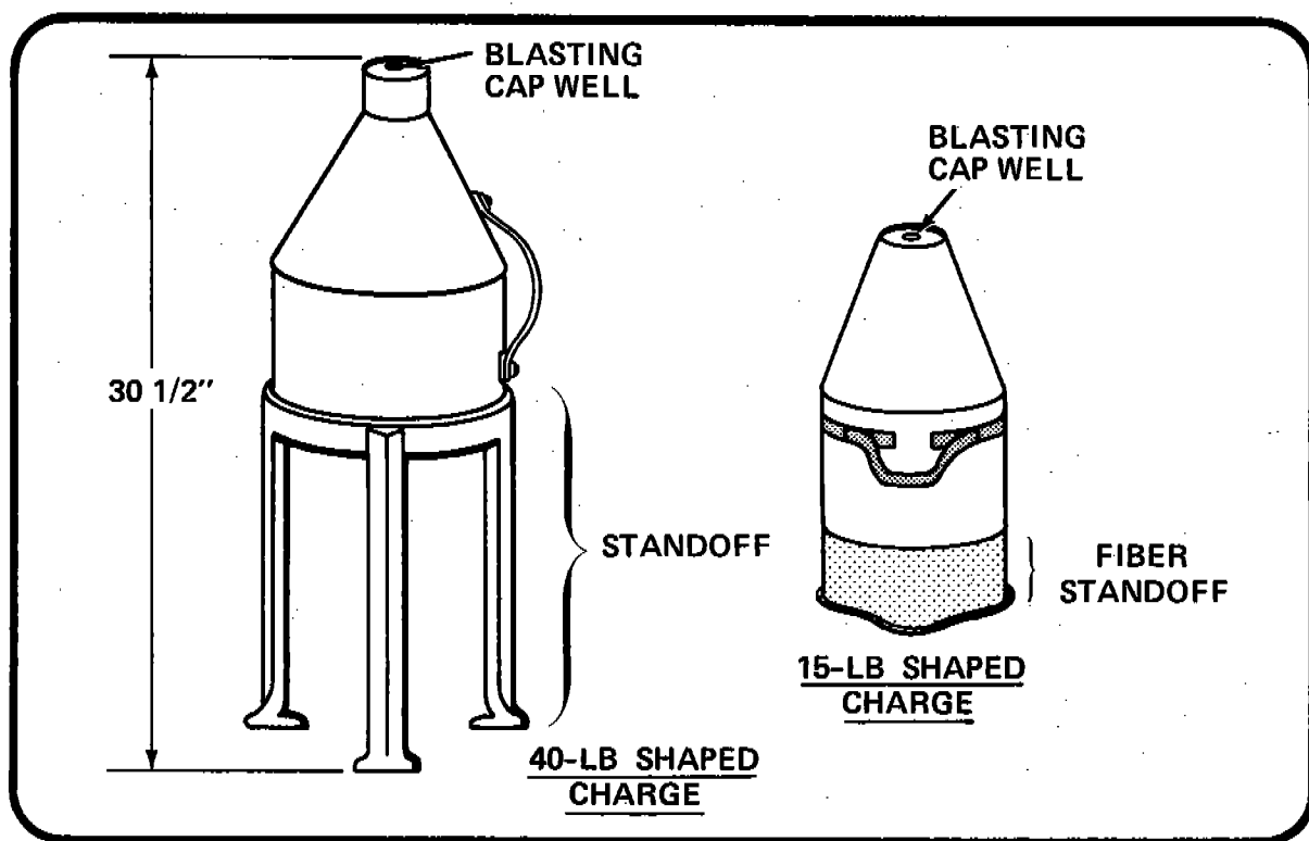
Figure 19 STANDARD MILITARY SHAPED CHARGES
