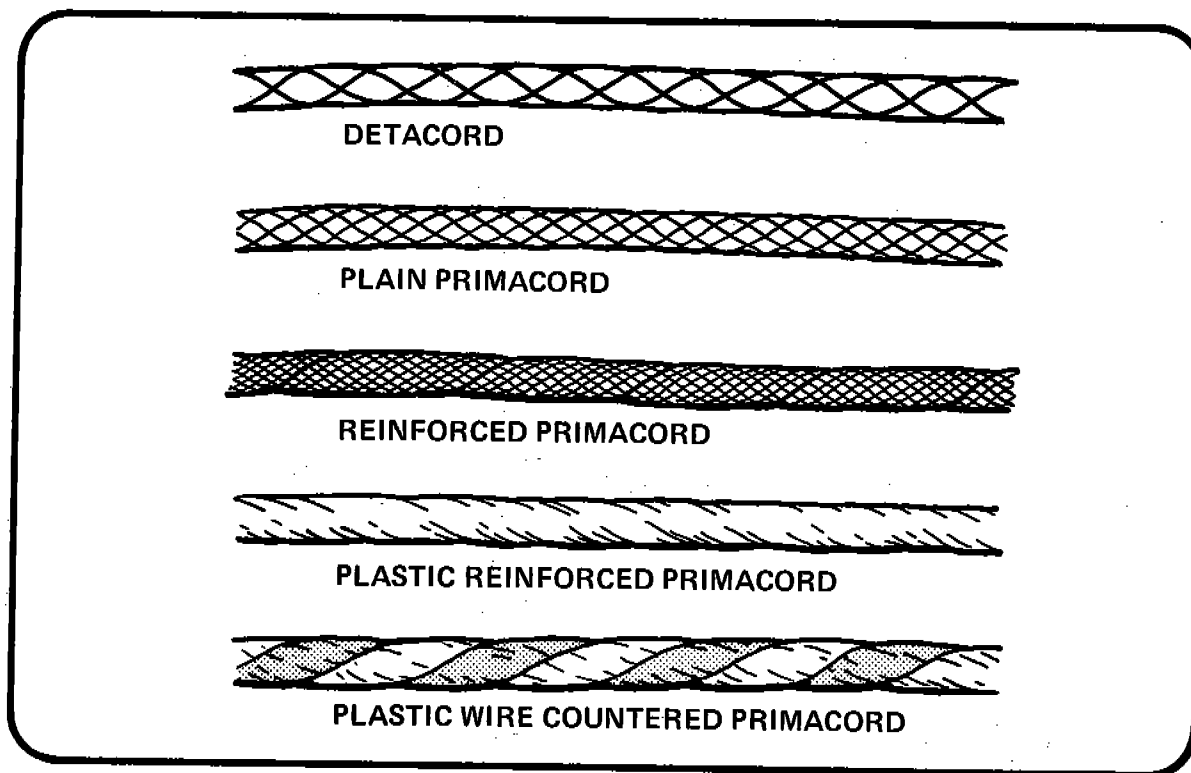
Figure 30 DUPONT DETONATING CORD MARKINGS
