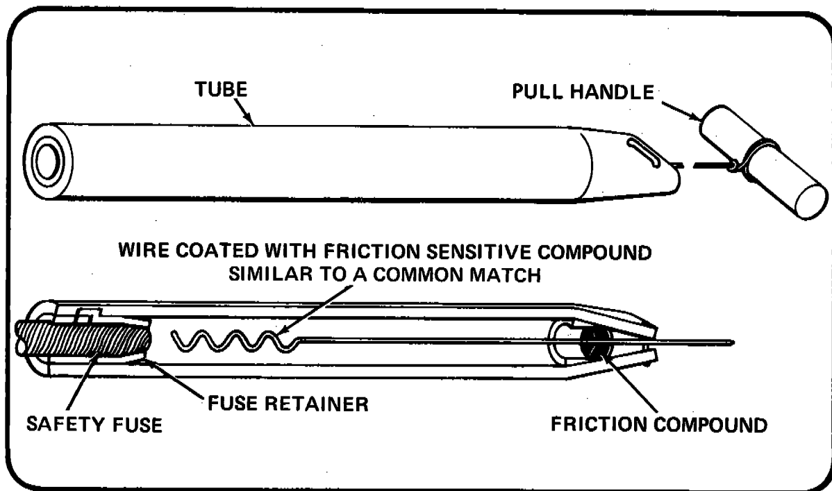
Figure 57 FRICTION TYPE FUSE IGNITER
