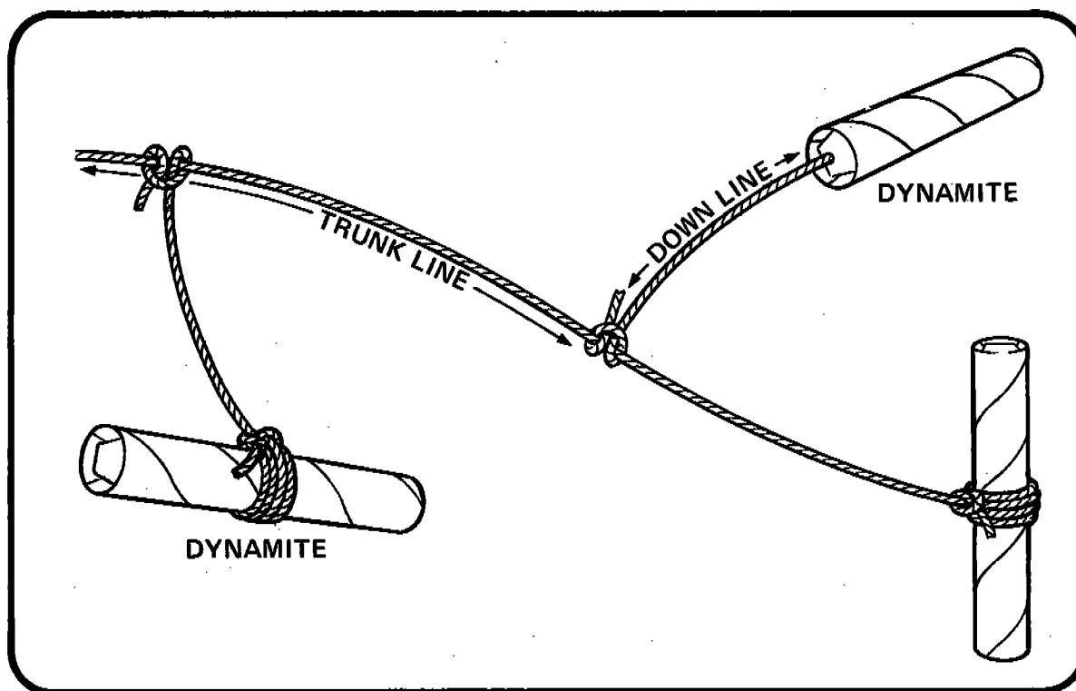
Figure 32 USE OF DETONATING CORD FOR SIMULTANEOUS NONELECTRIC DETONATION OF EXPLOSIVE CHARGES
