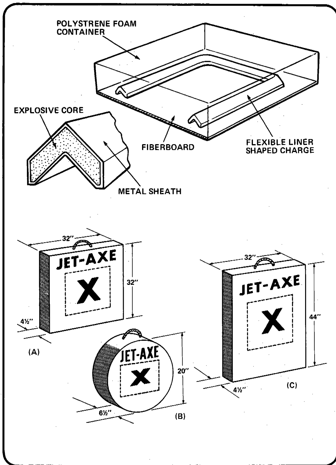
Figure 17 CONFIGURATION AND CONTAINERS OF JET-AXE LINEAR SHAPED CHARGE
