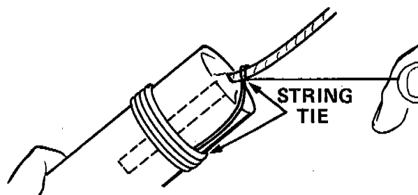
(A) NONELECTRIC BLASTING CAP
