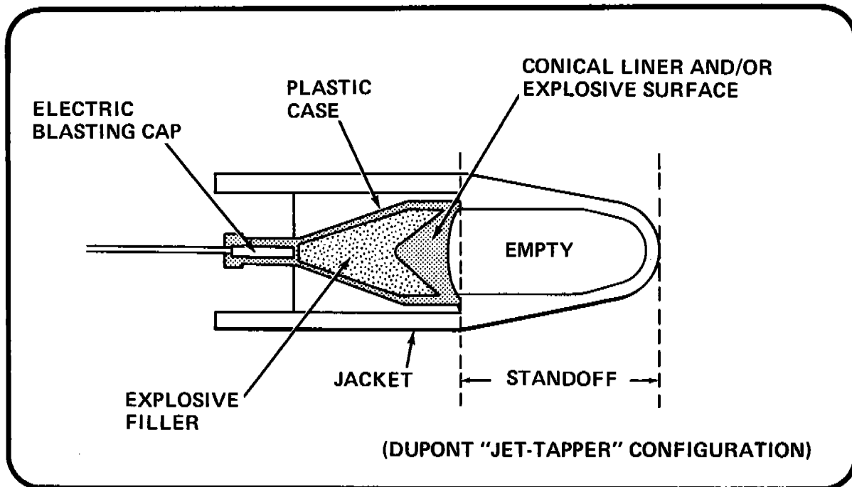
Figure 15 A TYPE OF COMMERCIAL CONICAL SHAPED CHARGE
