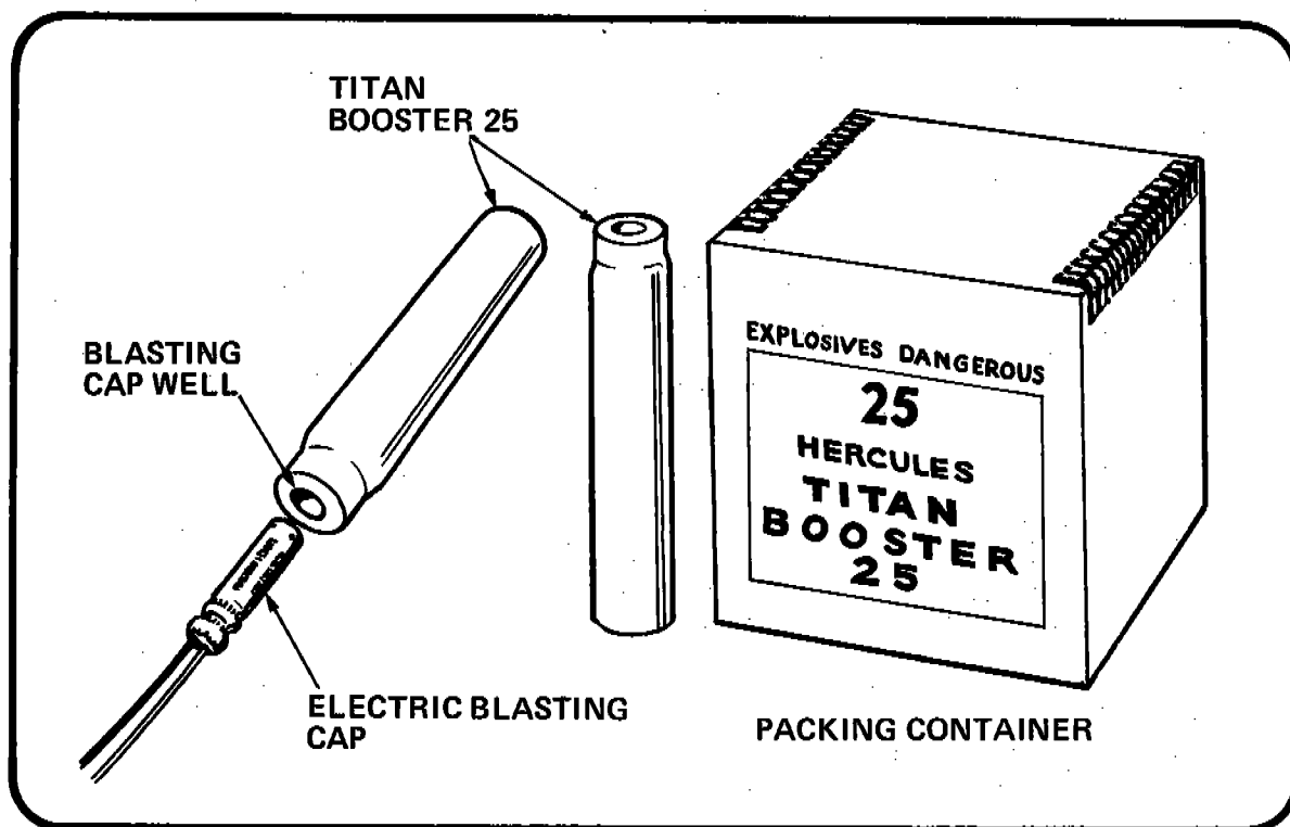
Figure 34 HERCULES TITAN BOOSTER 25
