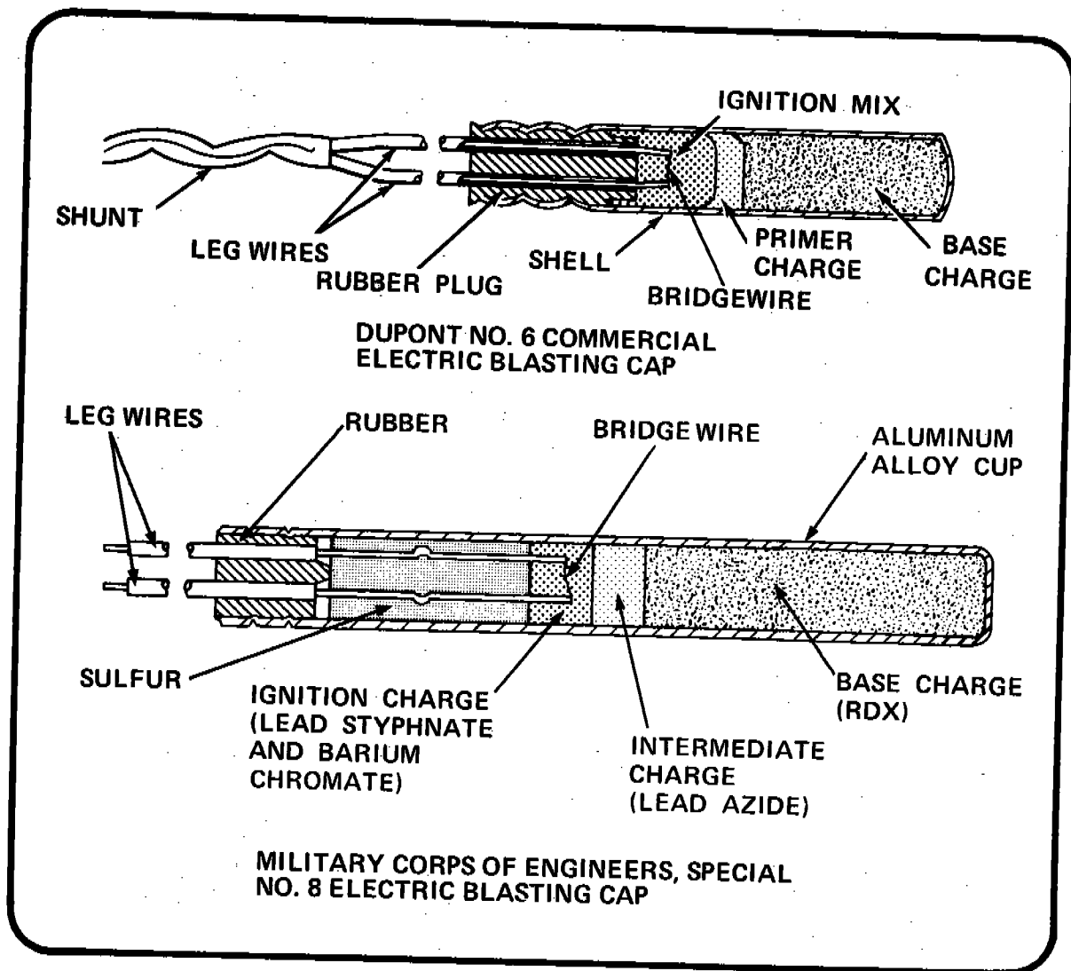
Figure 25 ELECTRIC BLASTING CAPS
