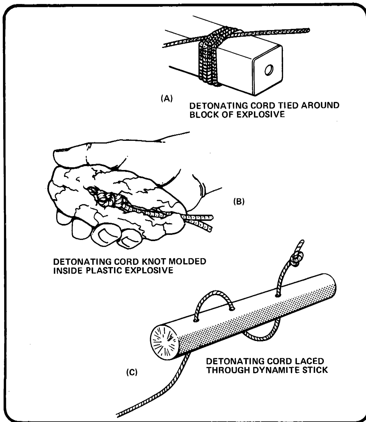
Figure 31 EXAMPLE OF USING DETONATING CORD TO PRIME EXPLOSIVE CHARGES
