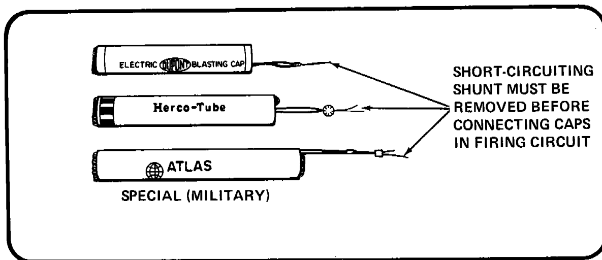
Figure 26 EXAMPLES OF PACKING AROUND ELECTRIC BLASTING CAPS
