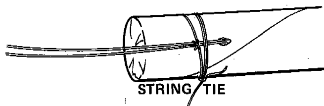
(B) ELECTRIC BLASTING CAP
