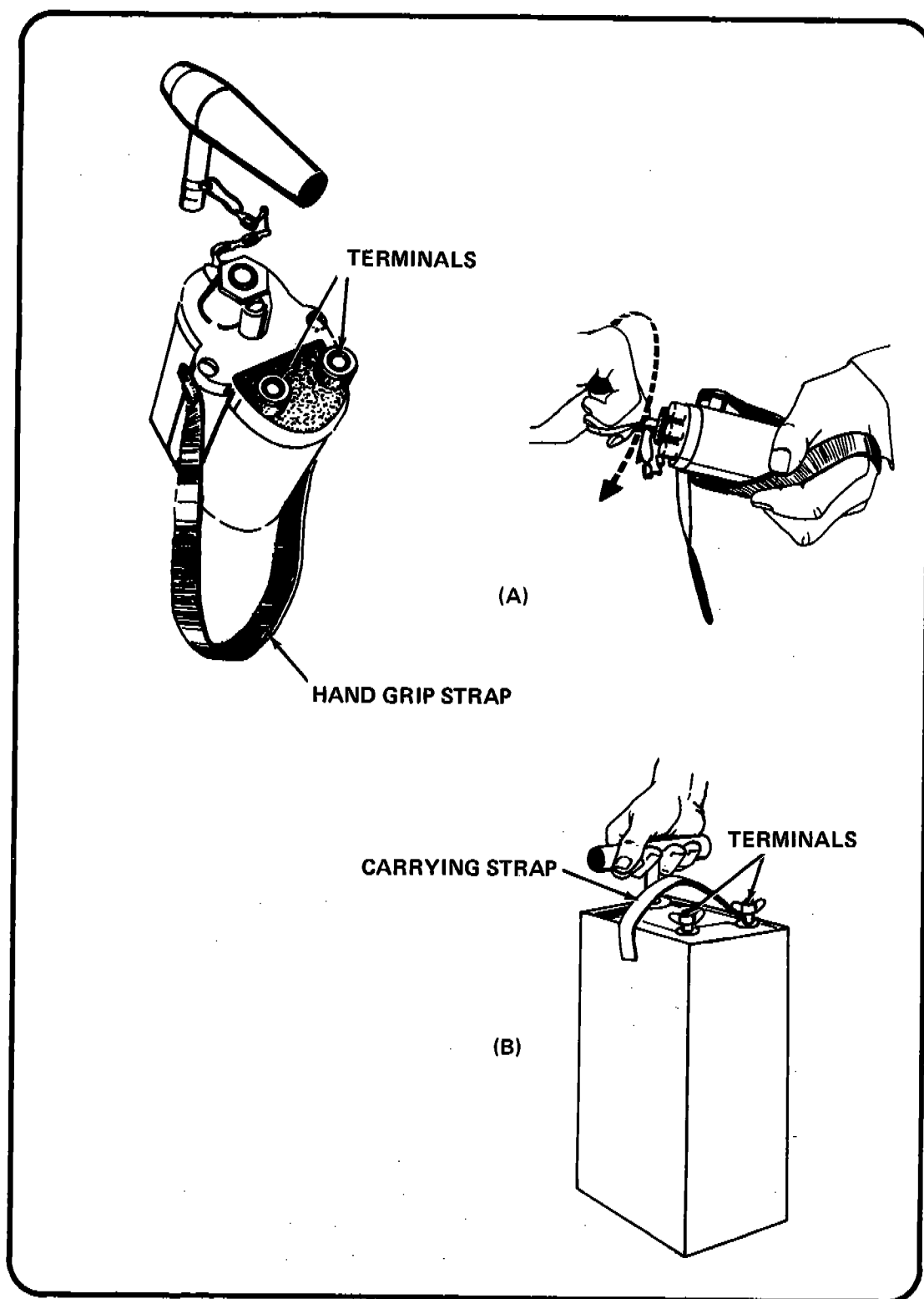
Figure 66 TWIST TYPE (A) AND PLUNGER TYPE (B) BLASTING MACHINES
