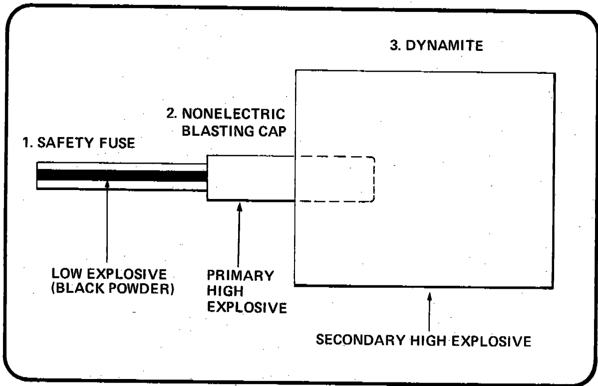
Figure 22 THREE-STEP EXPLOSIVE TRAIN
