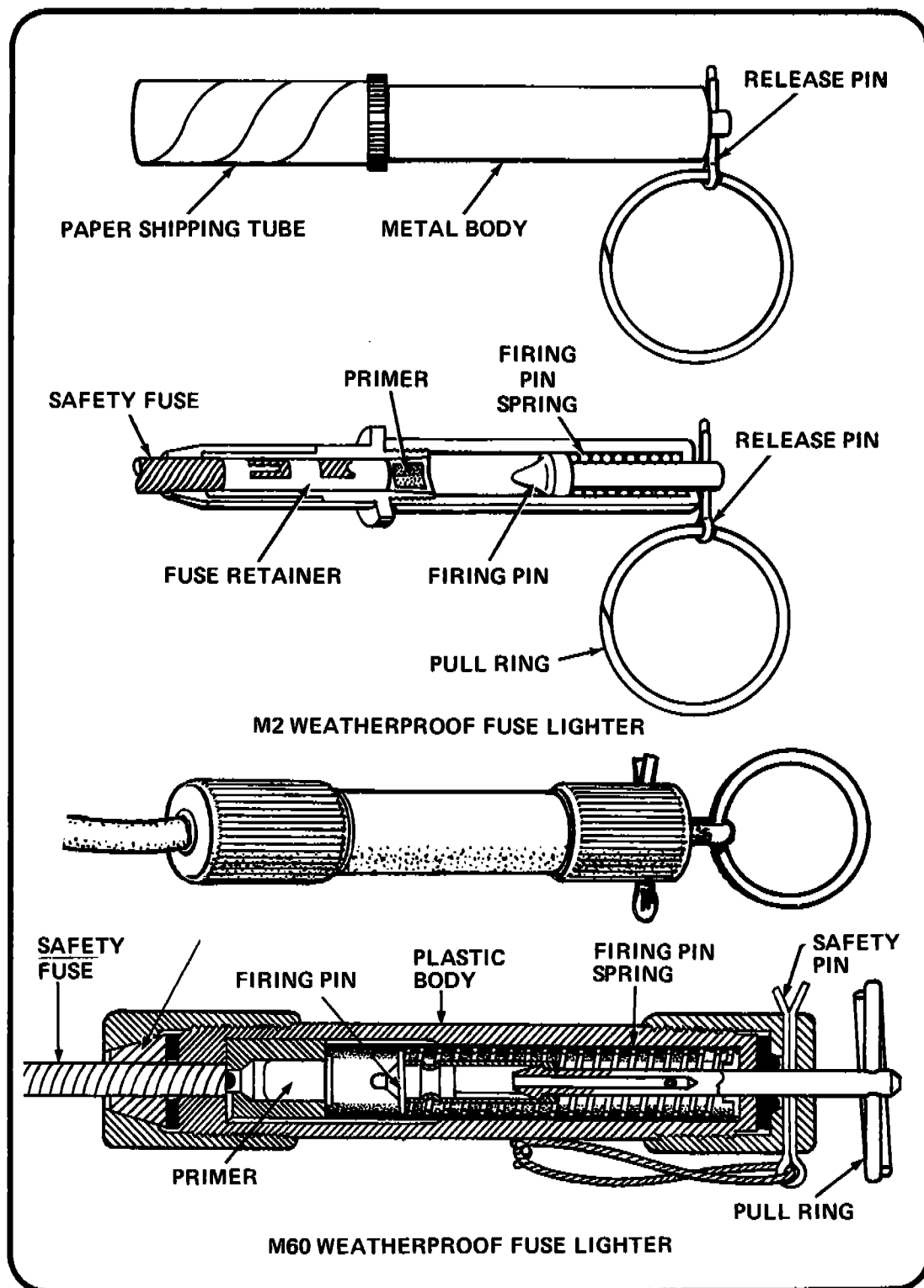
Figure 58 PERCUSSION FUSE IGNITERS
