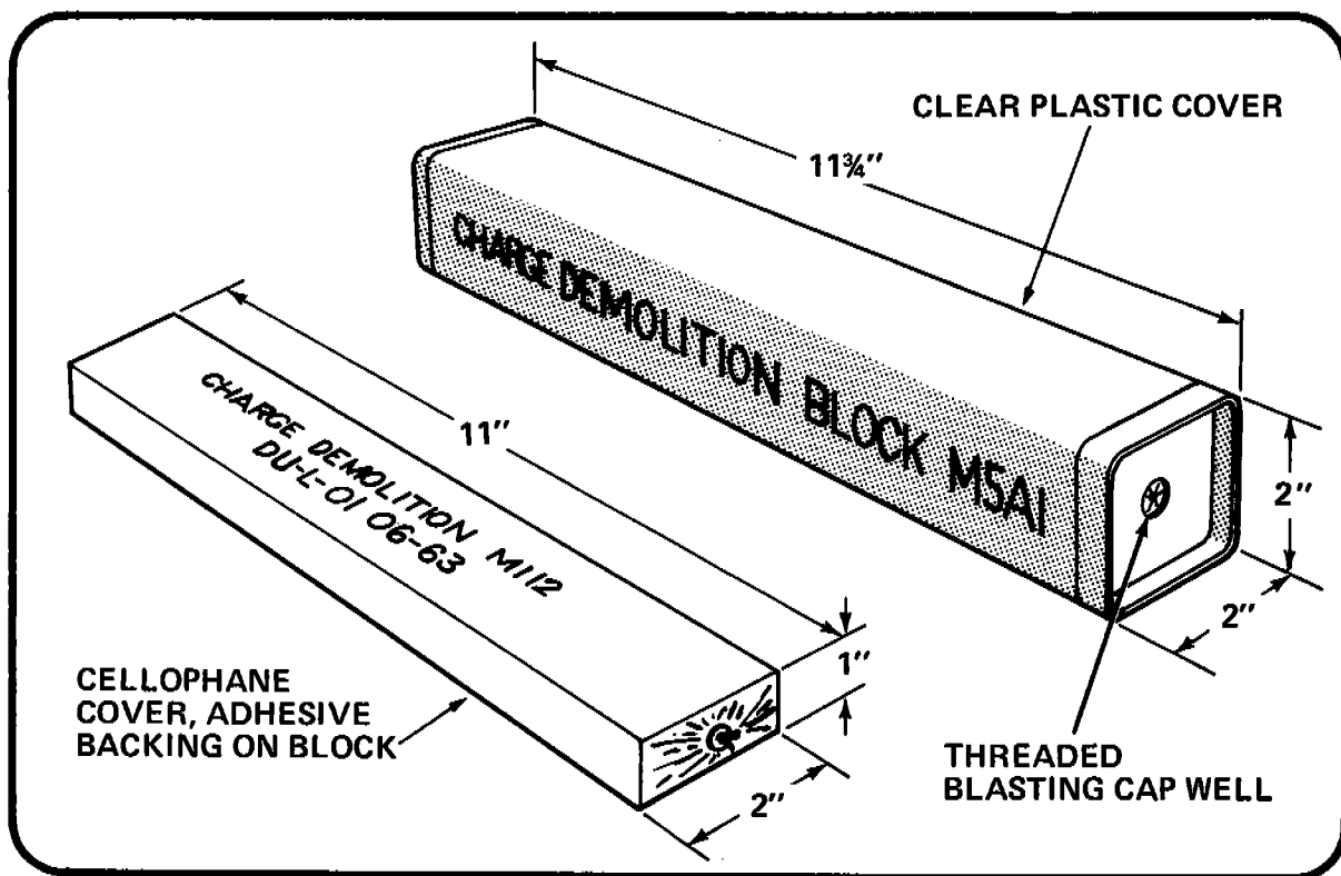
Figure 45 COMPOSITION C-4 DEMOLITION BLOCKS
