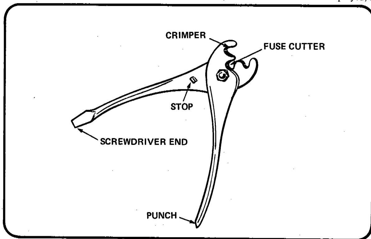
Figure 55 BLASTING CAP CRIMPING TOOL
