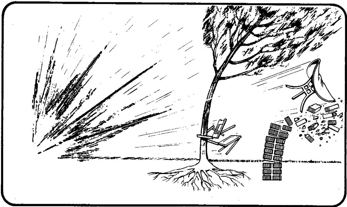
Figure 3 POSITIVE PRESSURE PHASE OF AN EXPLOSION
