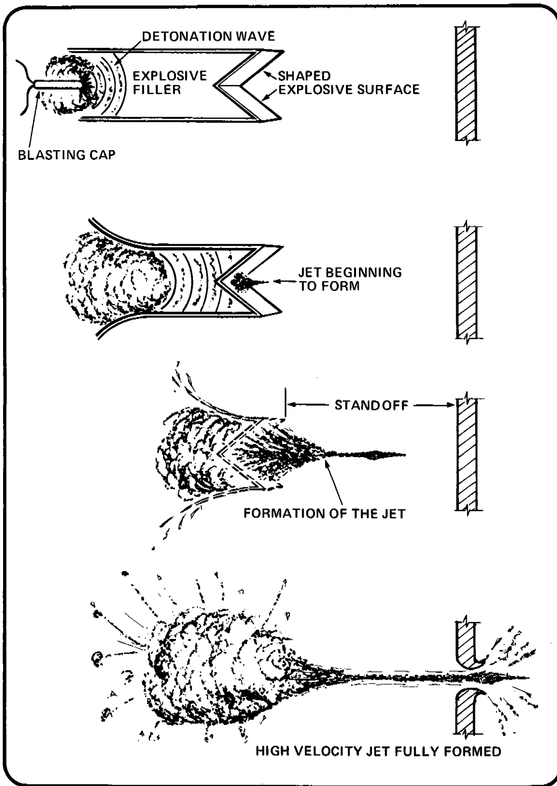
Figure 13 SHAPED CHARGE JET FORMATION
