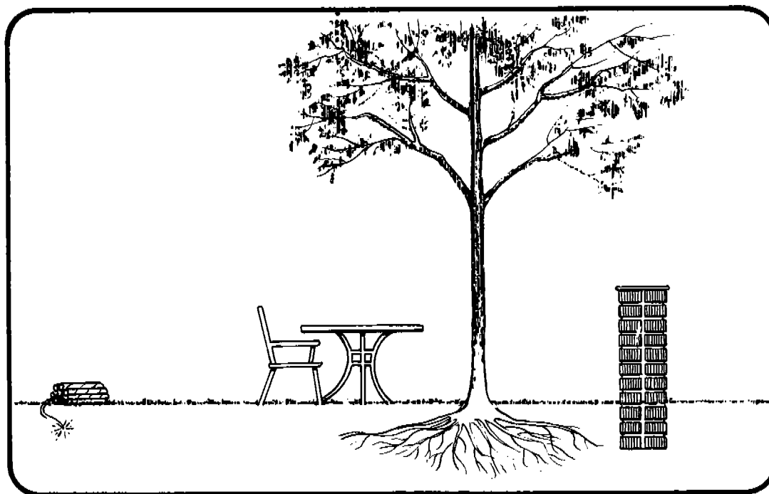
Figure 2 CONDITIONS PRIOR TO EXPLOSION
