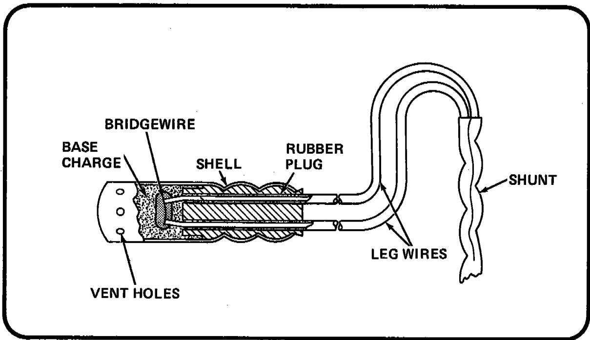
Figure 61 TYPICAL VENTED ELECTRIC SQUIB
