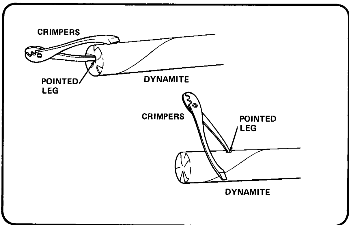
Figure 37 PREPARING DYNAMITE STICKS FOR INSERTION OF THE BLASTING CAP
