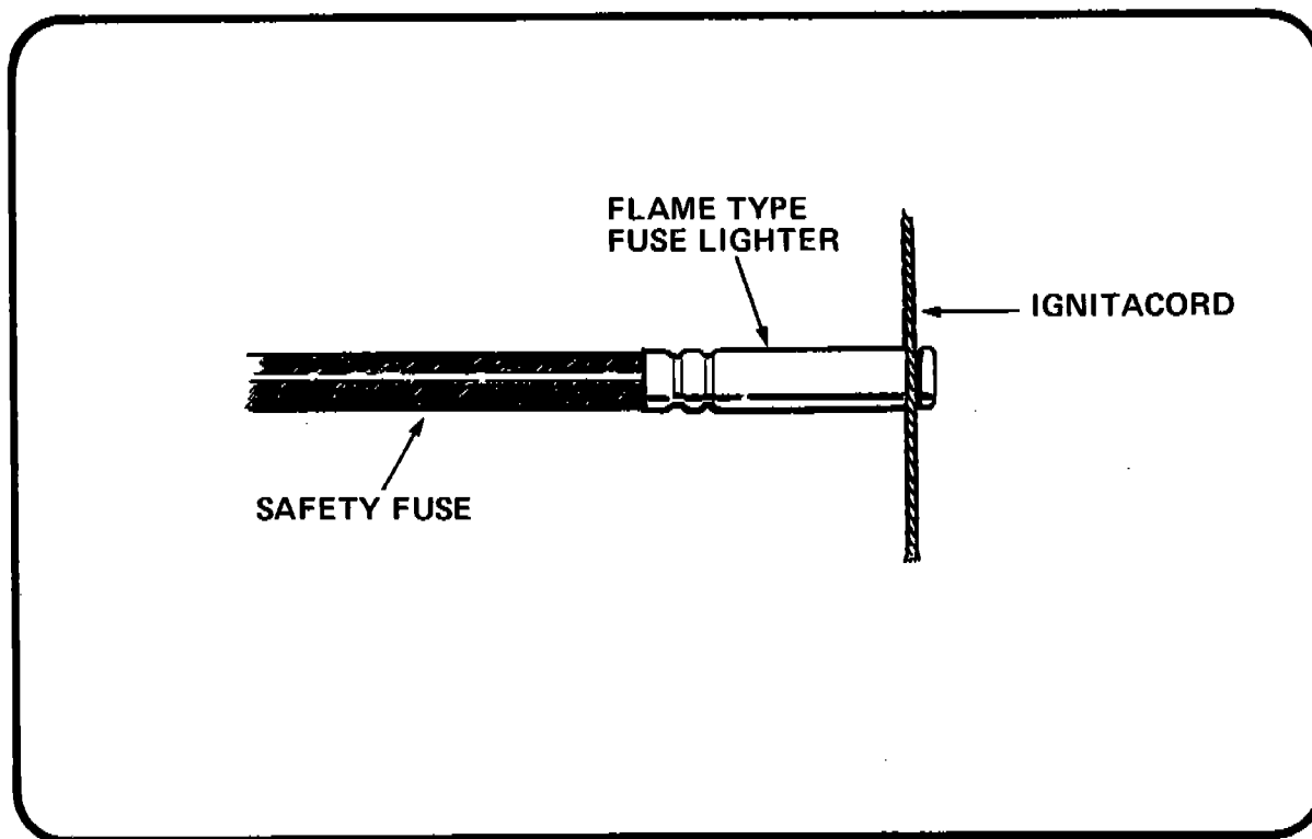
Figure 60 THERMALITE IGNITACORD INSERTED IN IGNITION SLOT OF FLAME TYPE FUSE LIGHTER
