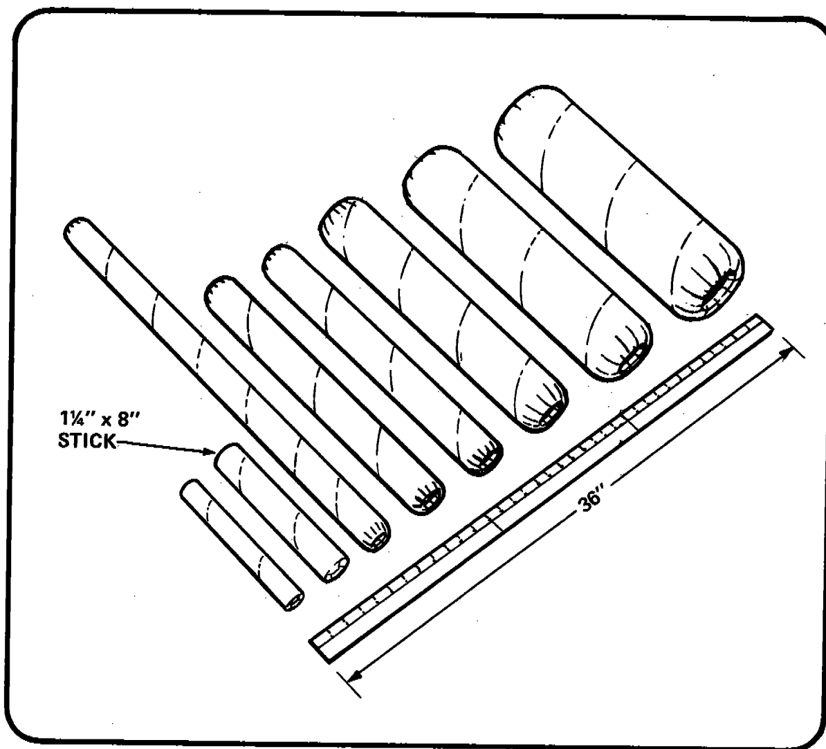
Figure 35 STANDARD DYNAMITE CARTRIDGE SIZES
