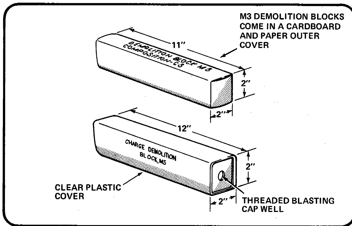
Figure 44 COMPOSITION C-3 DEMOLITION BLOCKS
