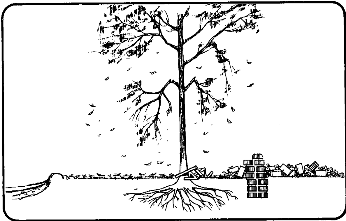
Figure 5 CONDITIONS AFTER AN EXPLOSION
