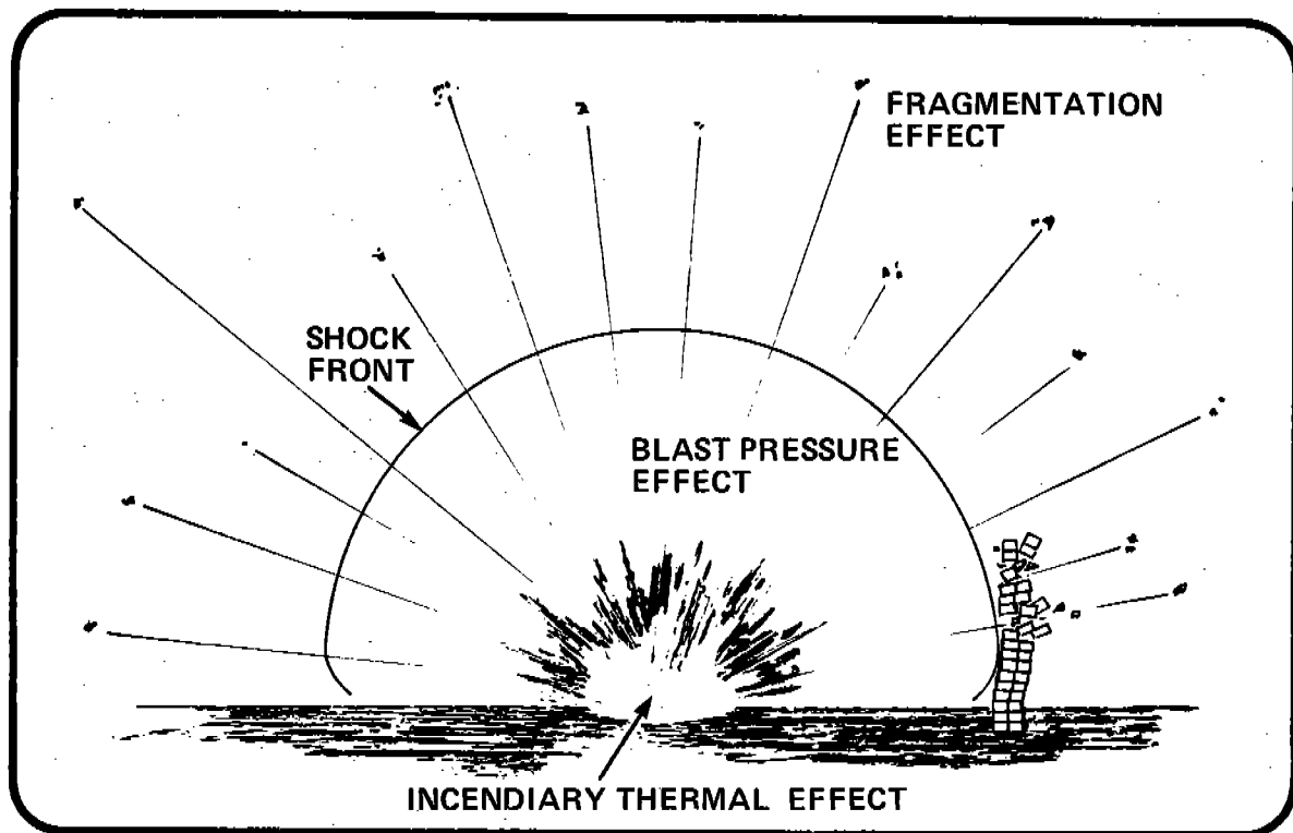
Figure 1 EFFECTS OF AN EXPLOSION
