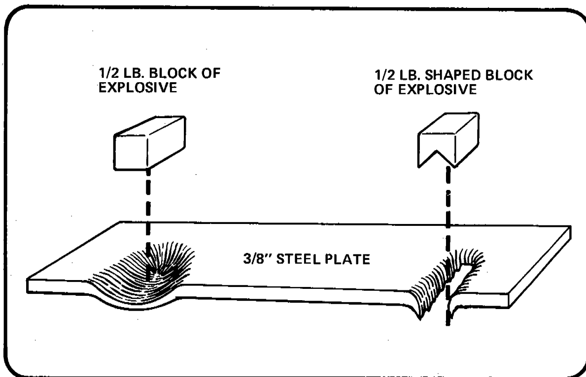
Figure 12 INCREASED EFFECT OF SHAPED EXPLOSIVE
