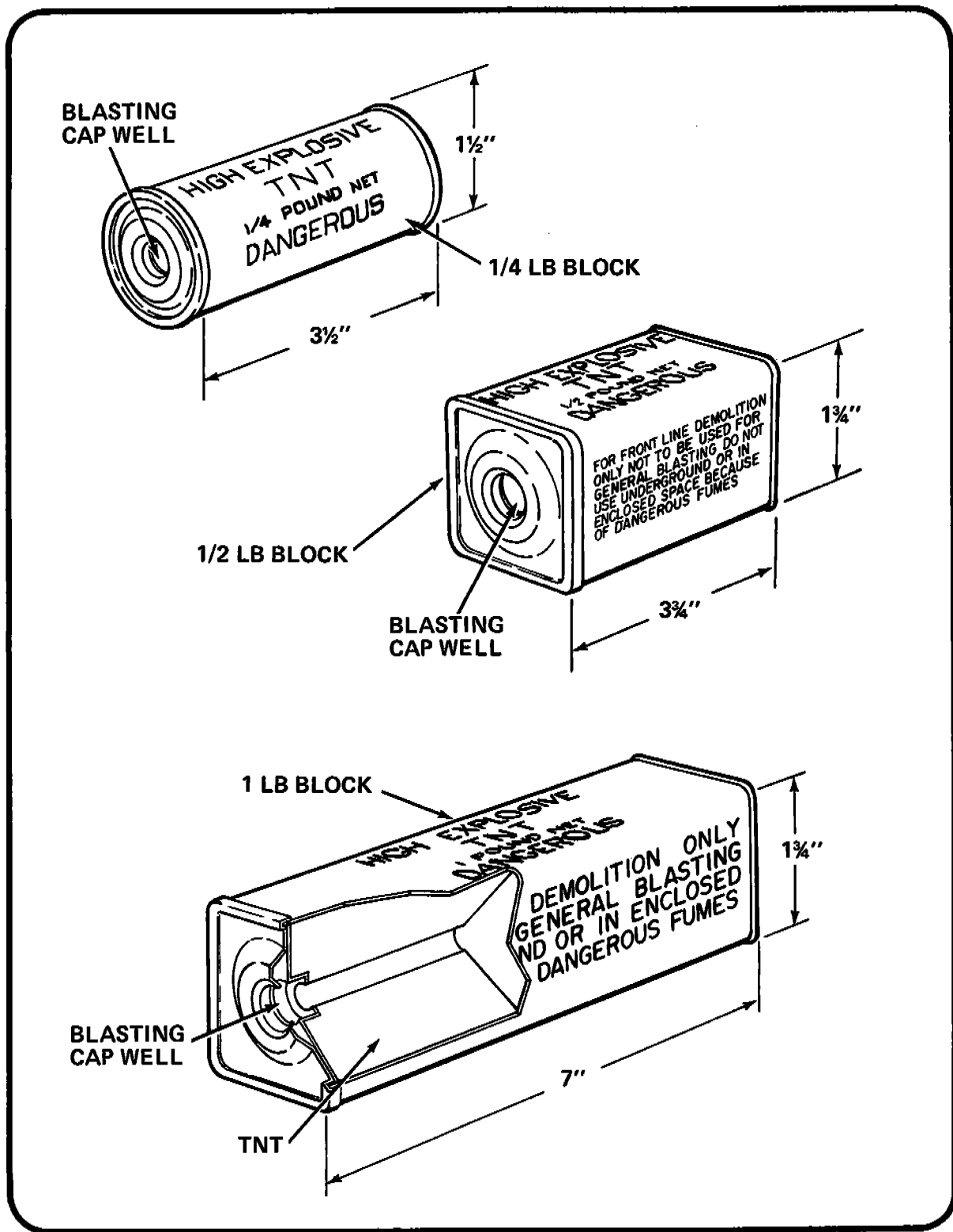
Figure 42 MILITARY TNT BLOCKS
