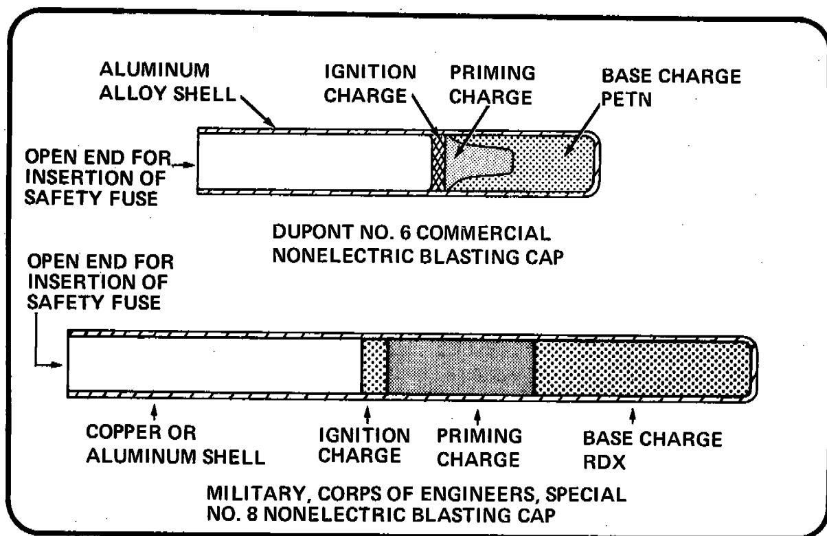
Figure 28 NONELECTRIC BLASTING CAPS
