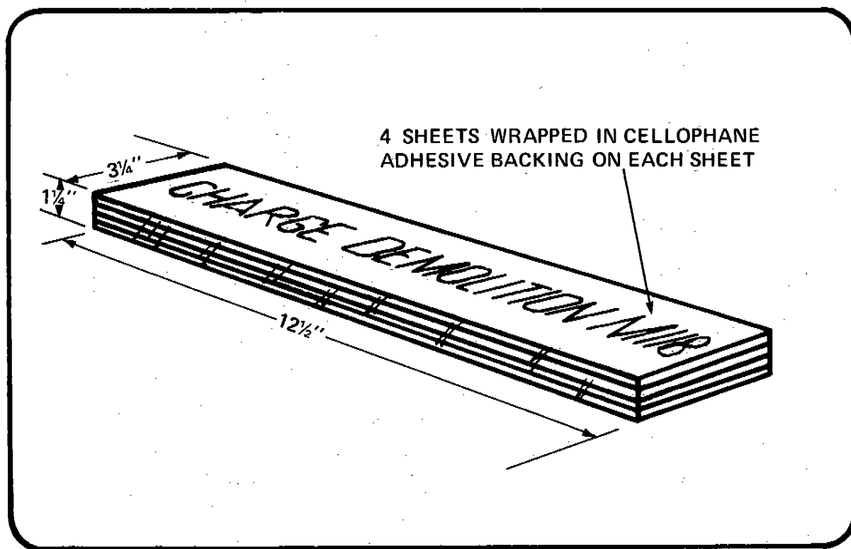
Figure 46 M118 MILITARY SHEET PETN DEMOLITION CHARGE
