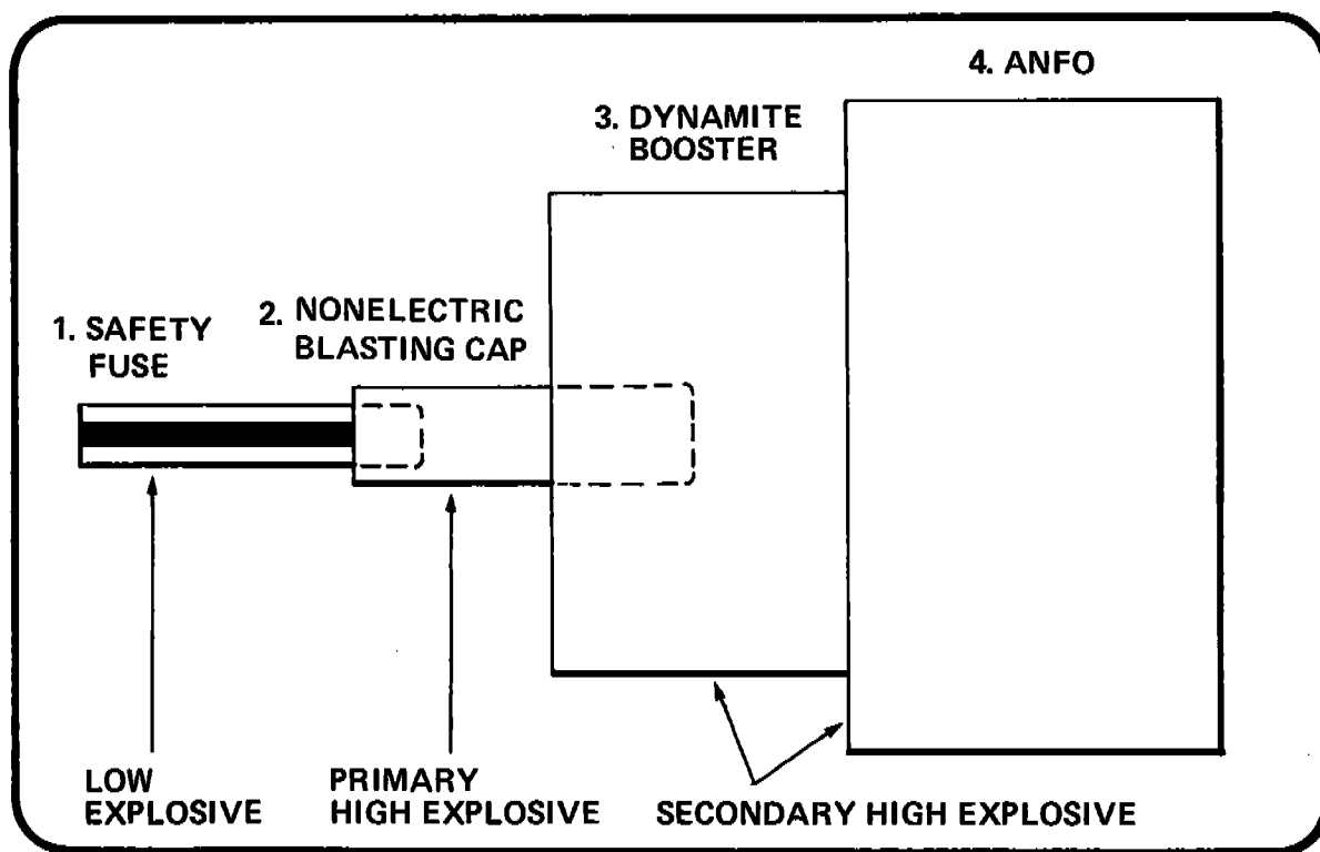
Figure 23 FOUR-STEP EXPLOSIVE TRAIN
