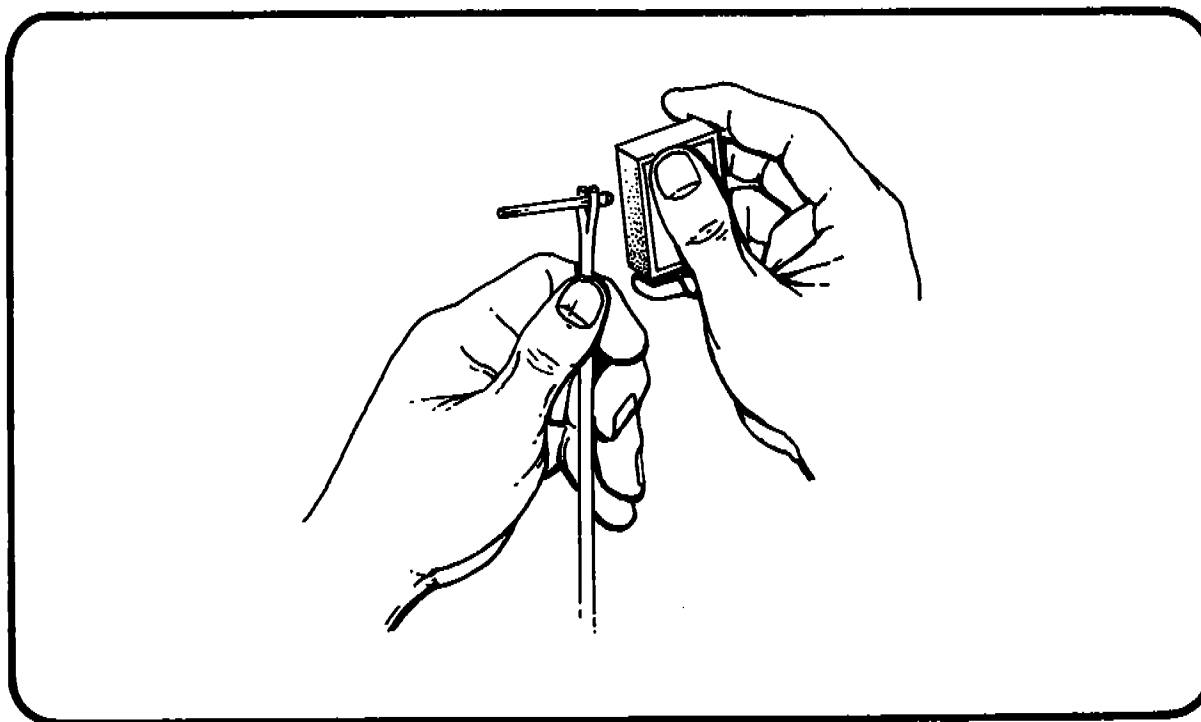
Figure 56 IGNITING SAFETY BLASTING FUSE WITH MATCHES
