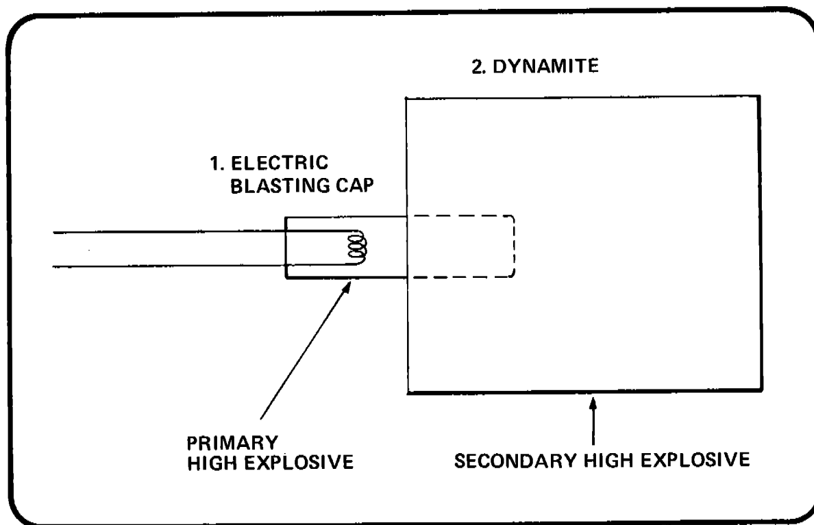
Figure 21 TWO-STEP EXPLOSIVE TRAIN
