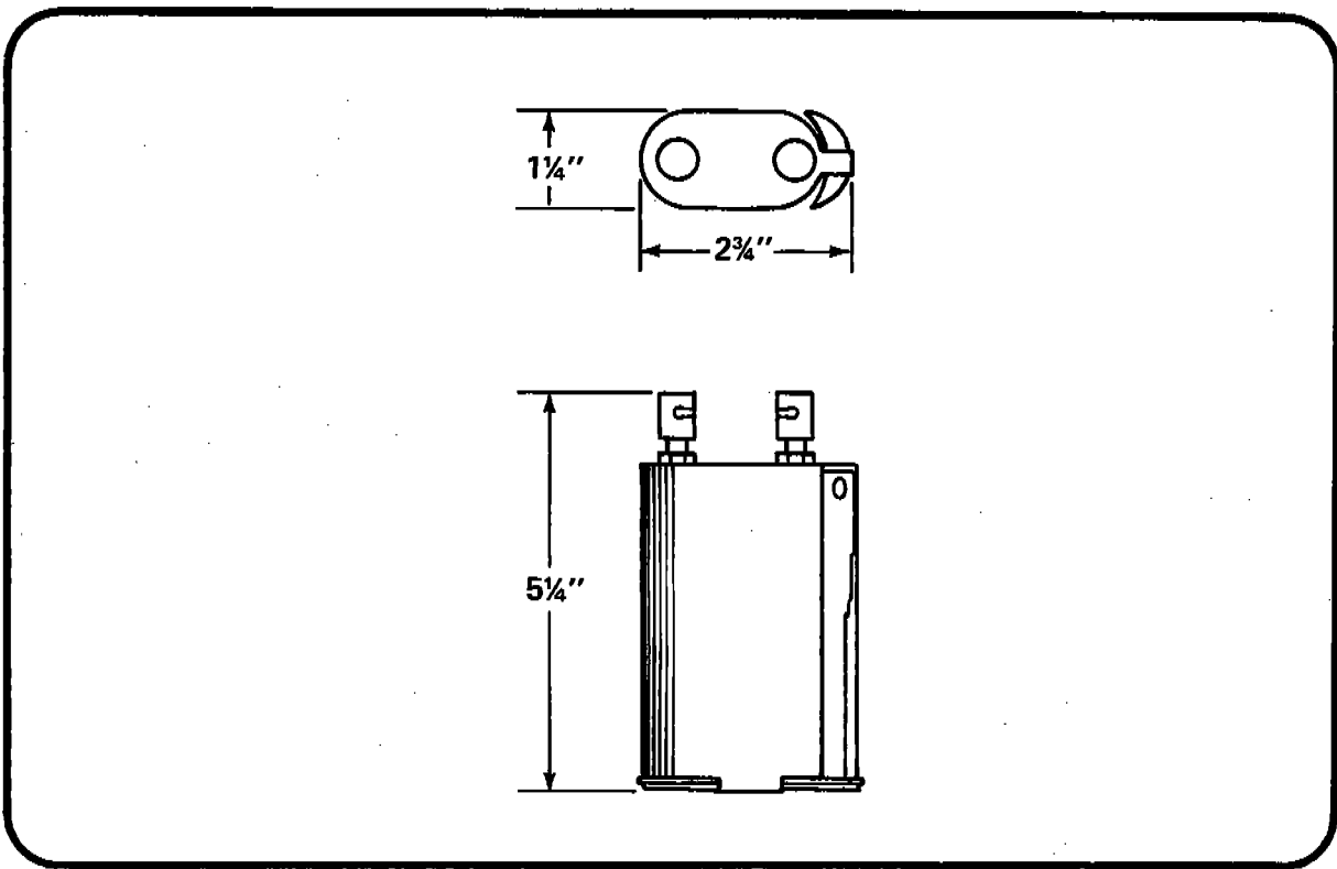
Figure 64 EXTERNAL DIMENSIONS OF THE MODEL 7107-7 AND MODEL 7107-4 MINIATURE BLASTING MACHINES. NOTE THAT THEY BOTH HAVE THE SAME DIMENSIONS. THEY ALSO WEIGH THE SAME: 12 OUNCES.
