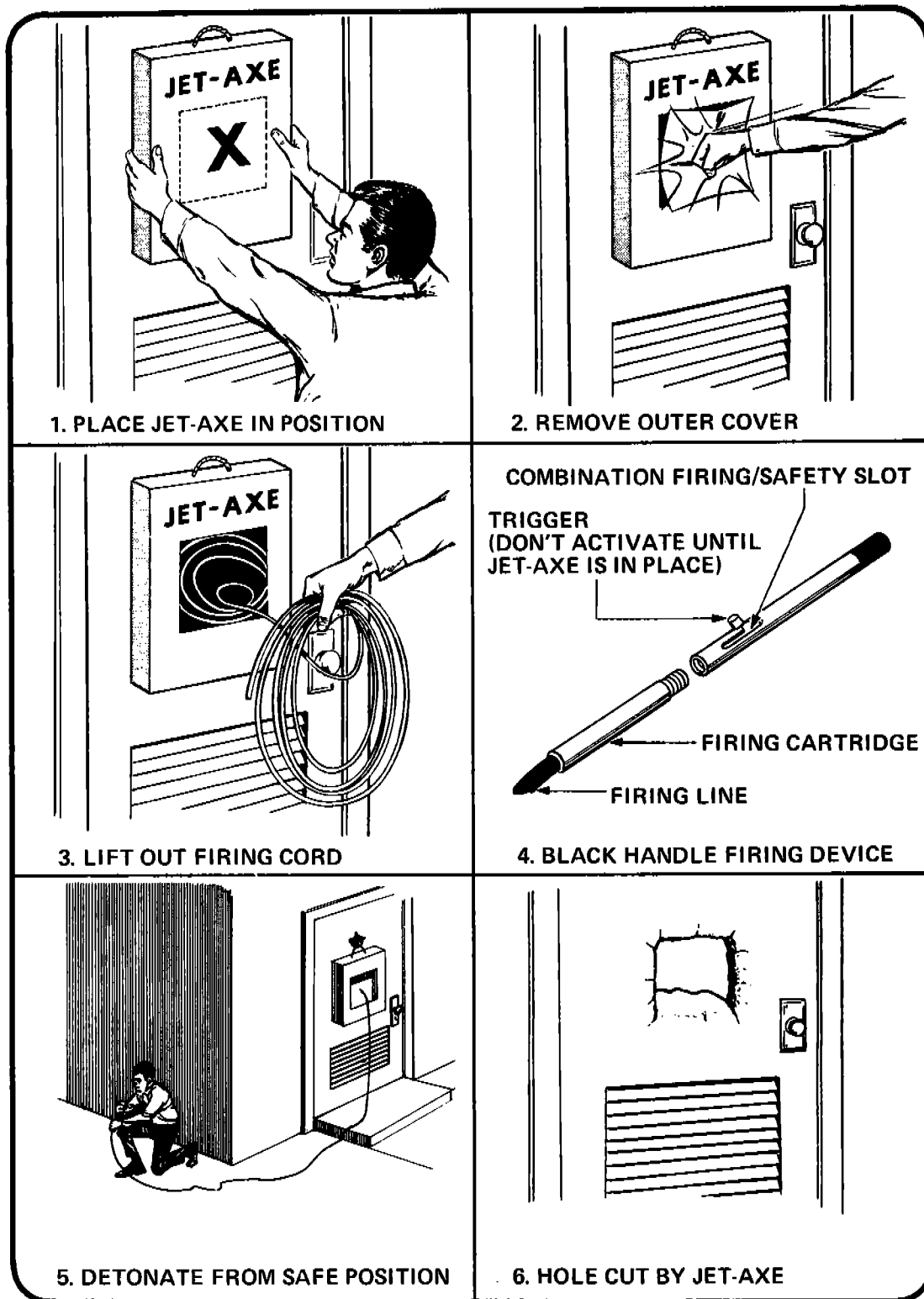
Figure 18 EMPLOYMENT OF JET-AXE
