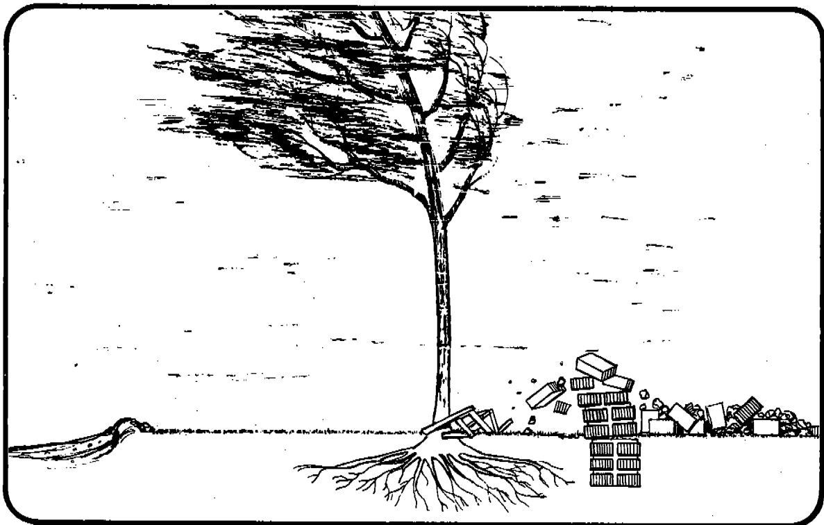
Figure 4 NEGATIVE PRESSURE PHASE OF AN EXPLOSION
