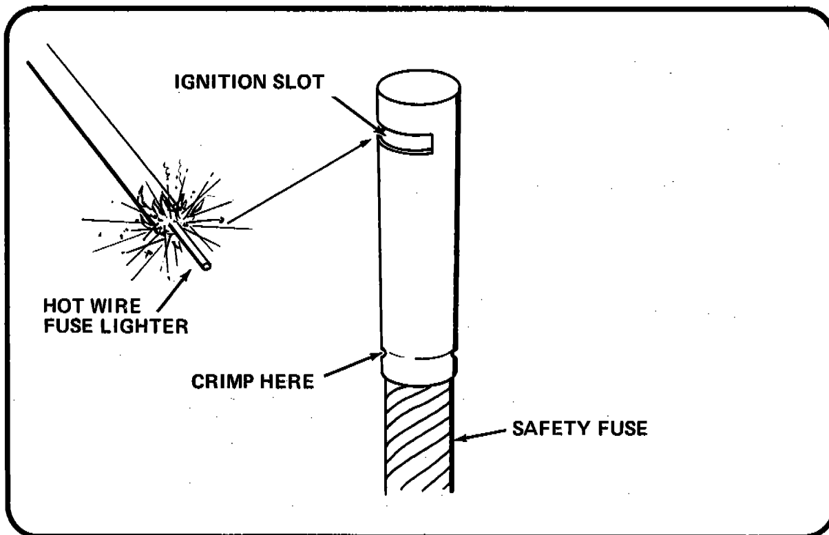
Figure 59 HOT WIRE FUSE LIGHTER AND FLAME TYPE FUSE LIGHTER
