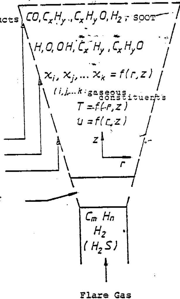
Fig. 6-1: Flare flame as a tubular reactor (schematic)
