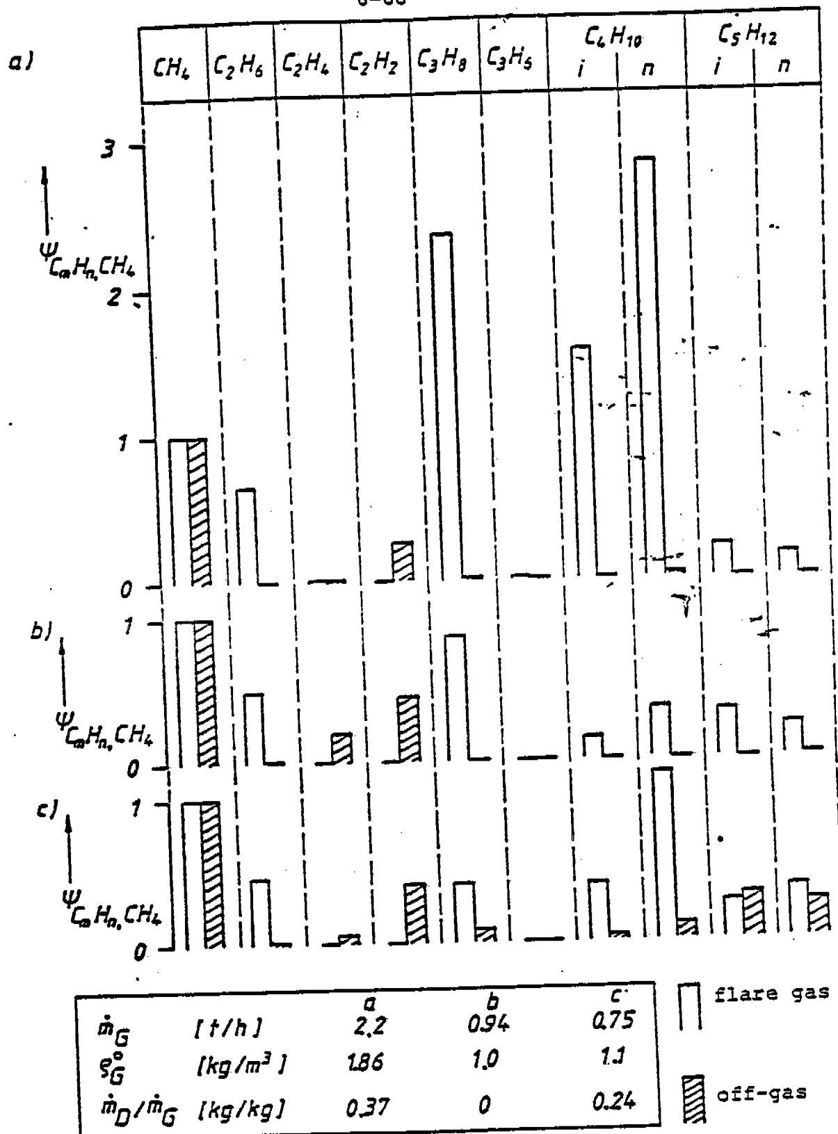
Fig. 6 - 22: Volume portion ratios of hydrocarbons in the flare gas and in the off-gas Test 2, 11, 12
