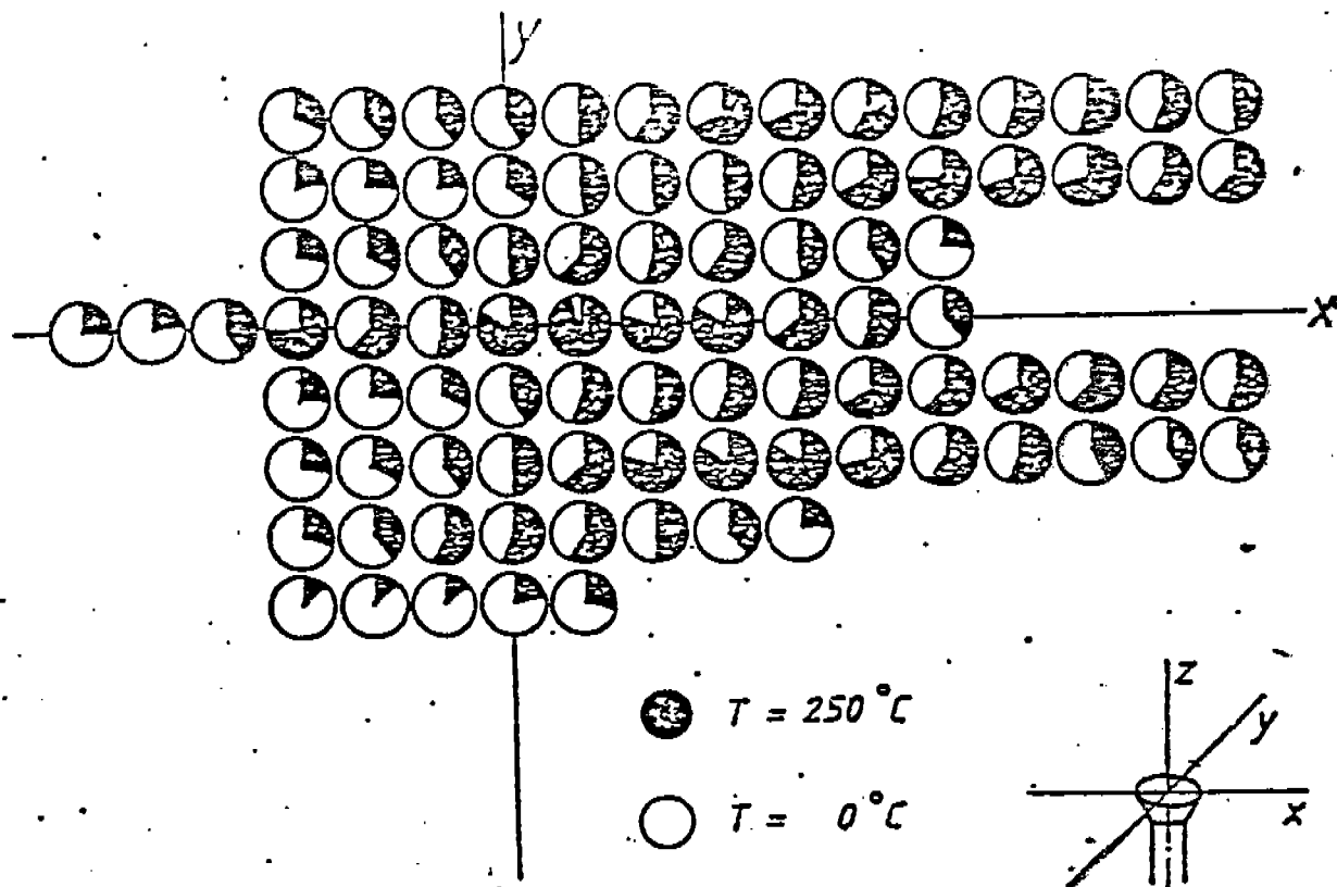
to Fig. 6-7: Distribution of the temperature in a horizontal plane above a flare flame burning in a cross draft. Test 06.010-.143
