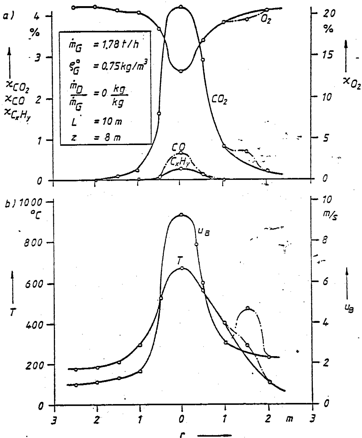
Fig. 6 - 2 : Distribution of the measured components in a secant of a flare flame burning in a calm atmosphere Test No. 13.011-.020
