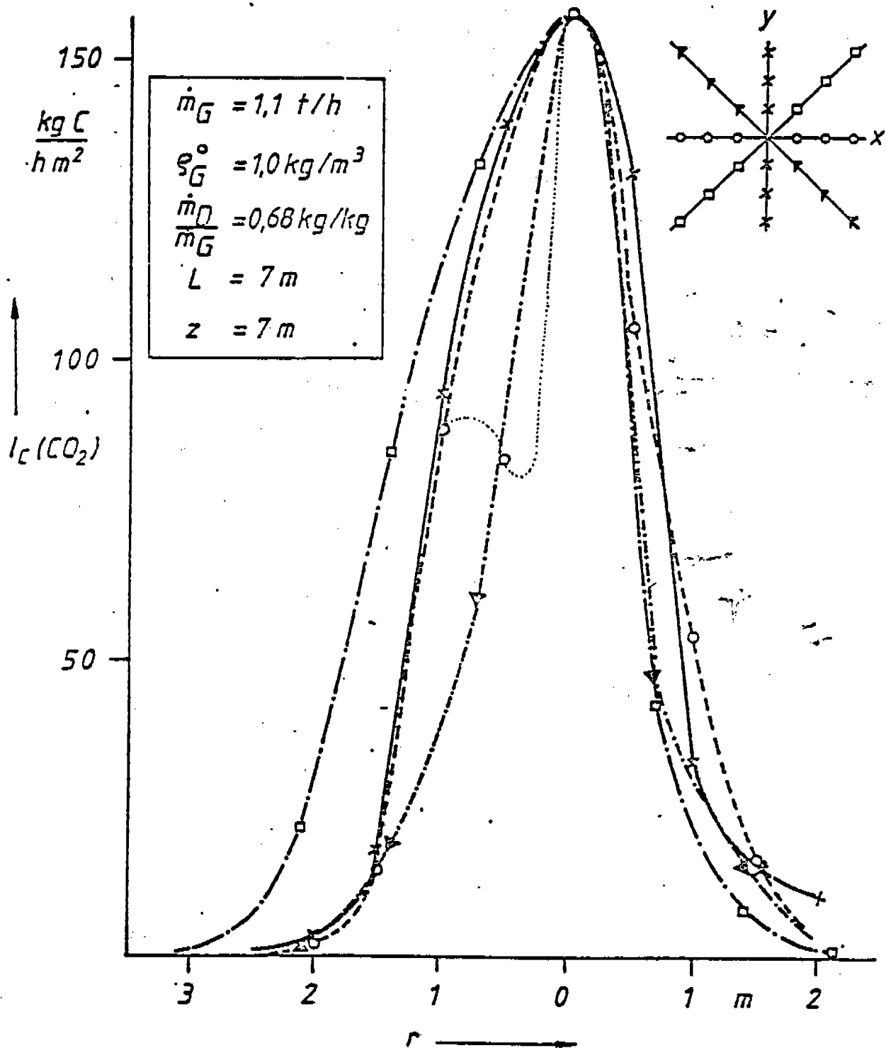
Fig. 6 - 3: Distribution of the mass flow density of the carbon bound as carbon dioxide in 4 diameters of a flare flame burning in a calm atmosphere Test 11.011-.035
