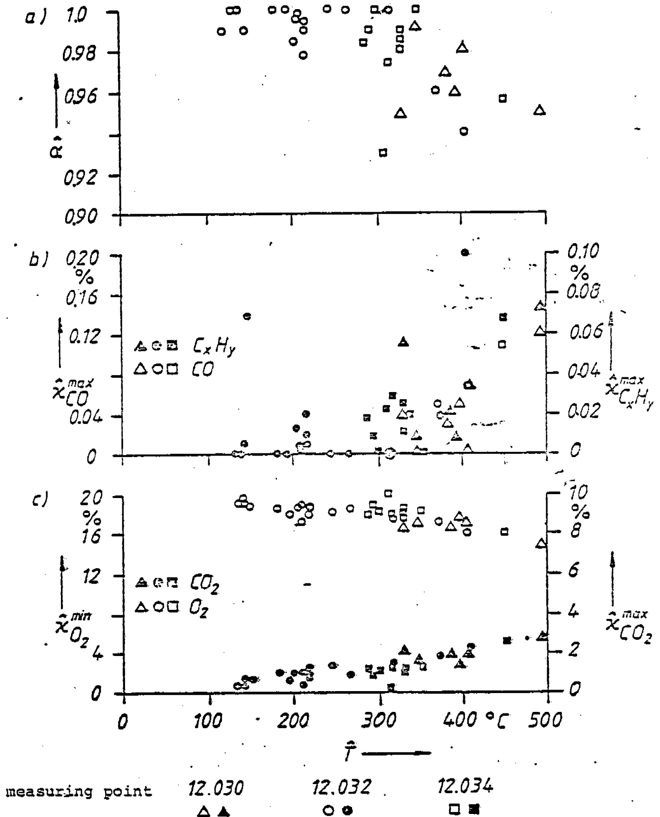
Fig. 6 - 12: Momentary values of measuring components and the local burnout degree in gusty wind calculated from these values Test 12.030-.034
