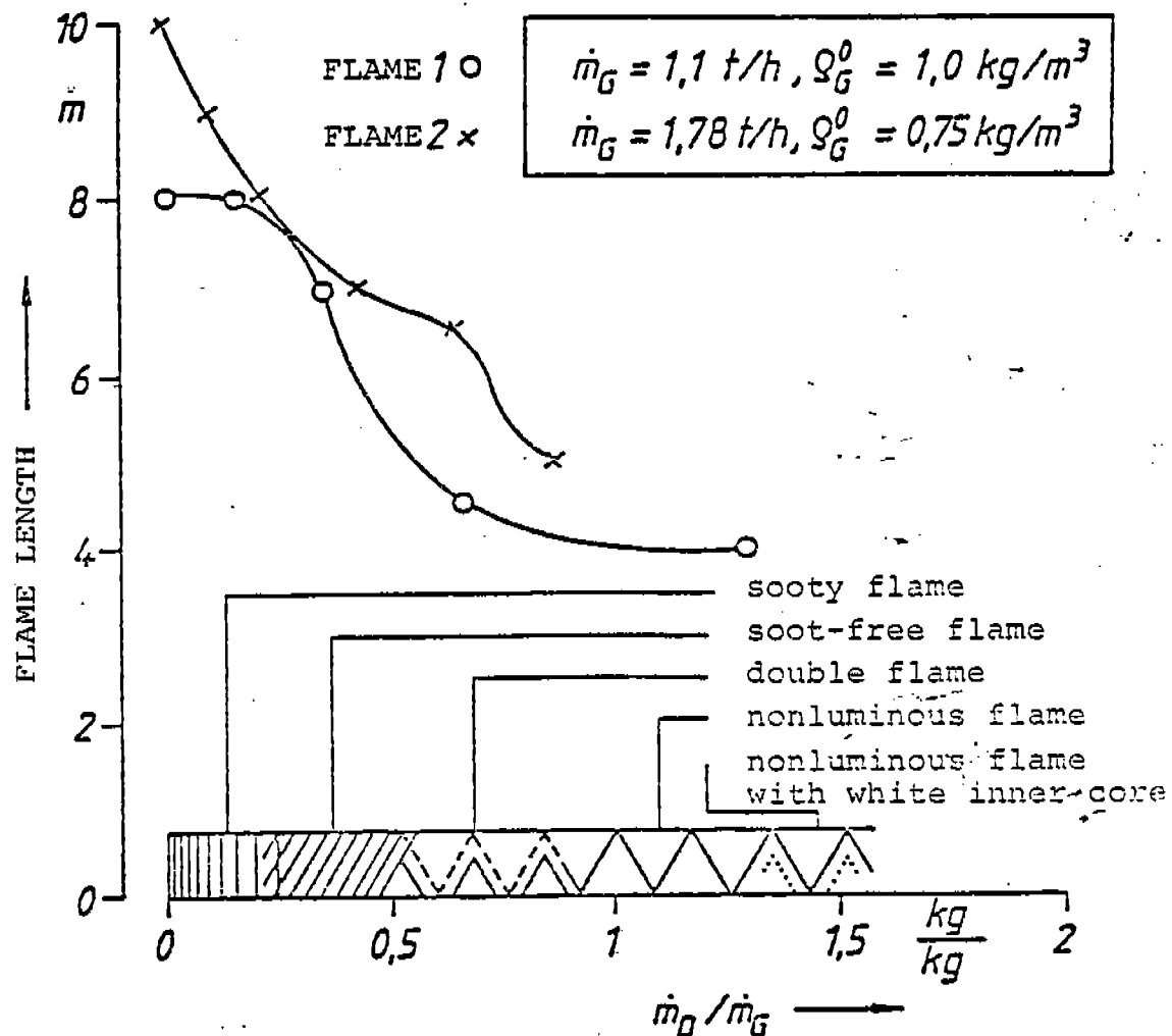
Fig. 6-13. Observed flame lengths as a function of the steam/gas ratio. Tests 11 and 13
