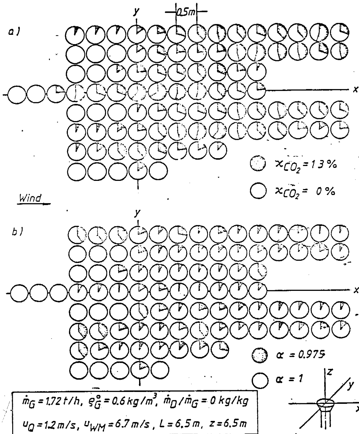
Fig. 6 - 7: Distribution of the volume portions of carbon dioxide and the local burnout degrees in a horizontal plane across a flare flame burning in a cross draft Test 06.101-.143
