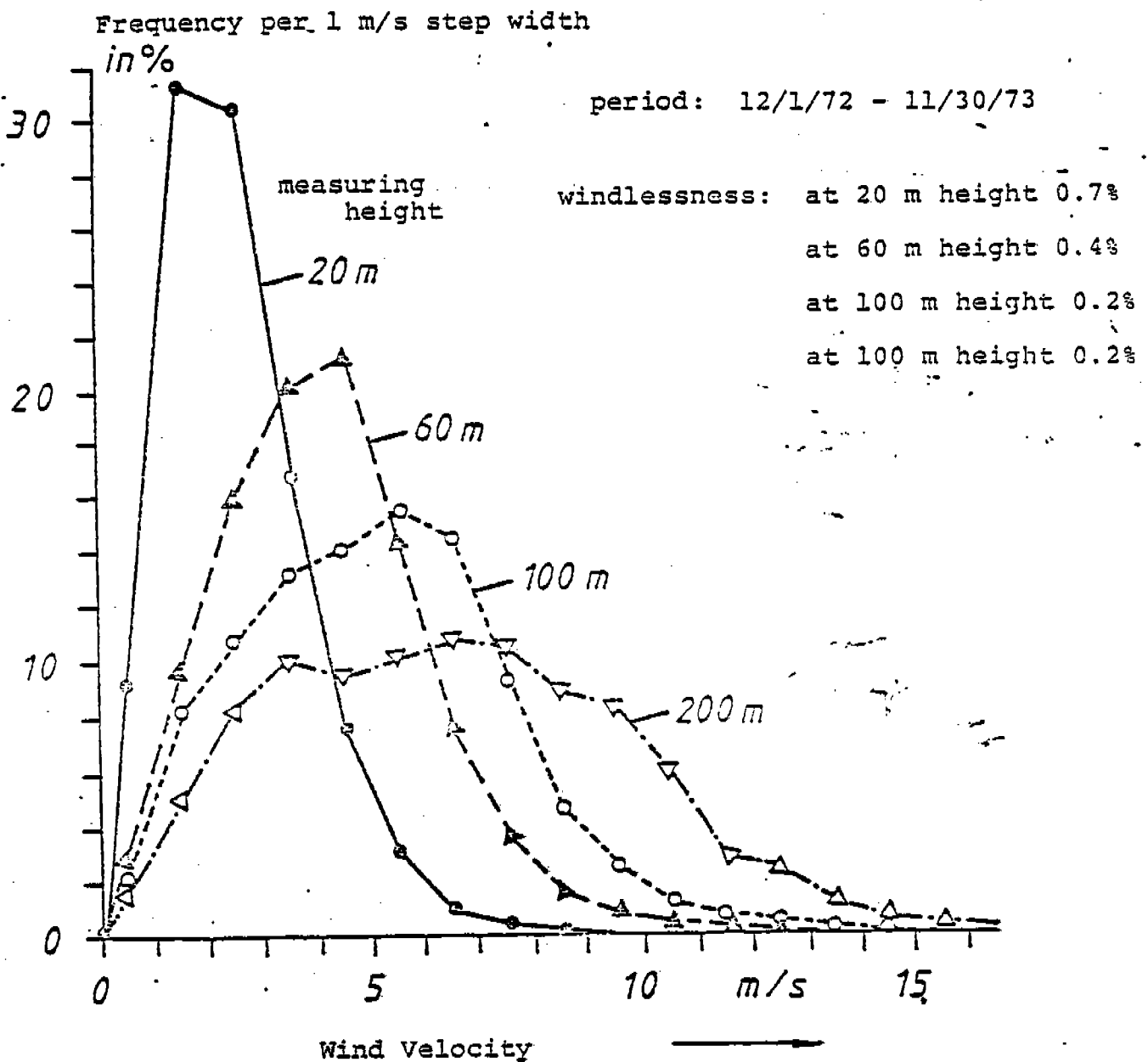
Fig. 6 - 5: Distribution of wind velocity at different heights [80]
