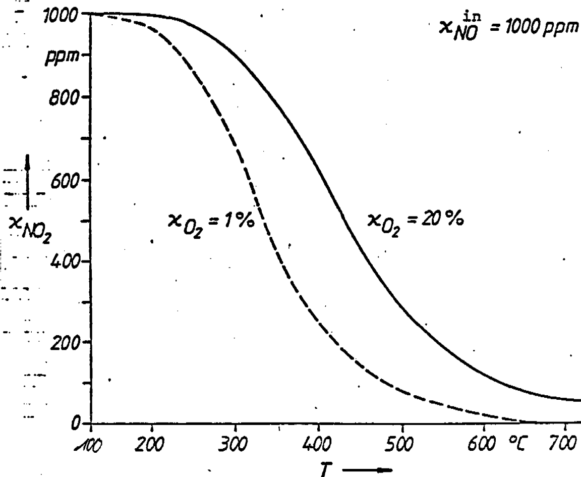
Fig. 4-4 : Equilibrium concentration of nitrogen dioxide as a function of the temperature for a nitrogen monoxide volume portion of 0.1% in mixture with oxygen volume portions of 20 and 1%, resp.
