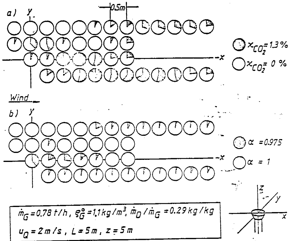
Fig. 6 - 8: Distribution of the volume portions of carbon dioxide and the local burnout degree in a horizontal plane across a flare flame burning in a cross draft
