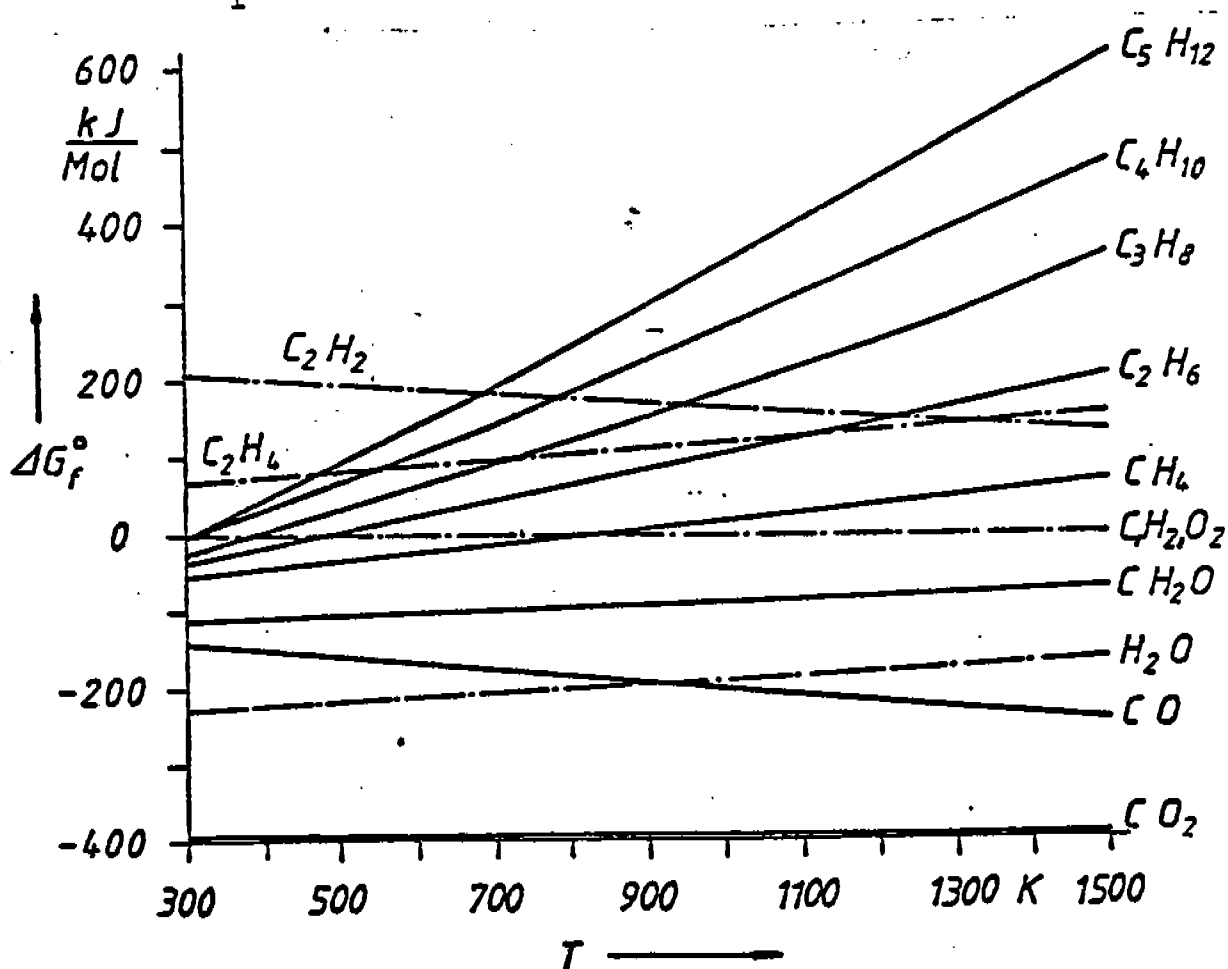
Fig. 4-2 : Standard free enthalpy of formation as a function of the temperature.
