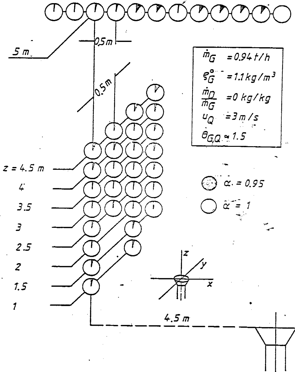
Fig. 6 -10: Distribution of the local burnout degrees in a vertical plane at the end of a flare flame burning in a cross draft Test 08.001-.047
