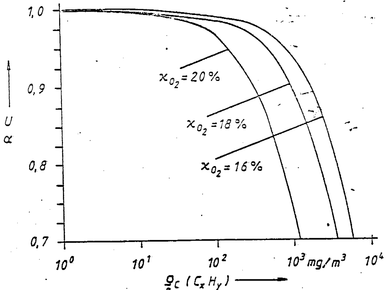
Fig. 6 - 6: Degree of conversion and local degree of burnout as a function of the mass concentration of organically bound carbon with different oxygen volume portions
