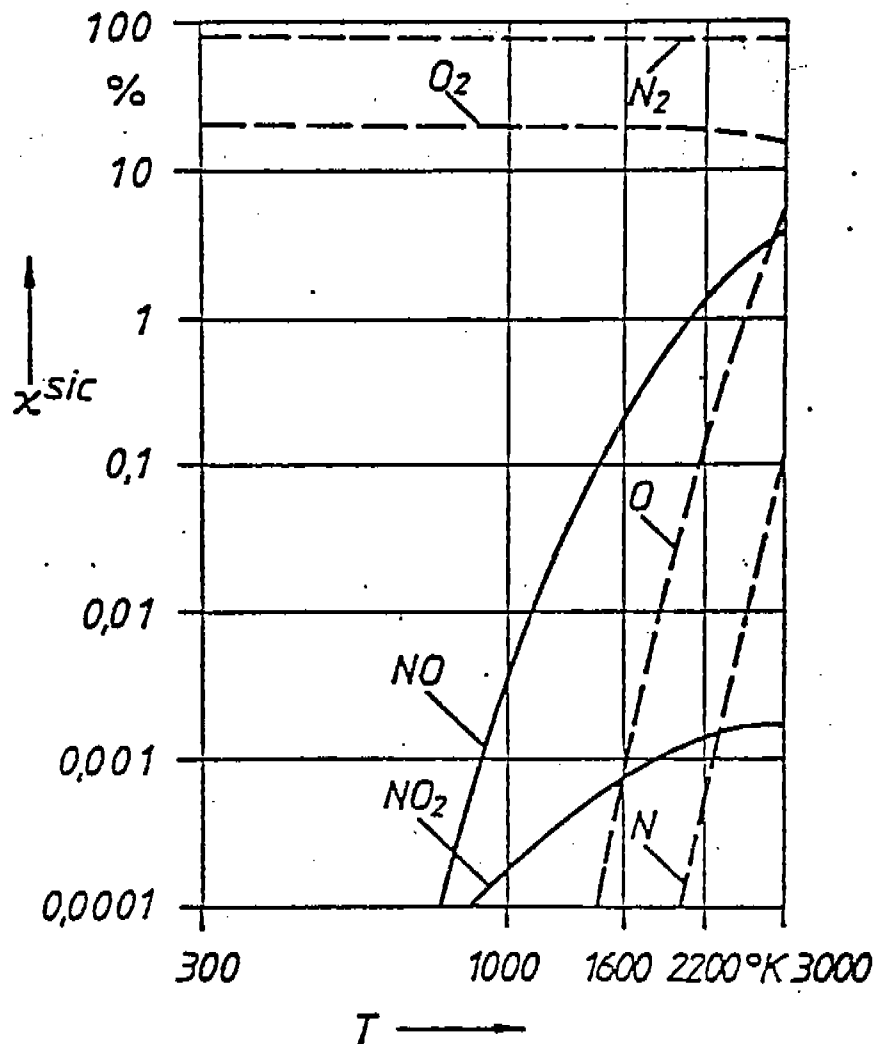
Fig. 6 - 25: Volume portions of nitrogen oxides at chemical equilibrium [99]
