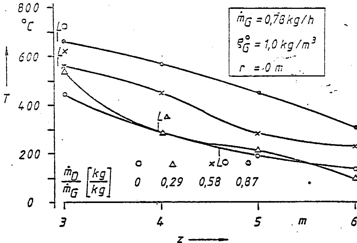
Fig. 6-16. Temperature downstream (and upstream) of the end of flame L as a function of the steam/gas ratio. Test 08.133-.151
