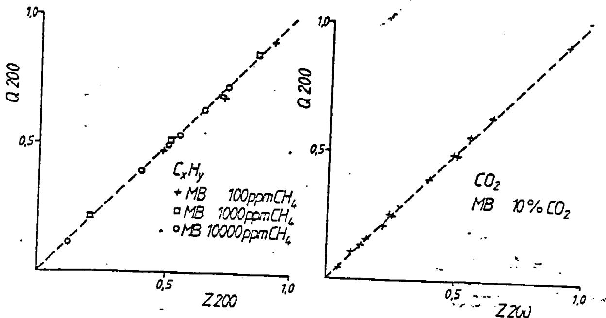
Fig. 5-7. Comparison of the test values of the gas analyzers for carbon dioxide and organically bound carbon with the measuring object being introduced at the sampling orifice and at the sampling gas distributor.
