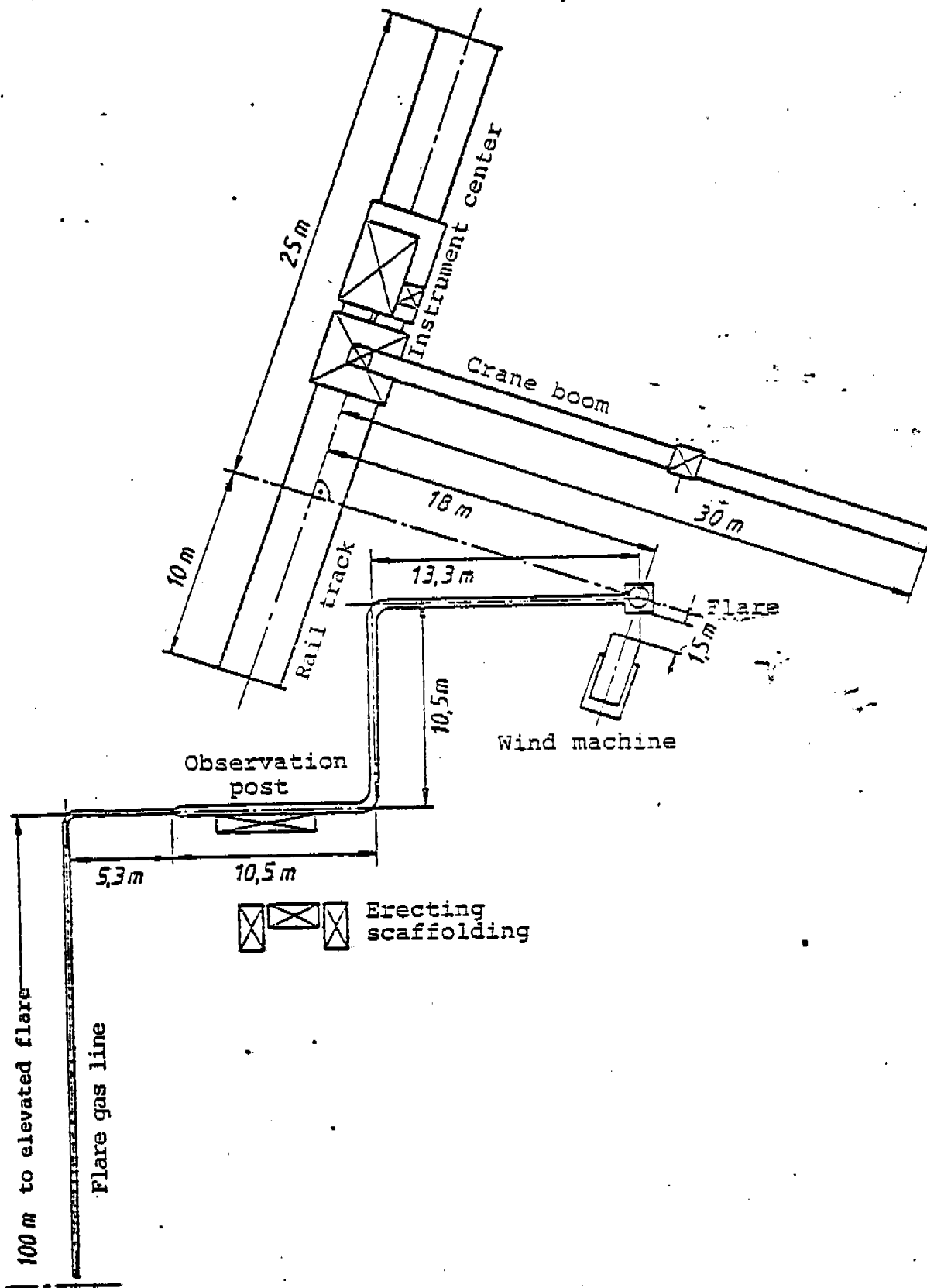
Fig. 5-2. Layout map of the testing arrangement
