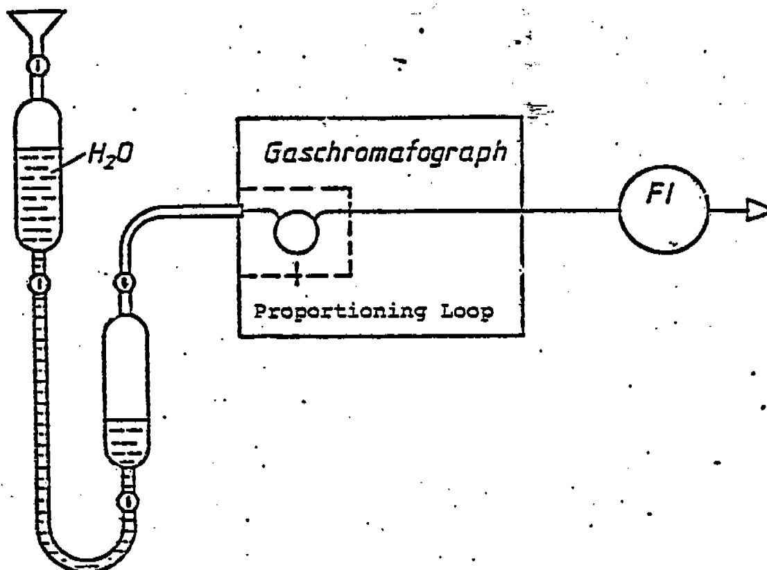
Fig. A.7-1: Flow diagram for introducing the sample in the gas-chromatographic analysis
