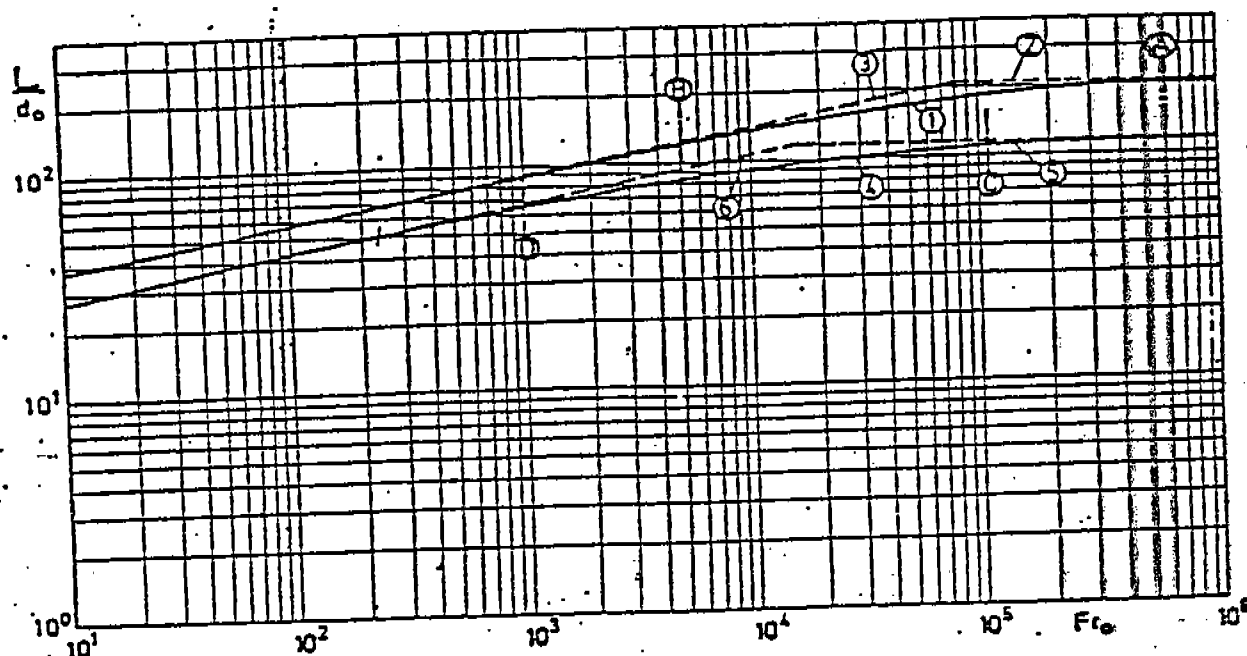
Fig. 7-8. Flame length for city-gas and natural gas, with allowance made for segregation.
