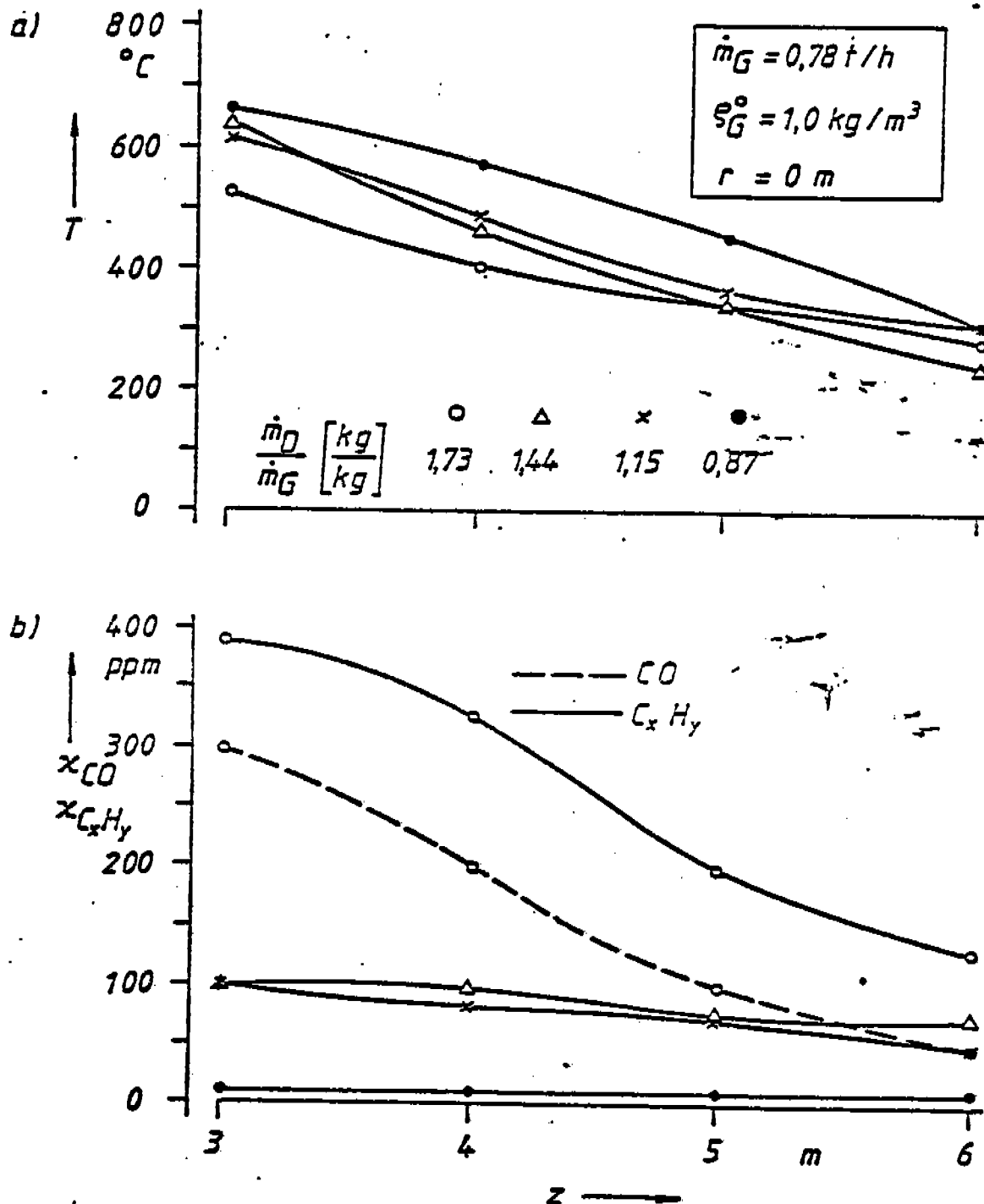
Fig. 6-19. Effect of large steam additions on the temperature and on the volume portions of organically bound carbon and carbon monoxide downstream of the end of the flame. Test 08.148-.166
