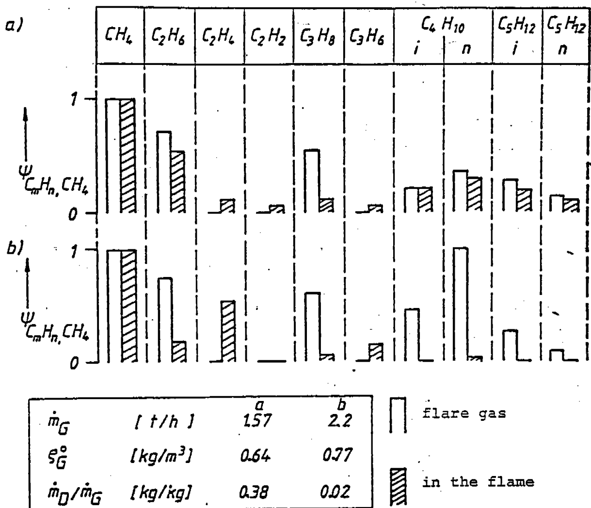
Fig. 6 - 23: Volume portion ratios of hydrocarbons in the flare gas and in the flame Test 16, 17
