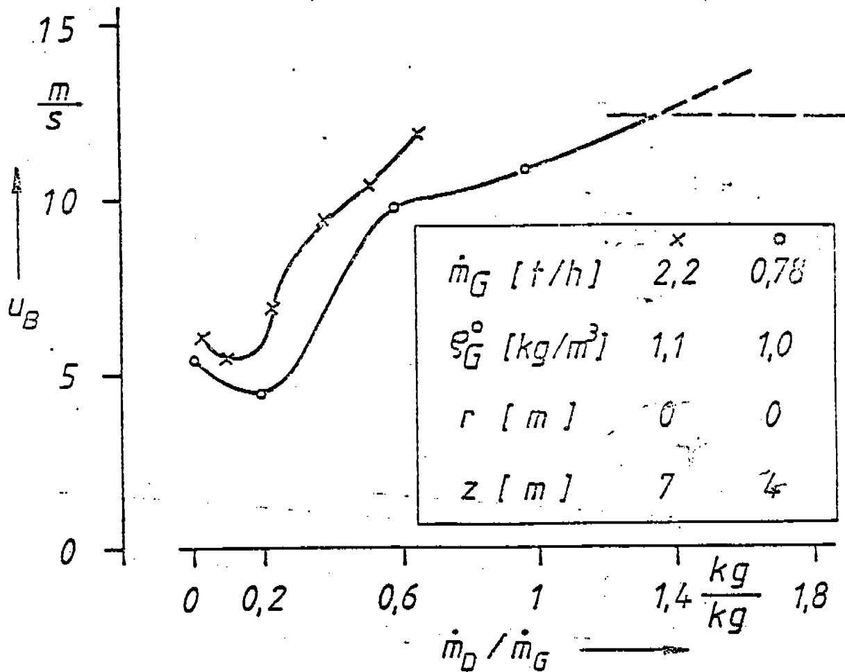
Fig. 6-15. Effect of steam/gas ratio on off-gas velocity. Tests 08.127-.132 and 08.167-.172
