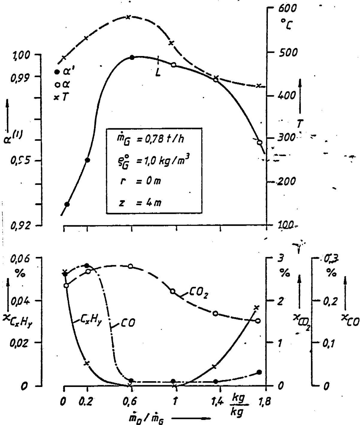
Fig. 6-18. Effect of large steam/gas ratios a) on the local burnout degree and the temperature b) on the volume portions of organically bound carbon, carbon monoxide and carbon dioxide Test 08.167-.172
