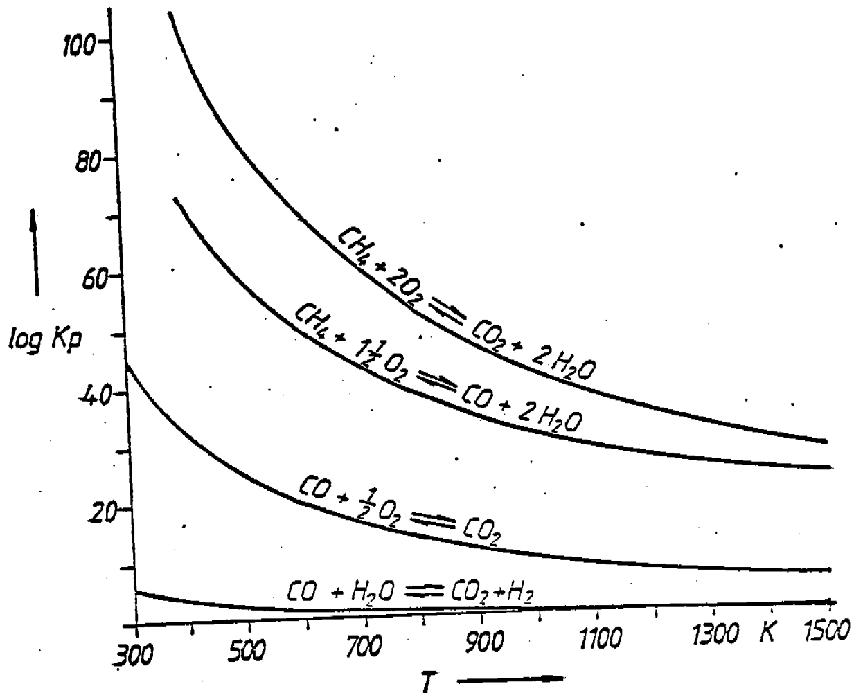
Fig. 4-3 : Equilibrium constants as a function of the temperature.
