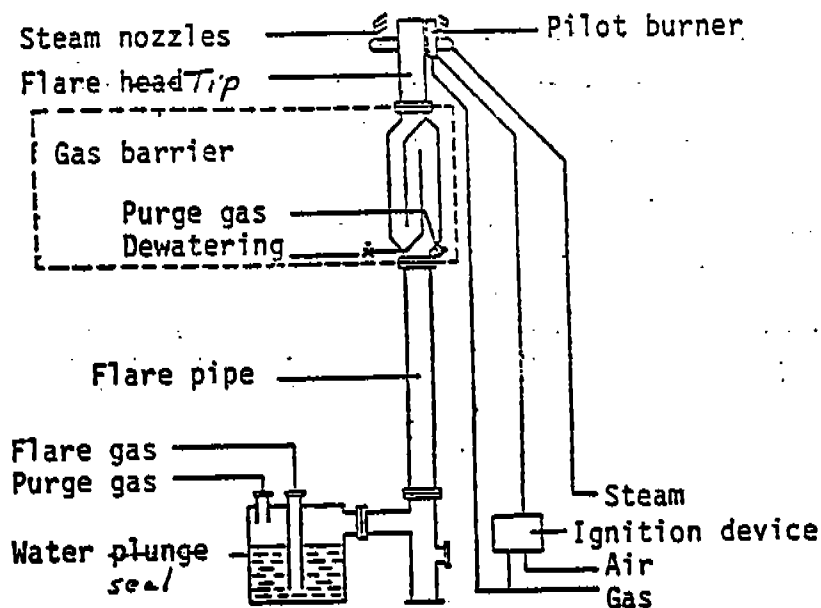
Fig. 1-1 High-Flare System (schematically) Elevated
