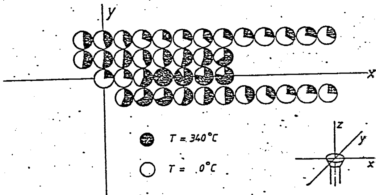
to Fig. 6-8: Distribution of the temperature in a horizontal plane above a flare flame burning in a cross draft. Test 03.001-.039
