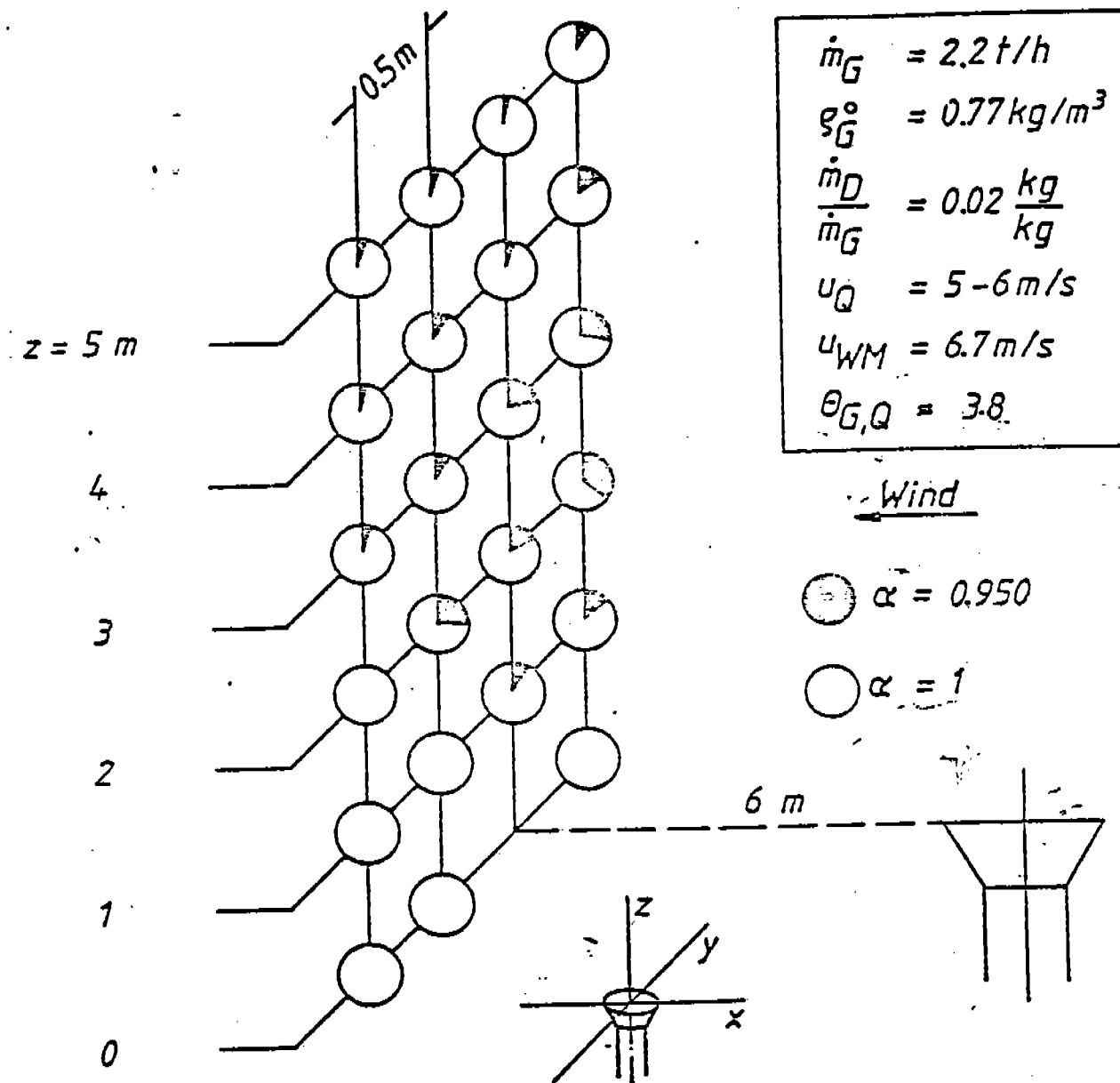
Fig. 6 - 9: Distribution of the local burnout degrees in a vertical plane at the end of a flare flame burning in a strong cross wind Test 16.001-.027
