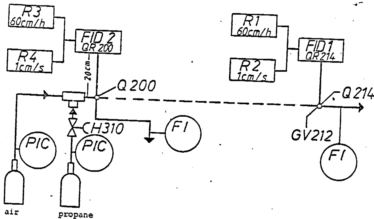
Fig. 5-8. Flow diagram for the testing arrangement for determining the behavior in time of the sample gas line.
