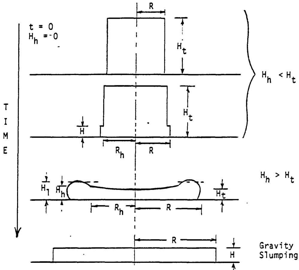
Figure V.2. Schematic Diagram of a Radially Spreading Cloud.
