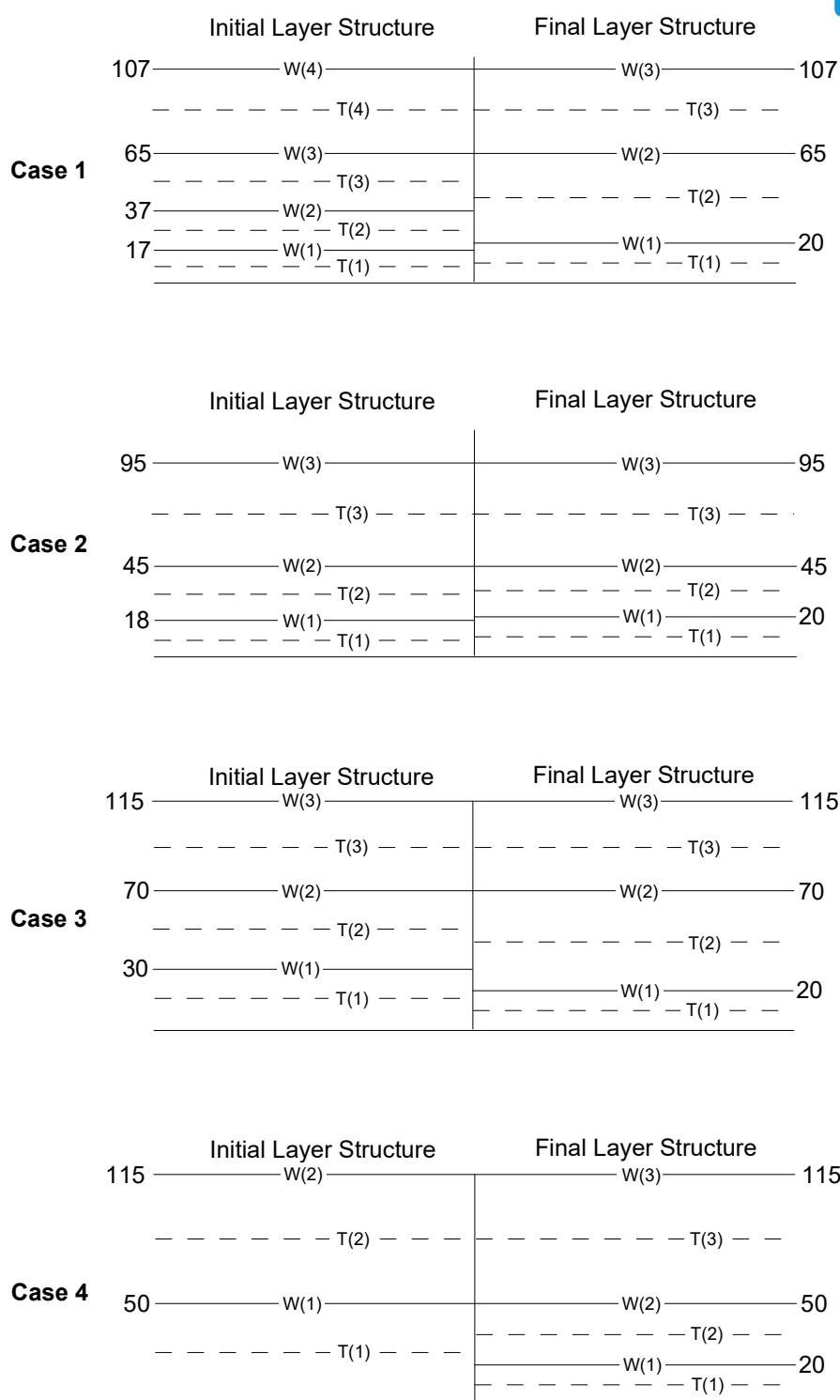
Figure 2-4. Schematic examples of the approach to introduce a 20-m deep first layer for CALPUFF. The four cases are described in the text: [1] ZFACE(1) < 19 m, ZFACE(2) < 39 m; [2] ZFACE(1) < 19 m, ZFACE(2) \geq 39 m; [3] 19 \text{ m} \leq ZFACE(1) < 39 m; and [4] ZFACE(1) \geq 39 m. Locations of vertical velocity (W) and temperature (T) are shown in each case.
