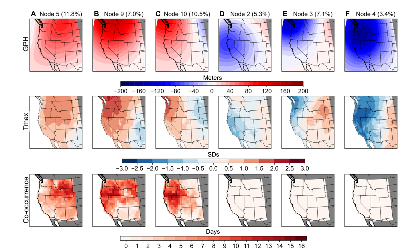
Fig. 3. The six SOM nodes with the largest [(A) to (C)] and smallest [(D) to (F)] PM 2.5 /ozone co-occurrence risk. Top: Geopotential height (GPH) anomalies for each SOM node trained over 1979 to 2020. Middle: Composite standardized anomalies of daily maximum temperatures ( T_{max} ) on all days associated with each node during the 2001 to 2020 period. Bottom: Number of times each grid cell experienced local PM 2.5 /ozone co-occurrences during all widespread co-occurrence days associated with that node. The maximum possible number of co-occurrence days in a given grid cell is equivalent to the total number of widespread co-occurrence days associated with that node (node 5, 14 days; node 9, 16 days; node 10, 13 days; Table 1). Values in parentheses on top row indicate the frequency of each SOM node relative to all July to September days during the period of overlap with air pollution data (2001 to 2020).
