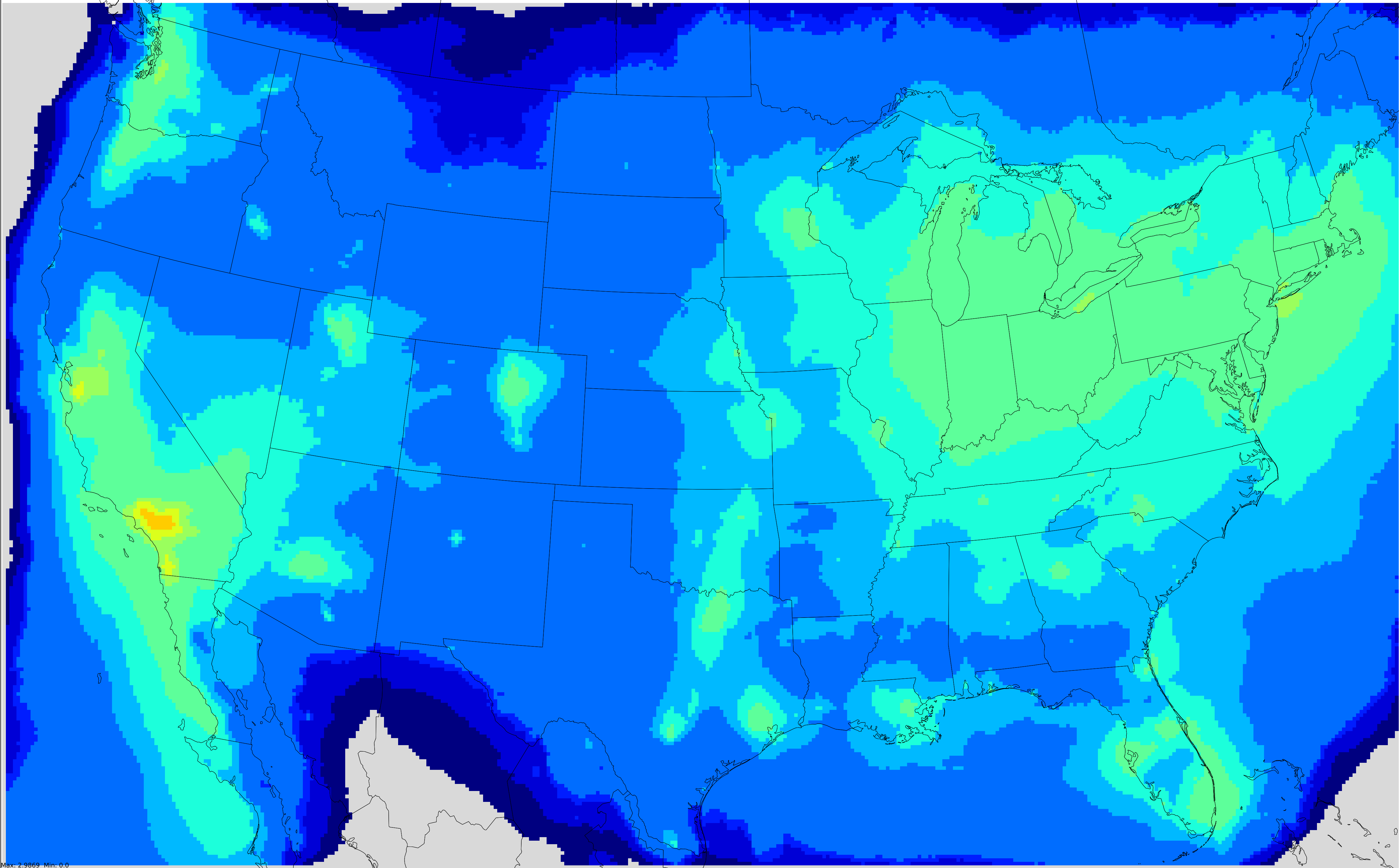
Projected 8-h max Average Seasonal Ozone concentration(ppb) from VOC in 2025 Onroad Light Duty
