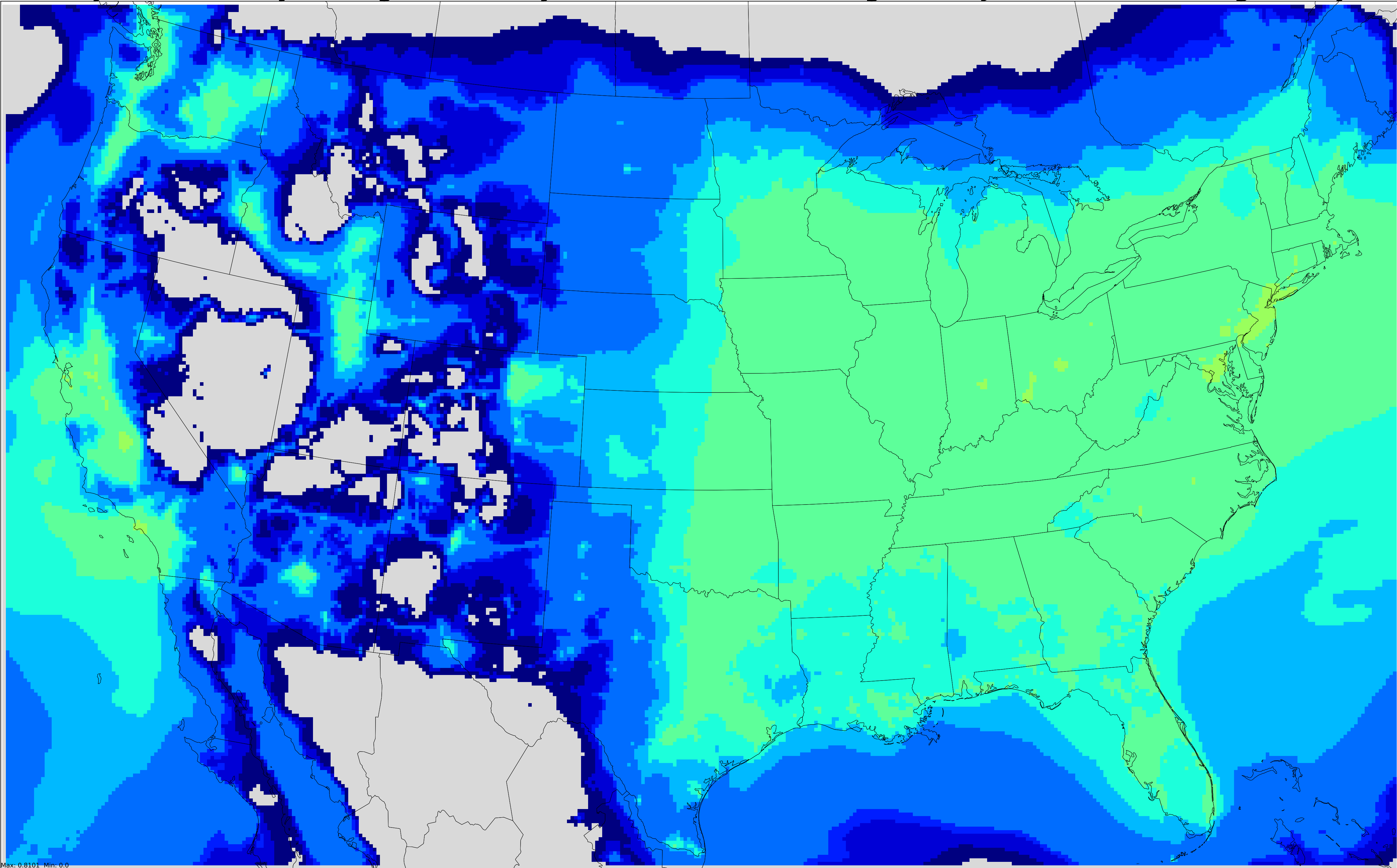
Projected Monthly Average secondary PM2.5 concentration(ug/m3) in Jan 2025 Onroad Light Duty
