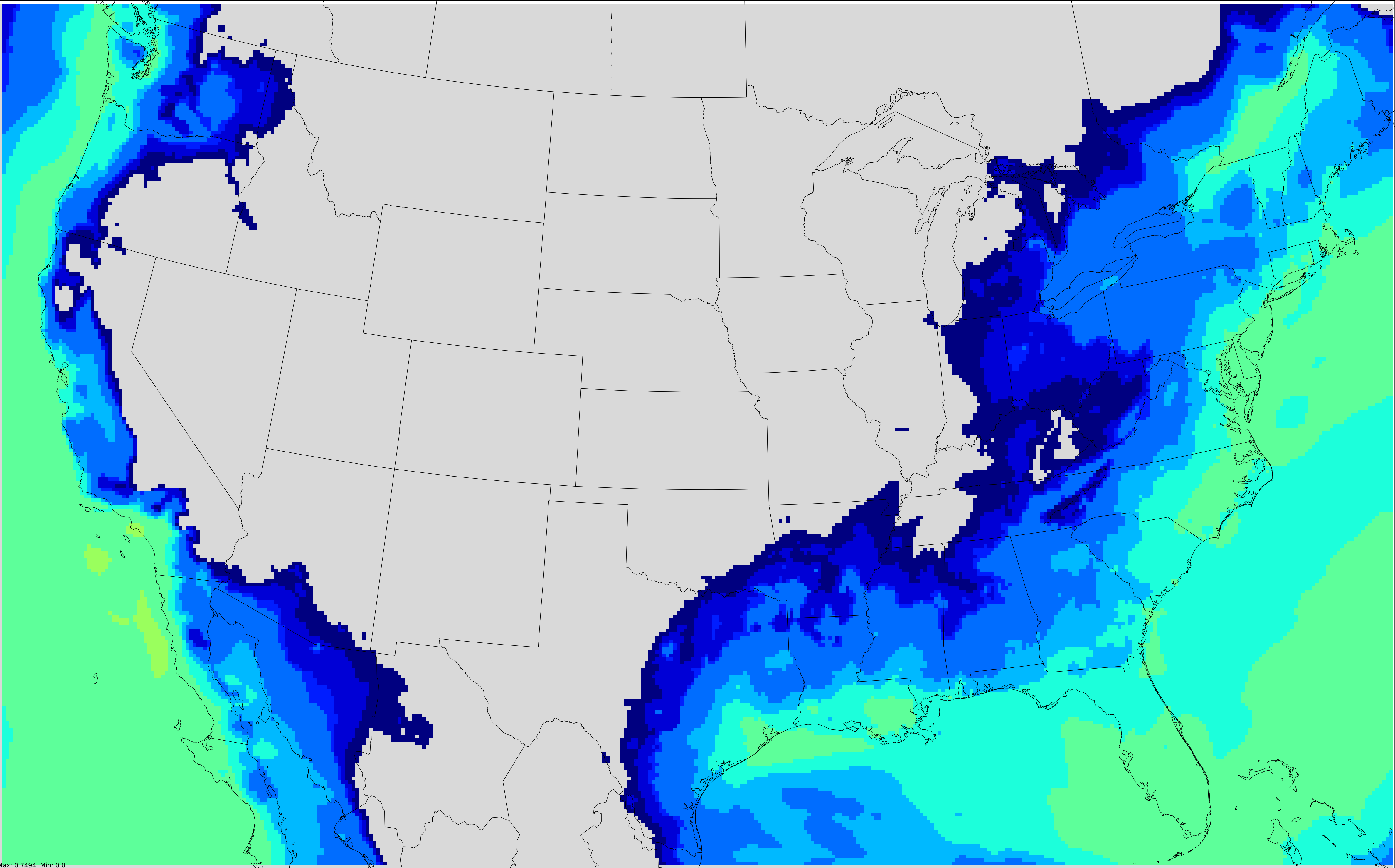
Projected Monthly Average Secondary PM2.5 concentration(ug/m3) in Jan 2025 C3 marine
