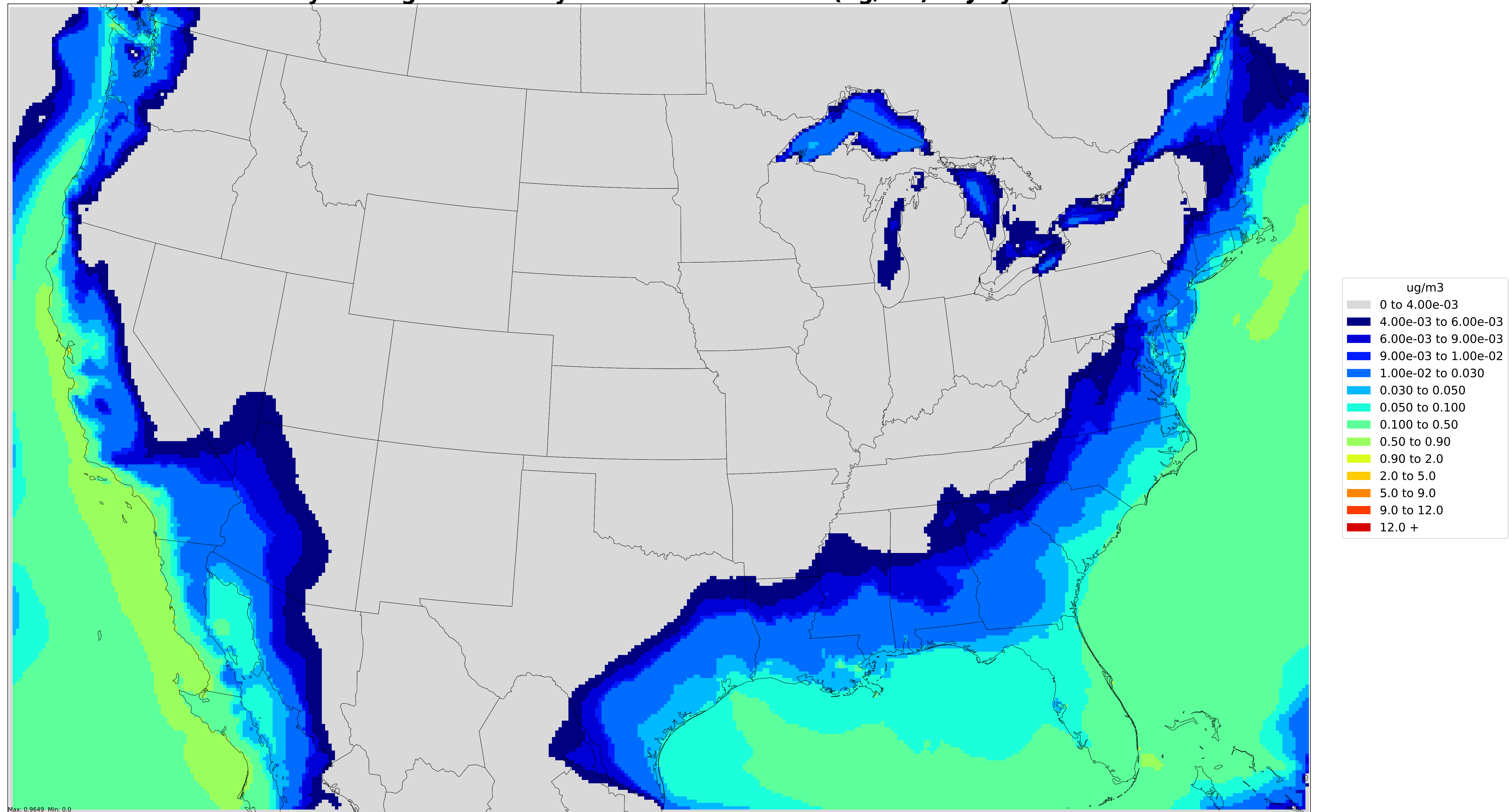
Projected Monthly Average Secondary PM2.5 concentration(ug/m3) in July 2025 C3 marine
