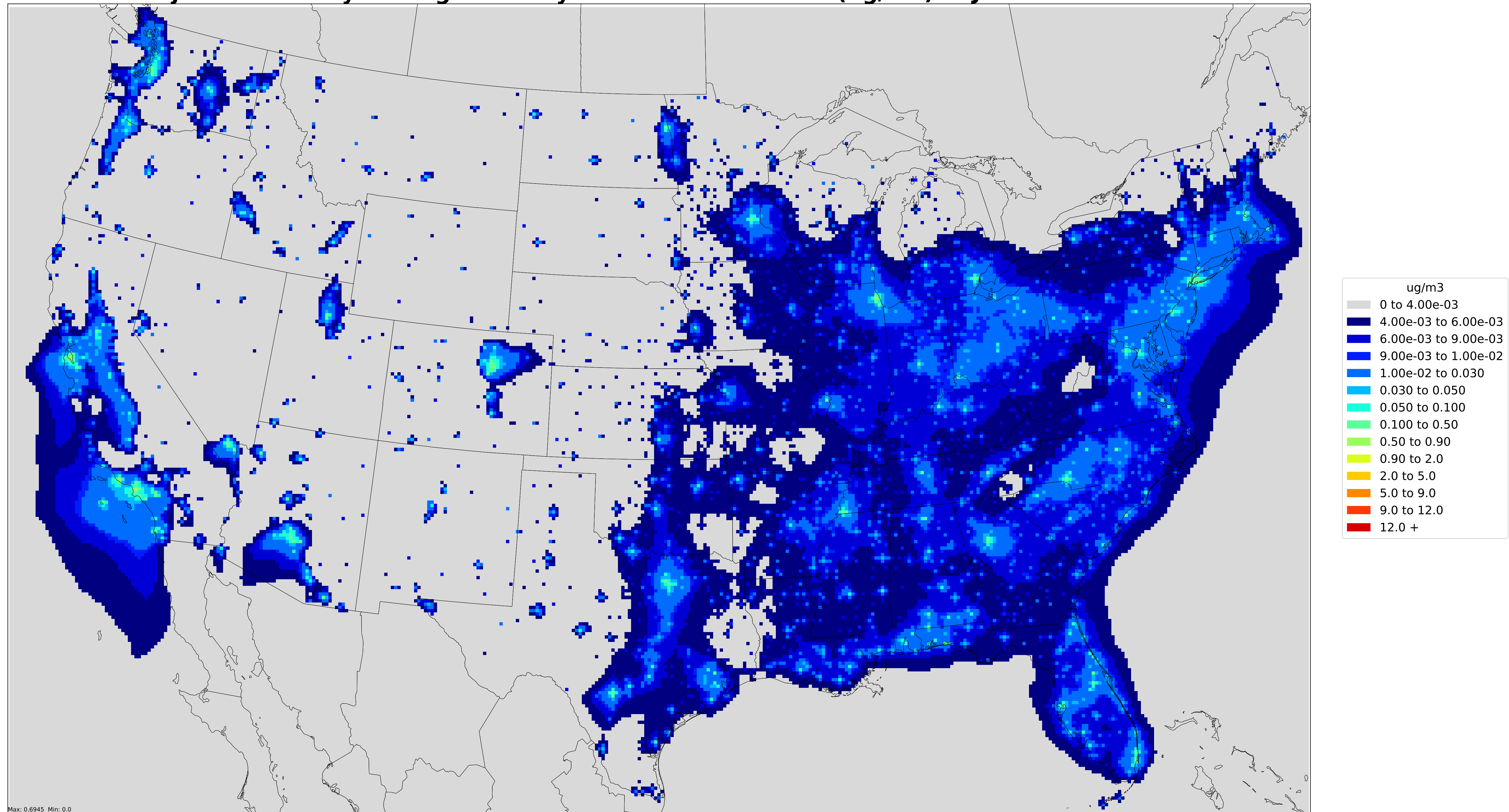
Projected Monthly Average Primary PM2.5 Concentration(ug/m3) in Jan 2025 Aircraft
