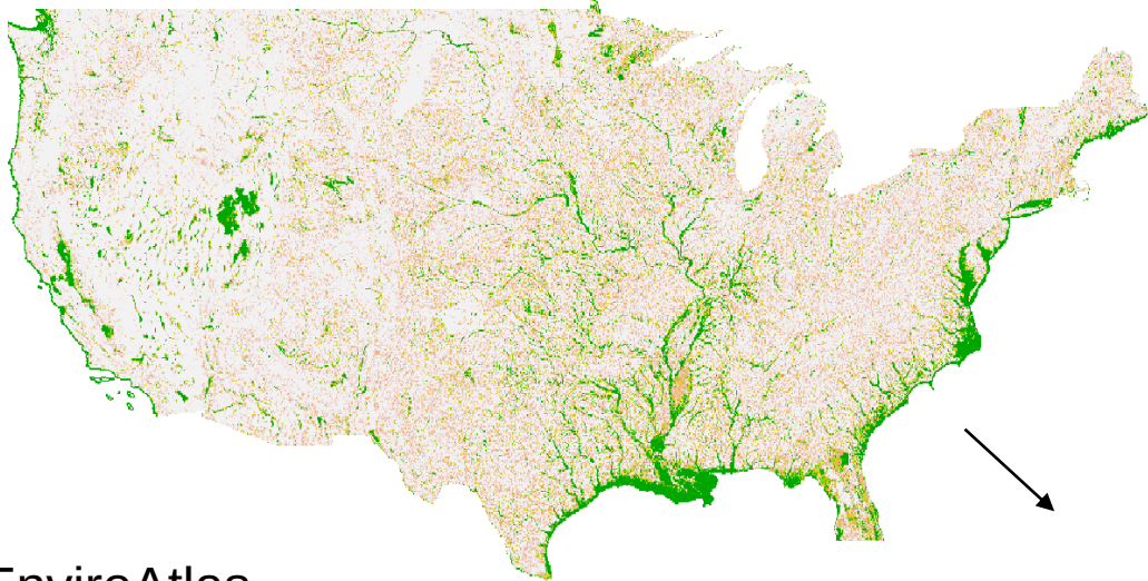
Floodplain
