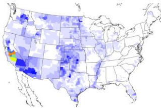
Emissions
