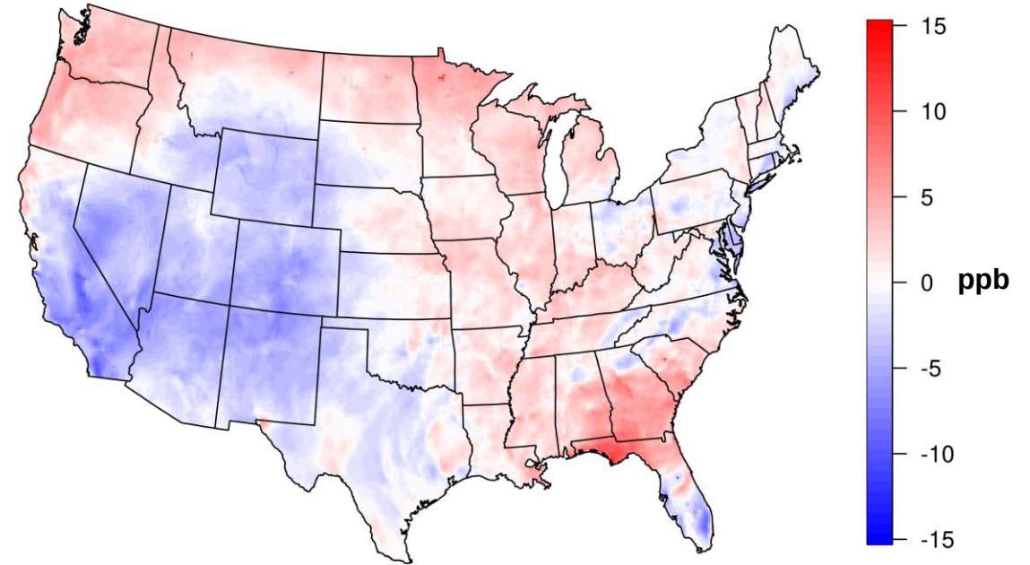
Monthly Mean MDA8 Difference (2015-2016): July
