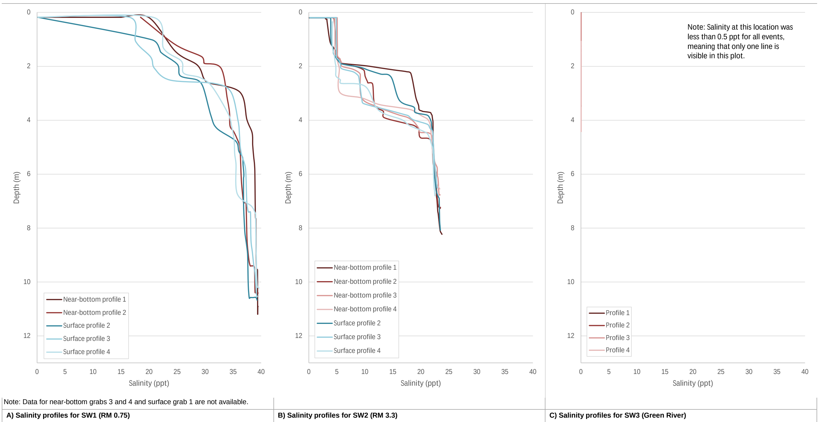
Figure C-5. Salinity profiles for storm 2 (ST2)
