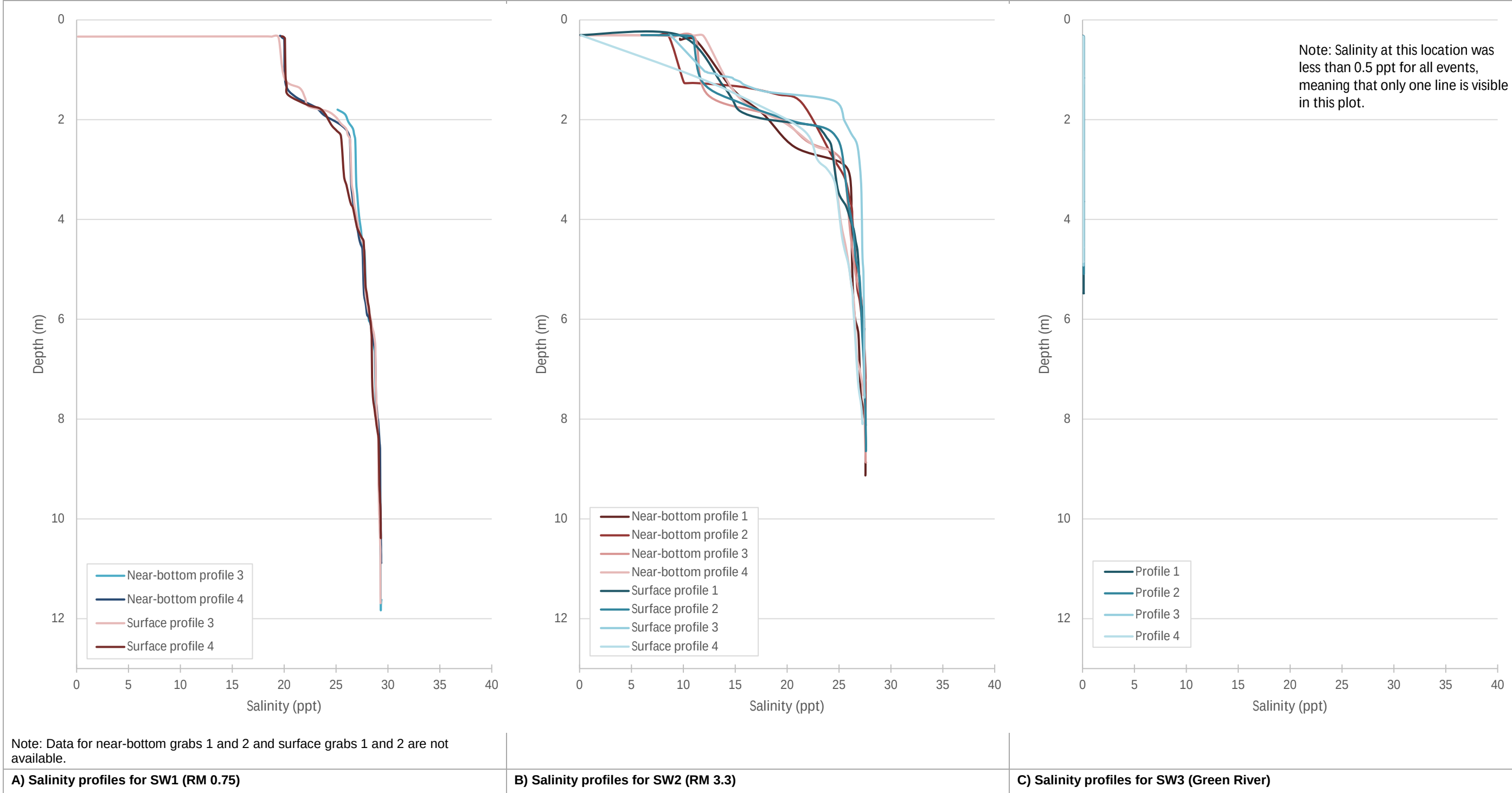
Figure C-3. Salinity profiles for dry baseflow event 2 (DB2)
