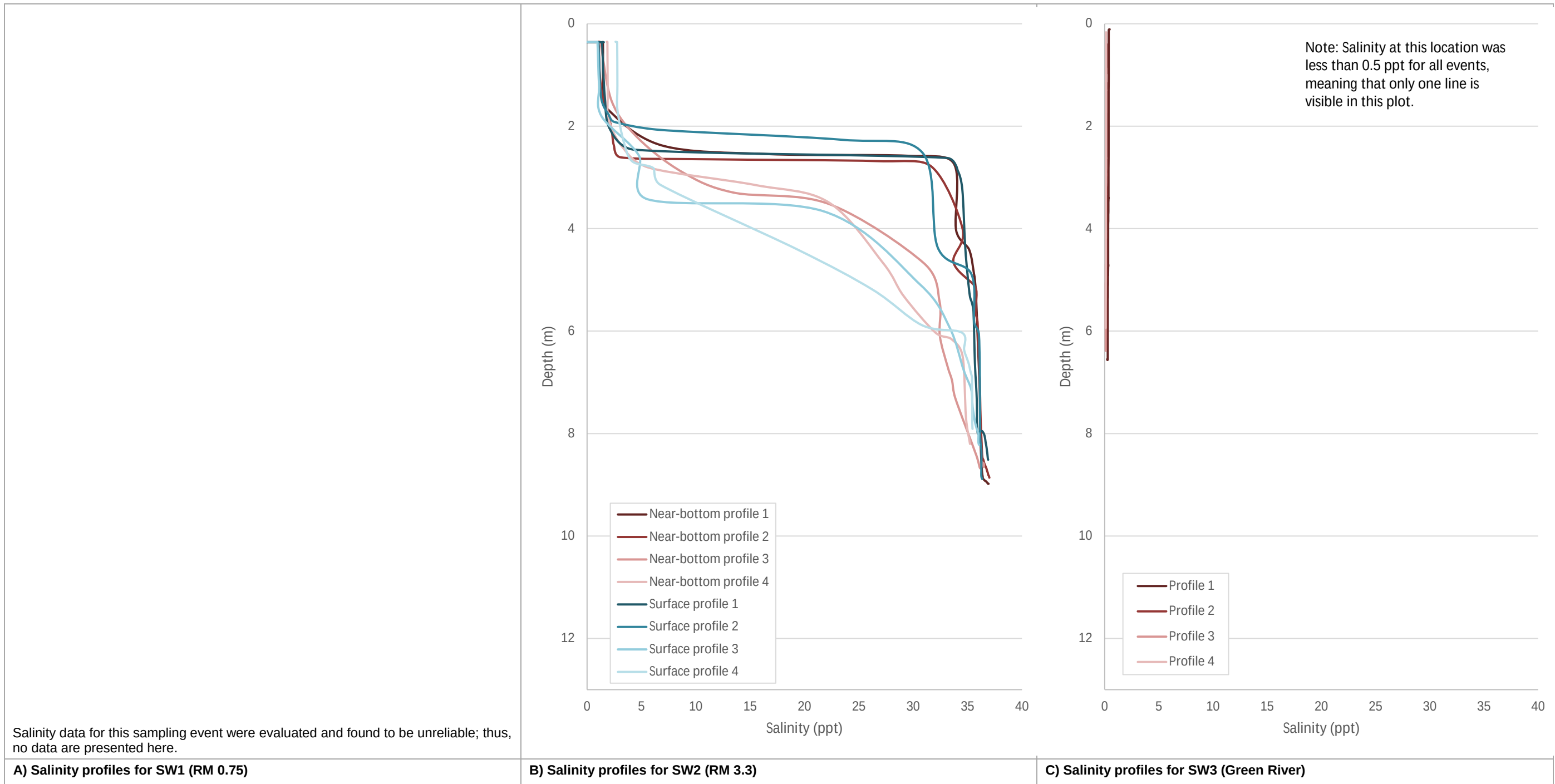
Figure C-8. Salinity profiles for wet baseflow 2 (WB2)
