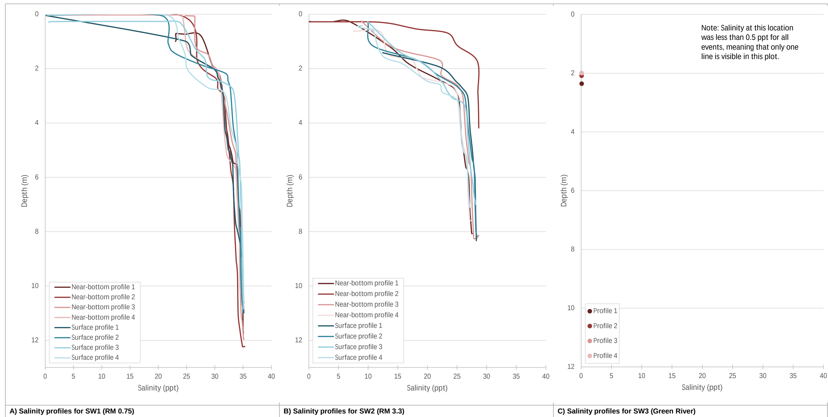
Figure C-2. Salinity profiles for dry baseflow event 1 (DB1)
