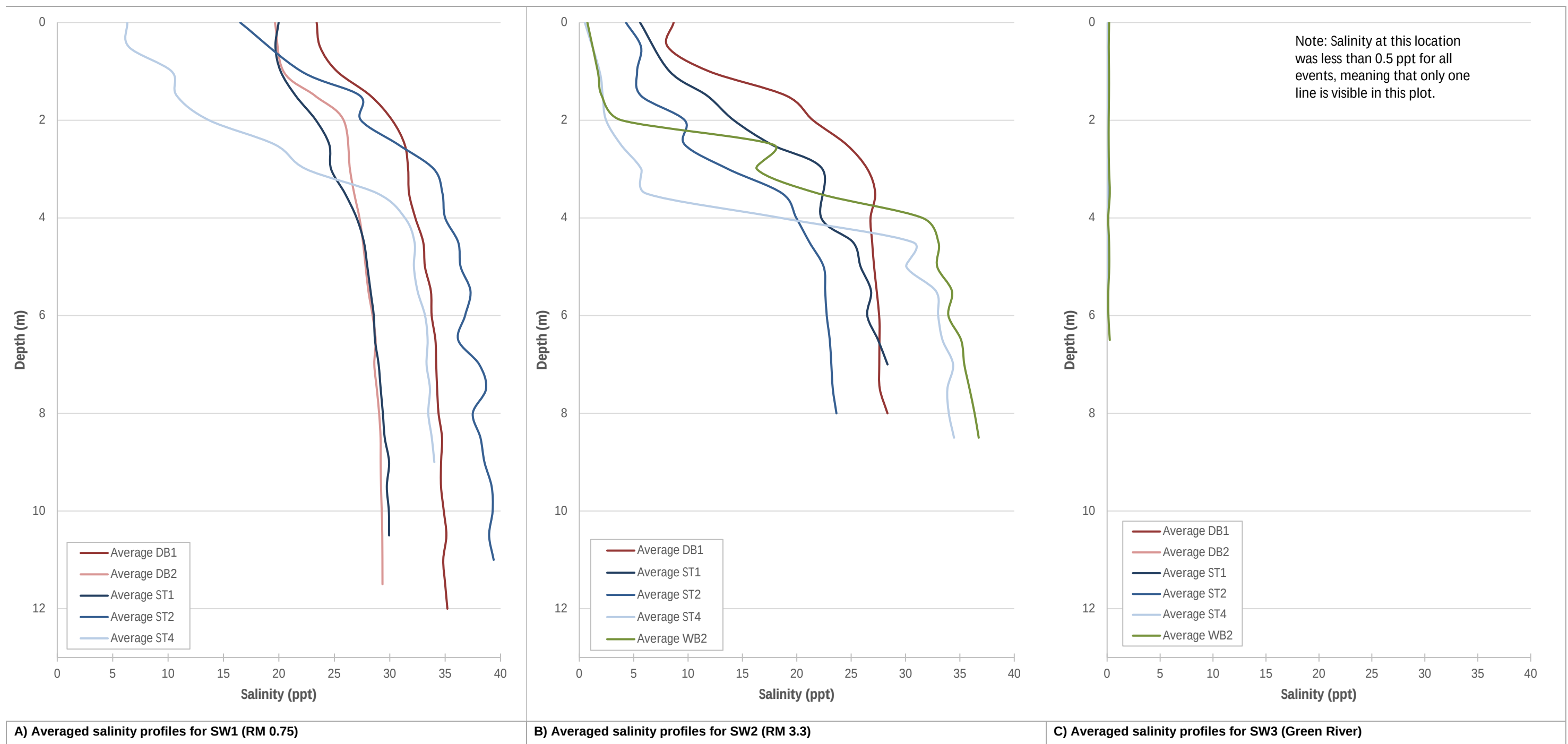
Figure C-1. Comparison of salinity profiles by location
