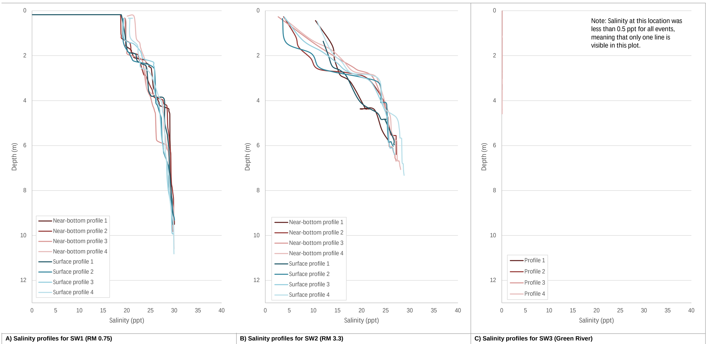
Figure C-4. Salinity profiles for storm 1 (ST1)
