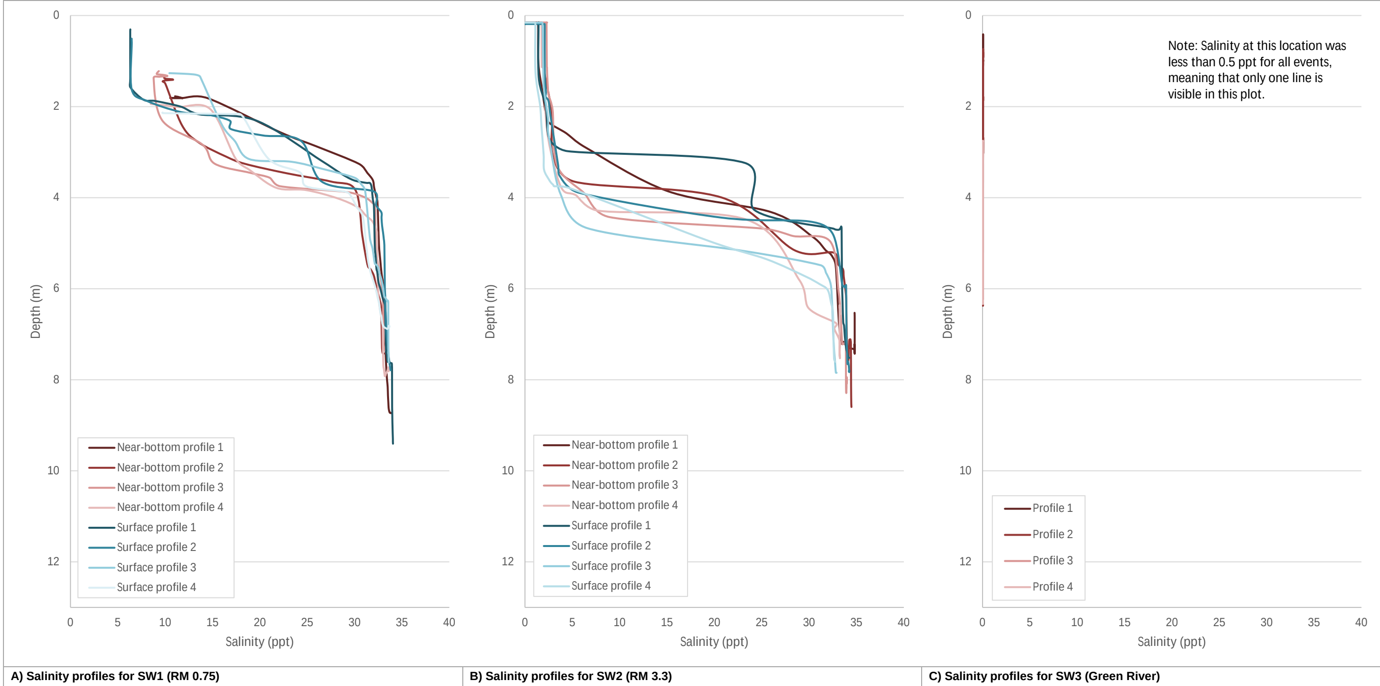
Figure C-6. Salinity profiles for storm 4 (ST4)
